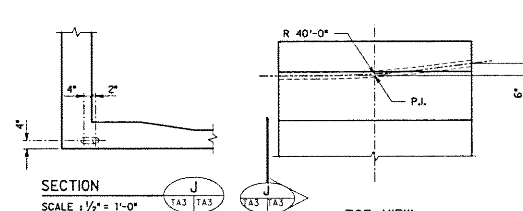
DEVIATION 7 SCALE: 1/2" = 1'-0"
