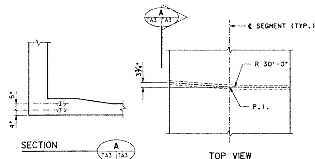
DEVIATION 1 SCALE: 1/2" = 1'-0"
