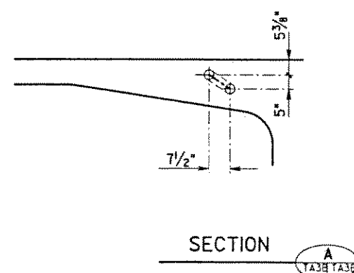
TYPICAL DEVIATION 8
