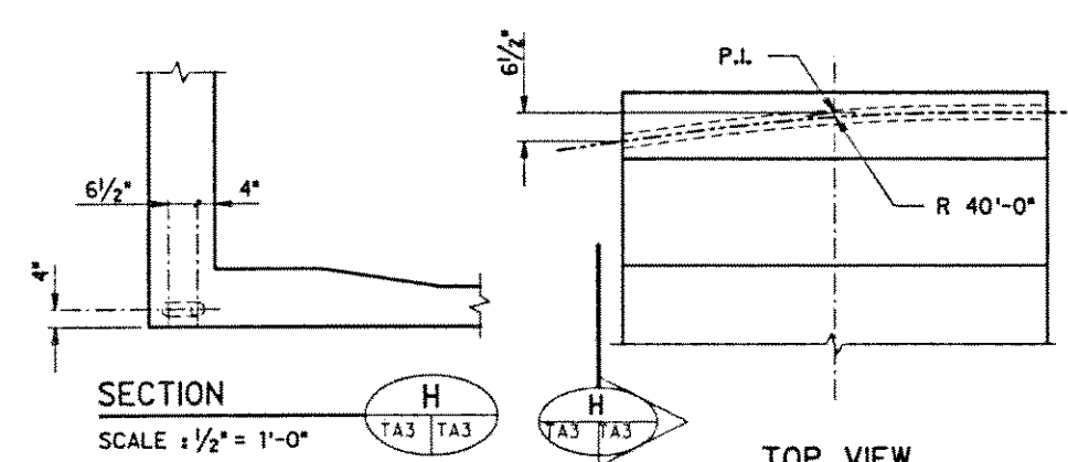
DEVIATION 6 SCALE: 1/2" = 1'-0"
