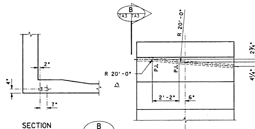
DEVIATION 2 SCALE: 1/2" = 1'-0"
