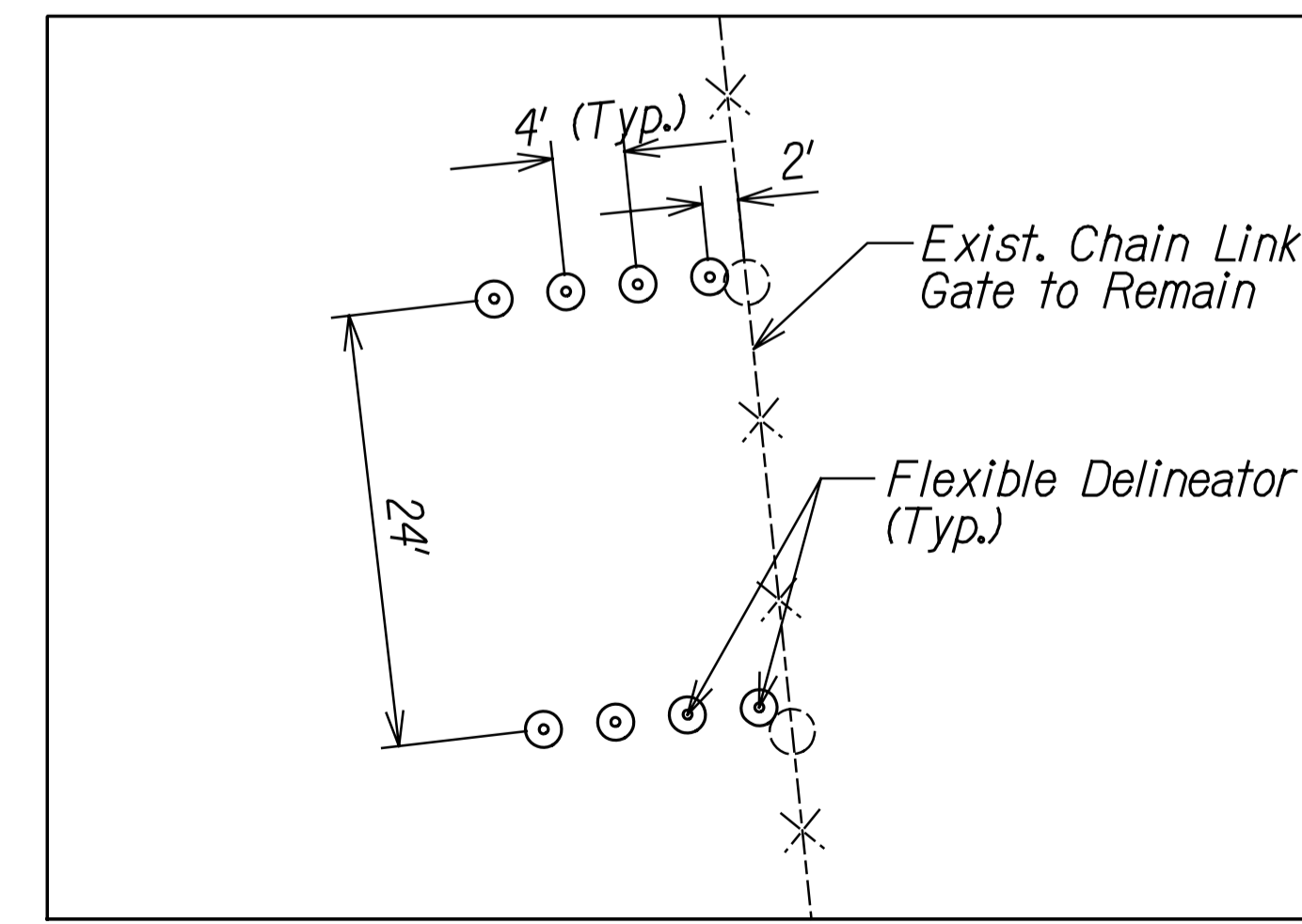
PLAN DETAIL 1 - FLEXIBLE DELINEATOR SPACING Scale: 1"=10'
