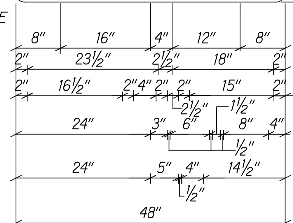
SIGN DETAIL (24"x48") NOT TO SCALE
