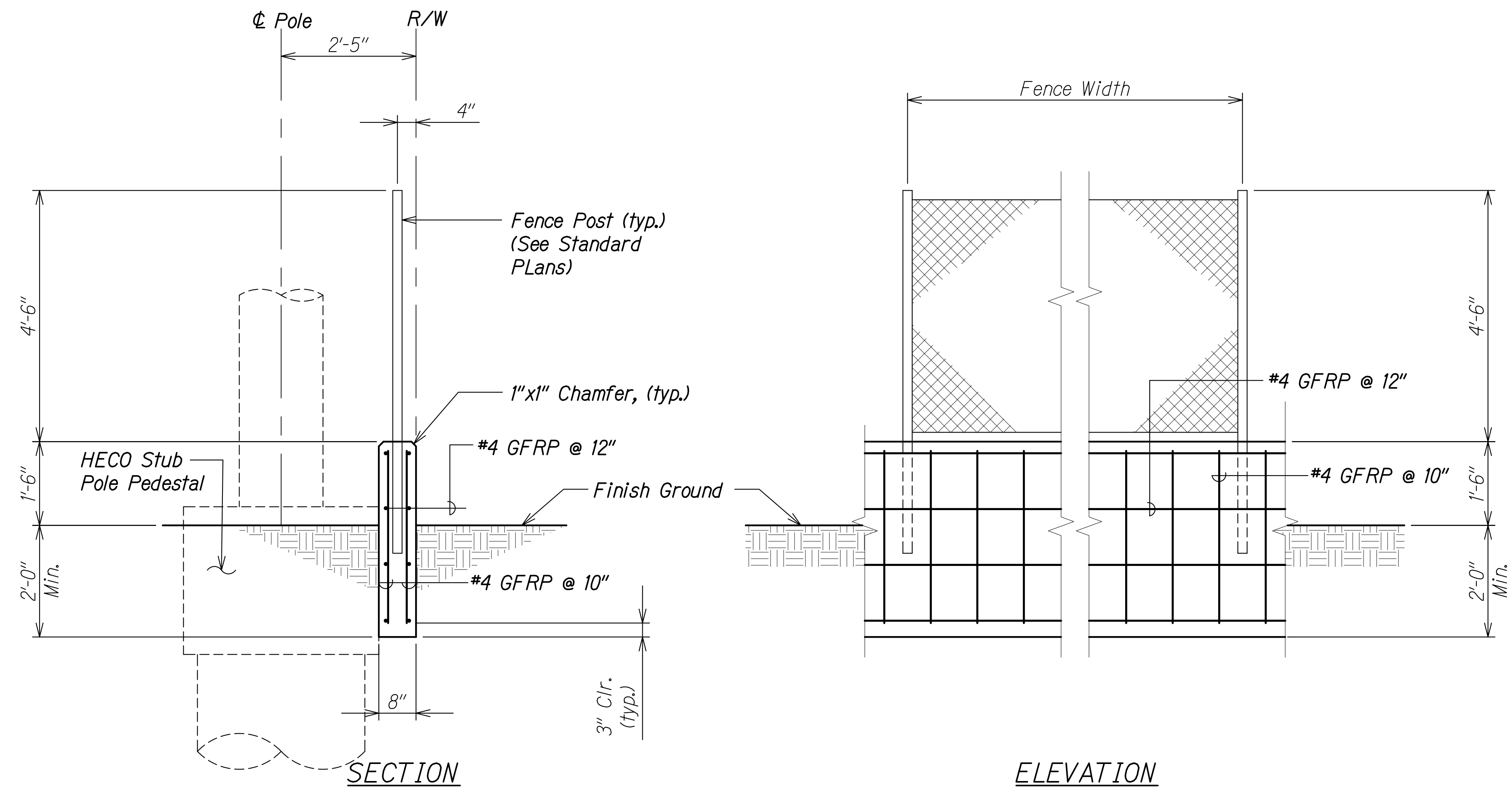
1'-6" CONCRETE CURB WITH MOUNTED 4'-6" CHAIN LINK FENCE Not to Scale
