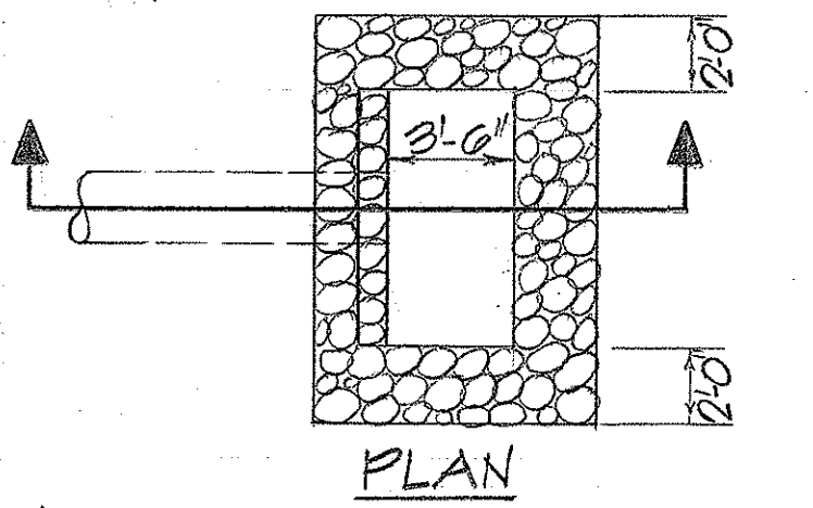
HEADWALL SEDIMENT TRAP
