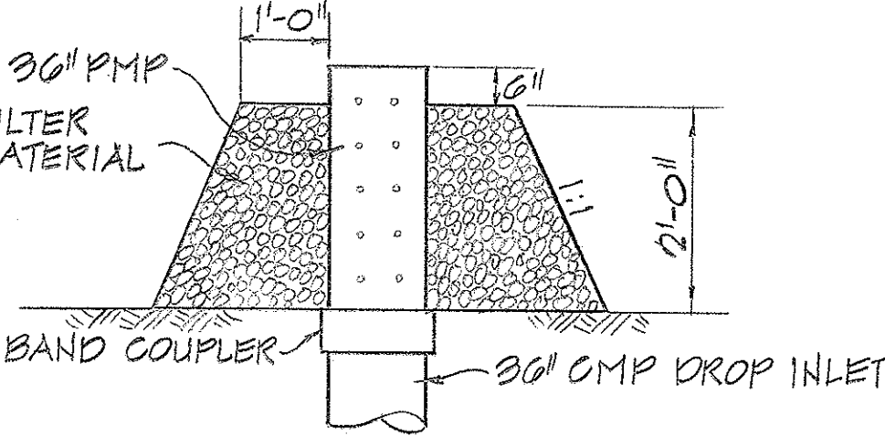
TYPE II RISER ASSEMBLY NOT TO SCALE
