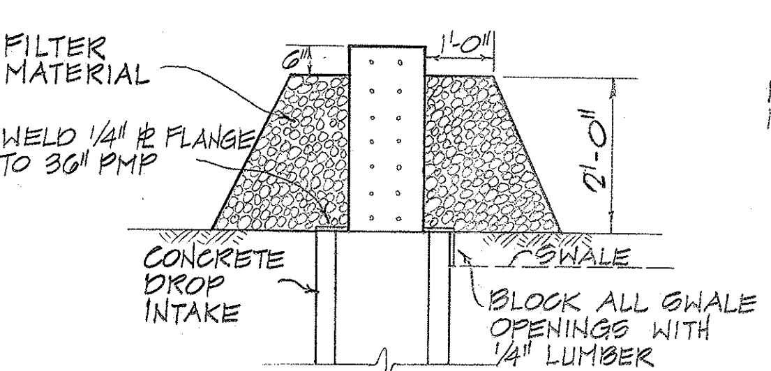
TYPE I RISER ASSEMBLY NOT TO SCALE
