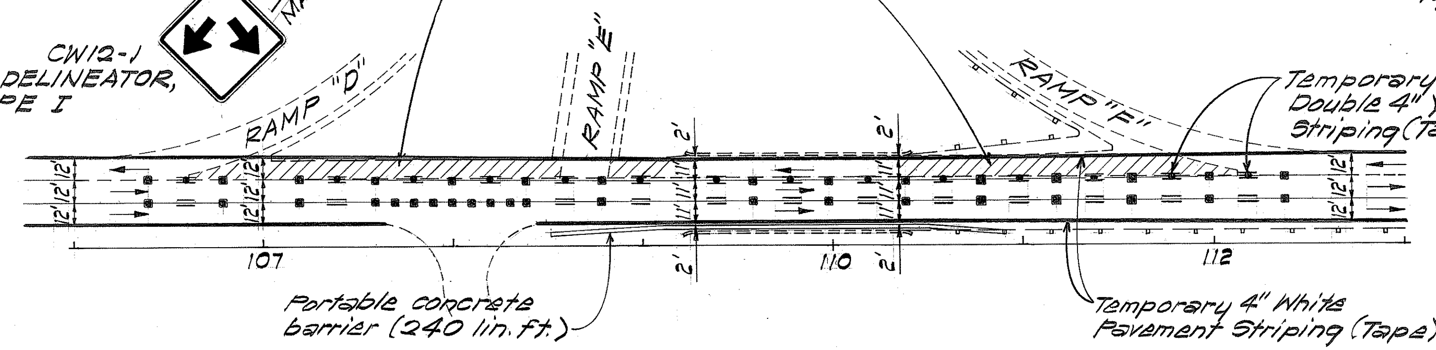
DETAIL OF DETOUR PLAN KAMOOALII STREAM BRIDGE Scale: 1"=50'
