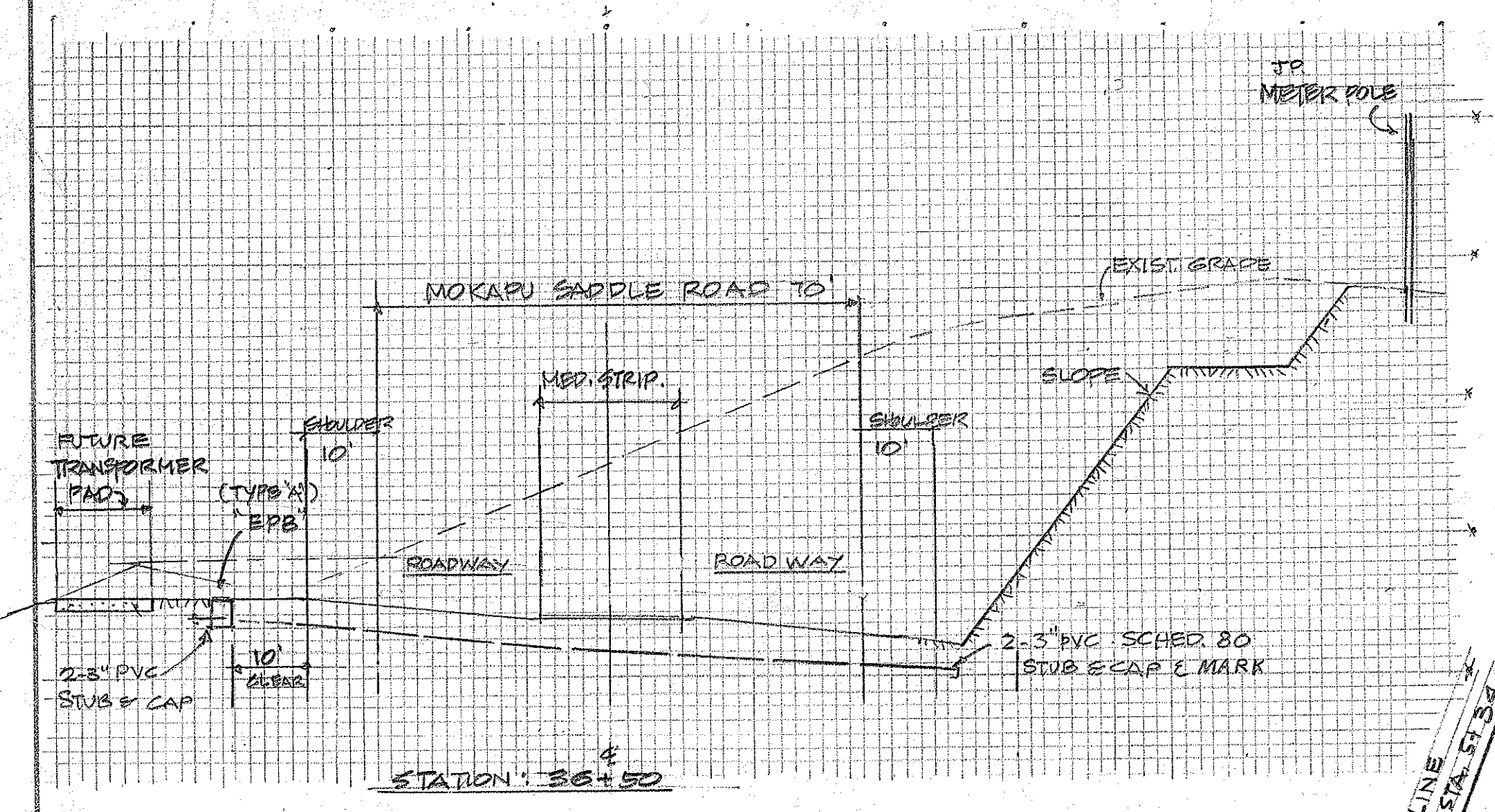
SECTION: STATION 36+50 MOKAPU SADDLE RD. SCALE: 1" = 20'
