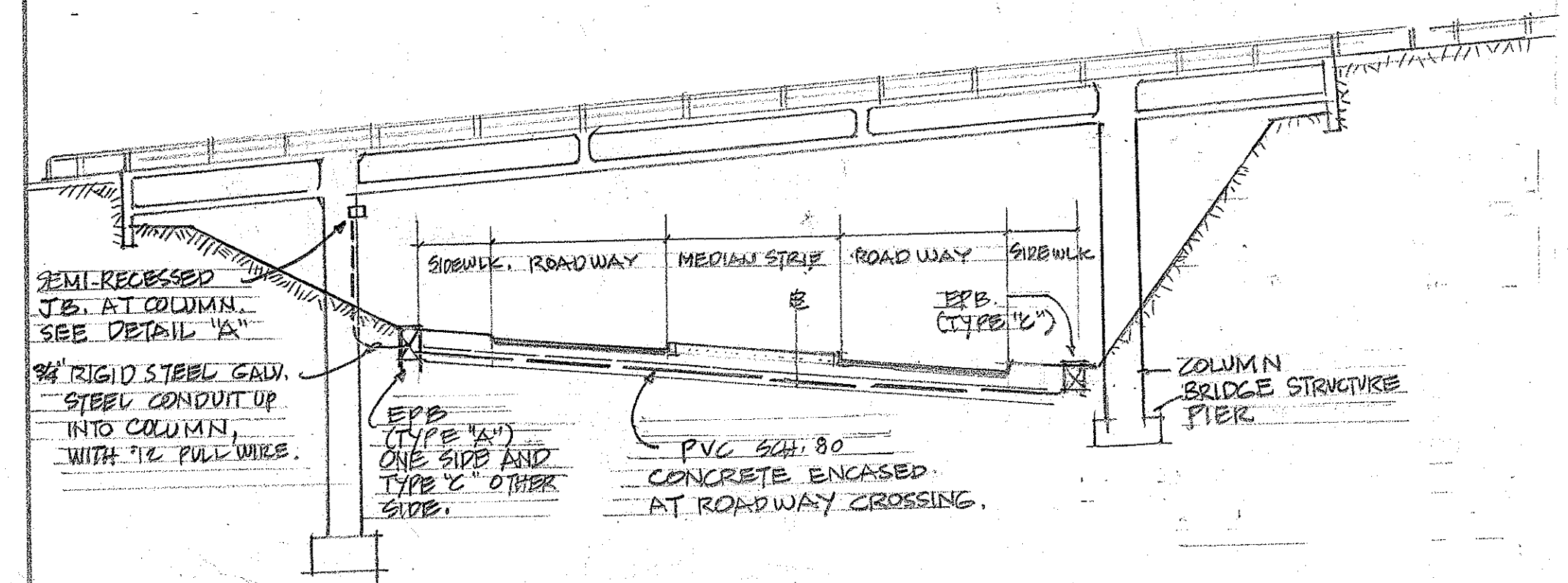
SECTION SHOWING KAILUA OVERPASS STRUCTURE & MOKAPU SADDLE ROAD SCALE: 1" = 20'
