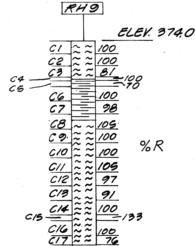
BORING RH9
