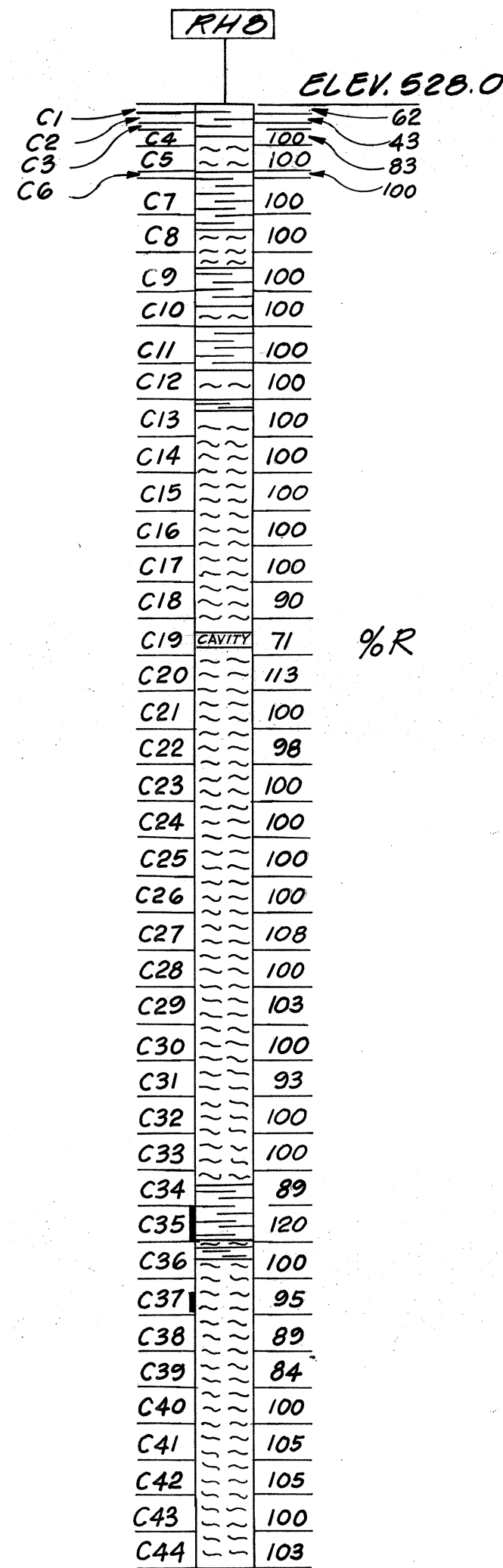
BORING RH8
