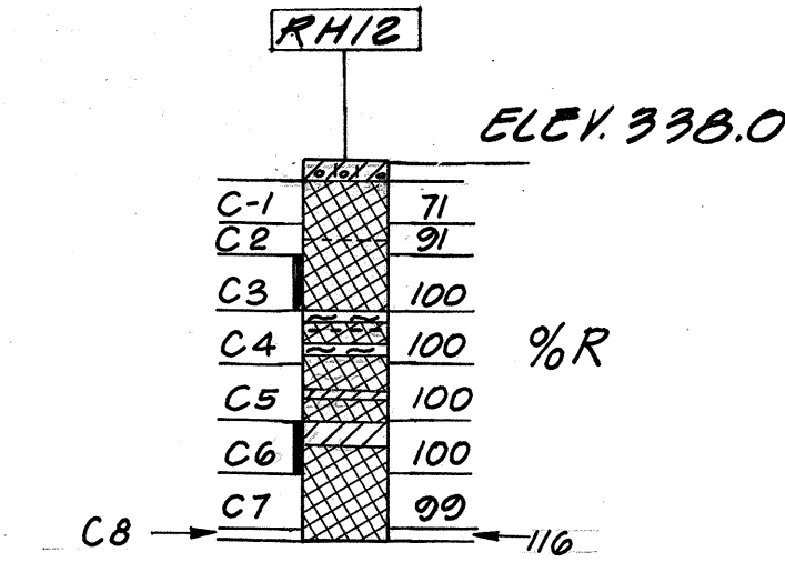
BORING RH12
