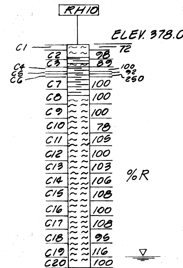
BORING RH10
