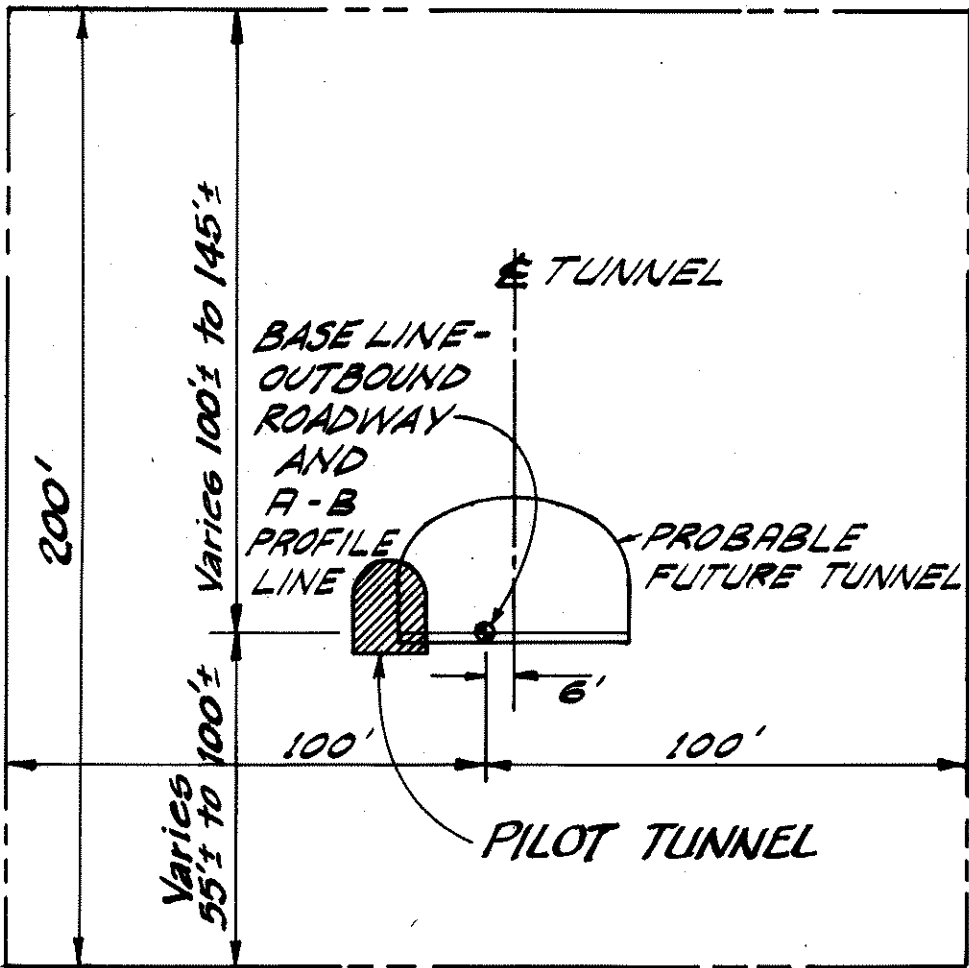
CROSS SECTION OF EASEMENTS 1 & 2 ALONG LINE A-B SCALE: 1" = 40'
