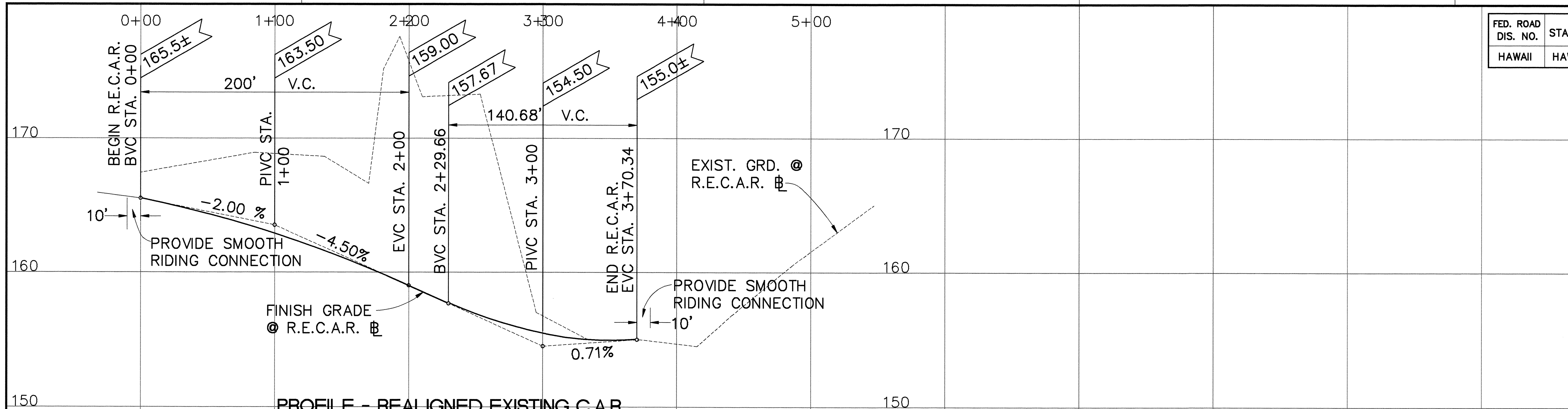
PROFILE - REALIGNED EXISTING C.A.R.
