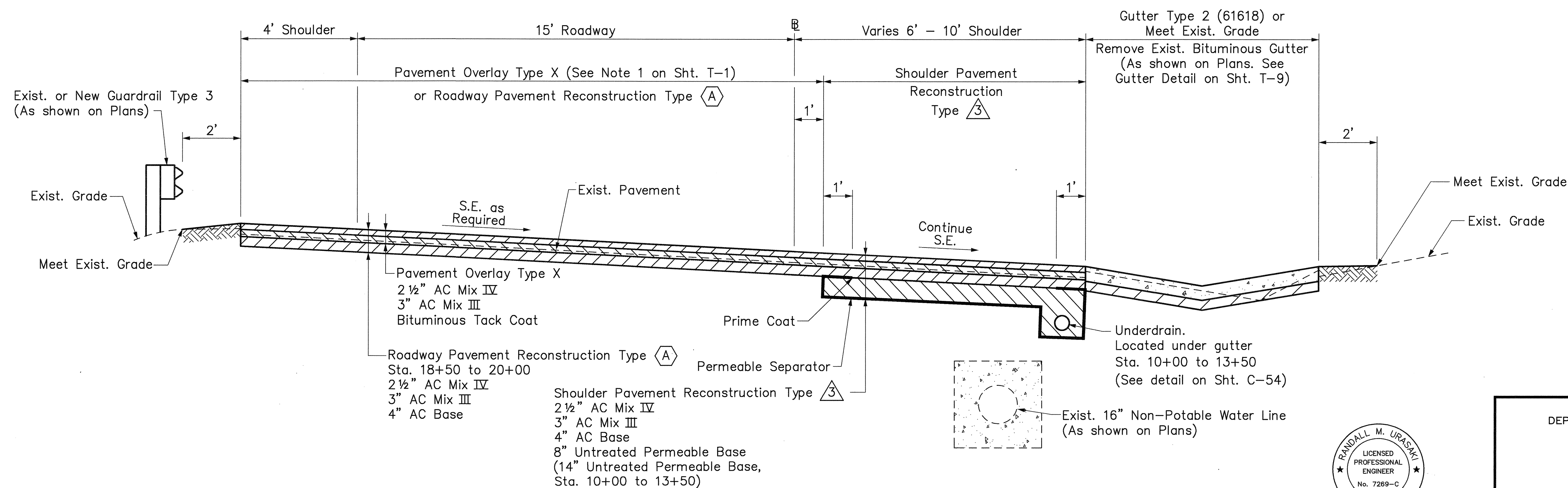
RAMP K SUPERELEVATED SECTION
