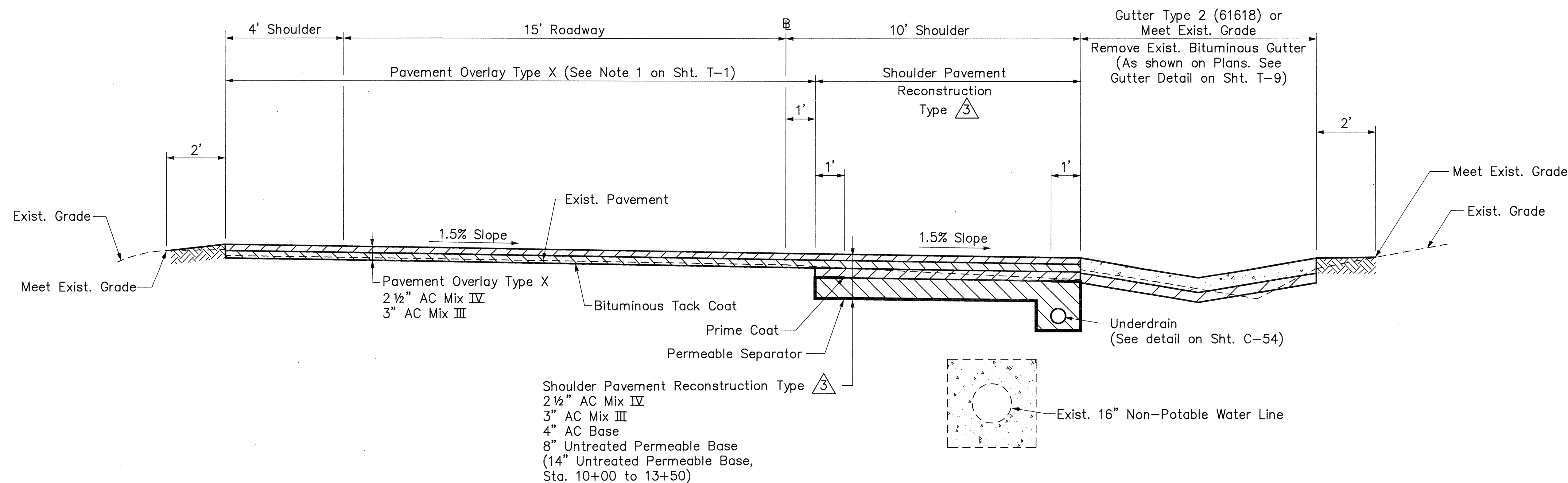
RAMP K NORMAL SECTION
