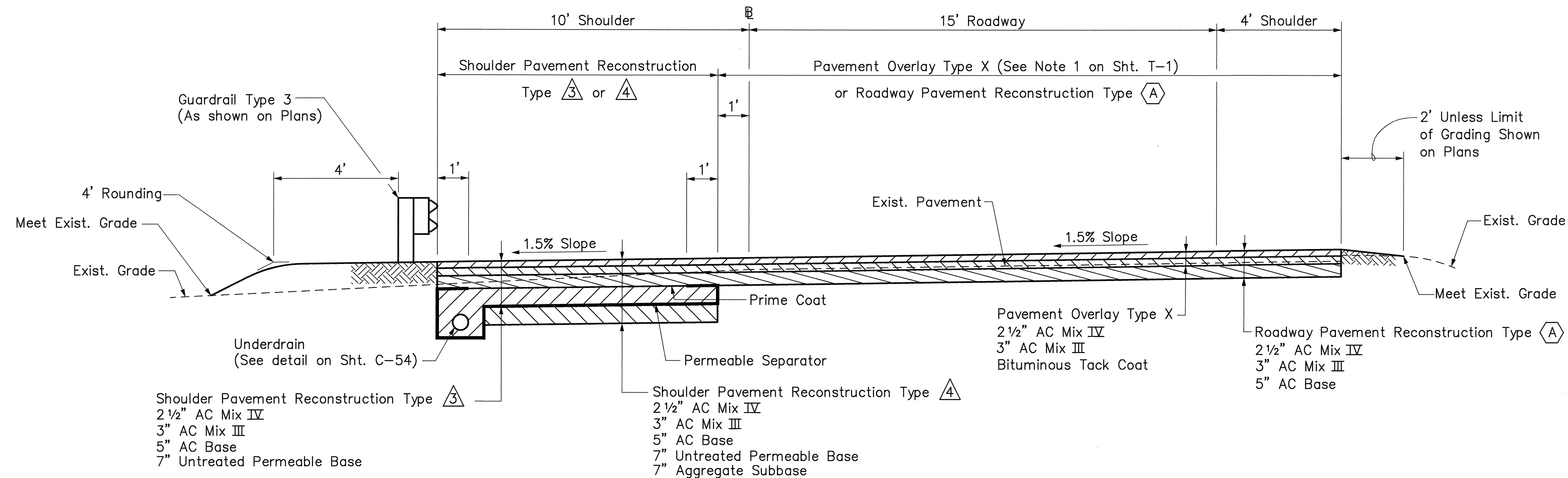
RAMP EW NORMAL SECTION
