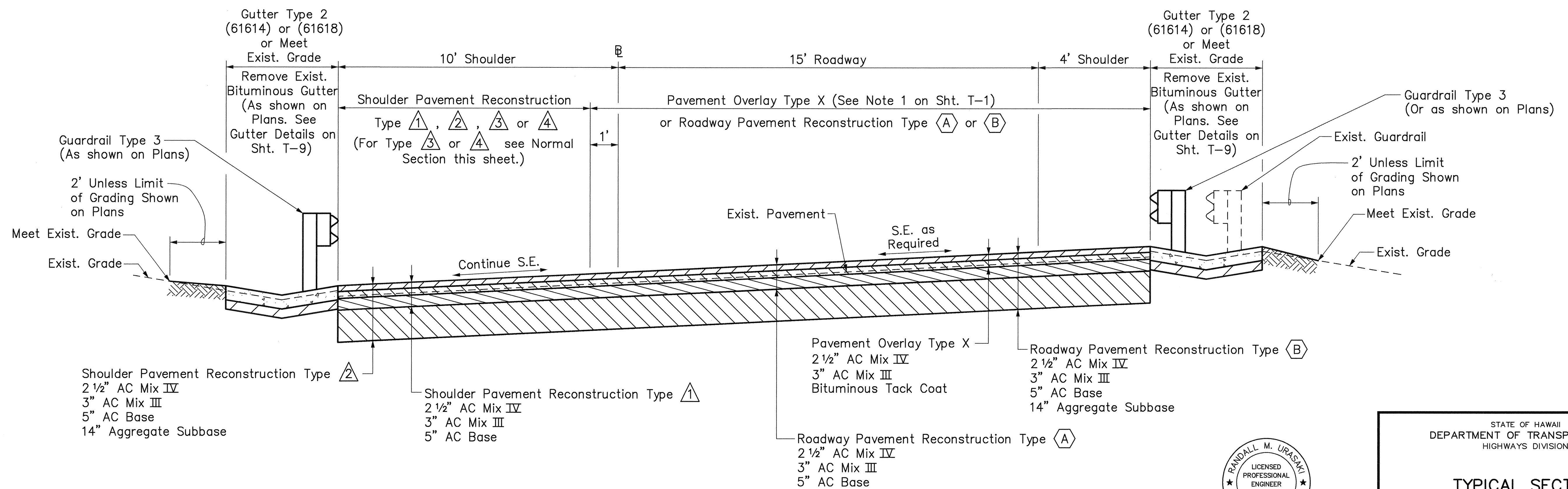
RAMP EW SUPERELEVATED SECTION
