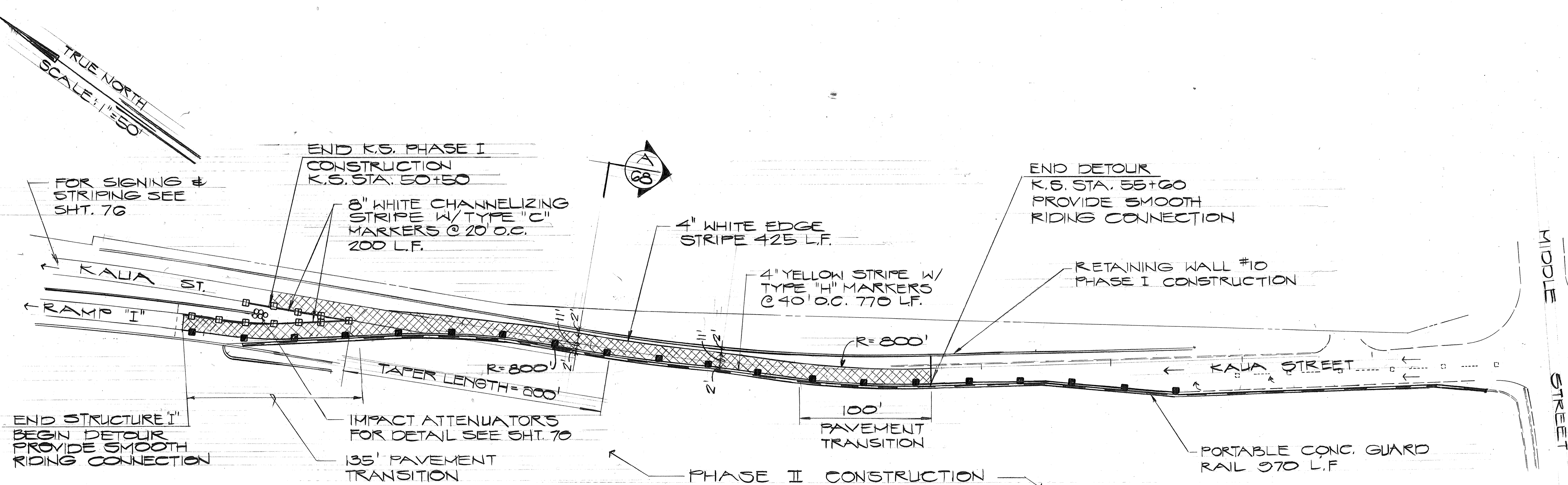
RAMP "I" PHASE II DETOUR SCALE: 1"=50'
