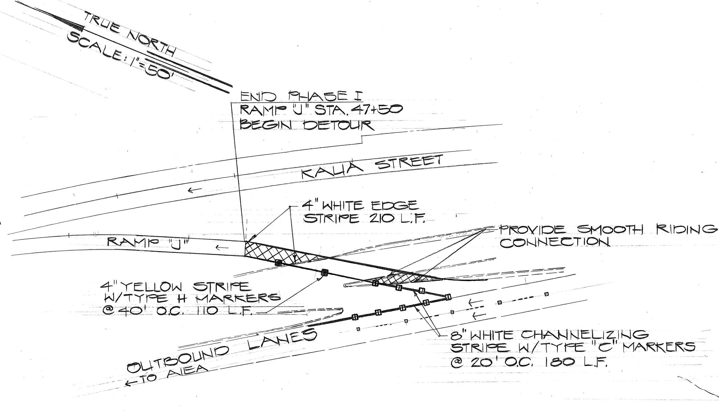
RAMP "J" PHASE II DETOUR SCALE: 1"=50'
