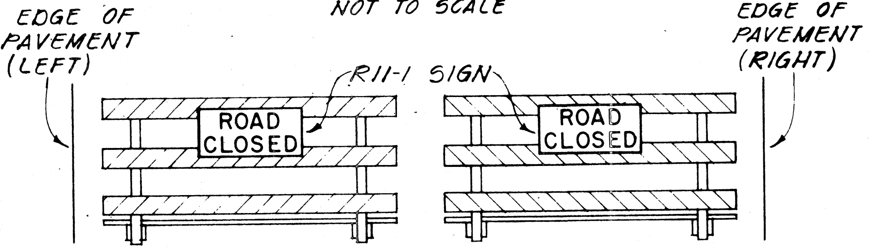
FRONT VIEW
