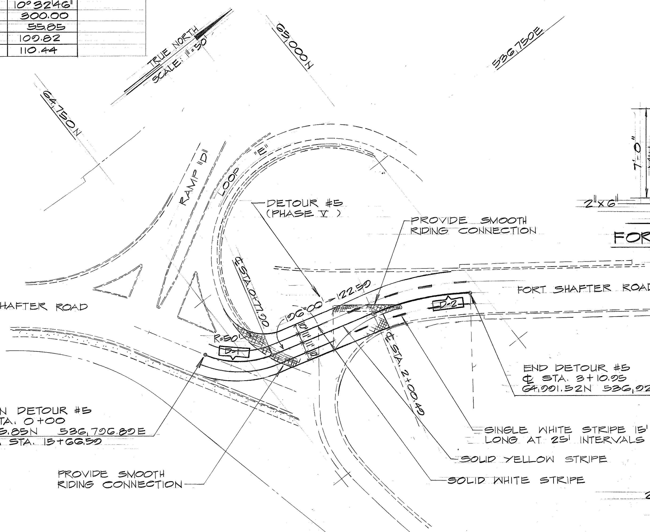
PLAN
