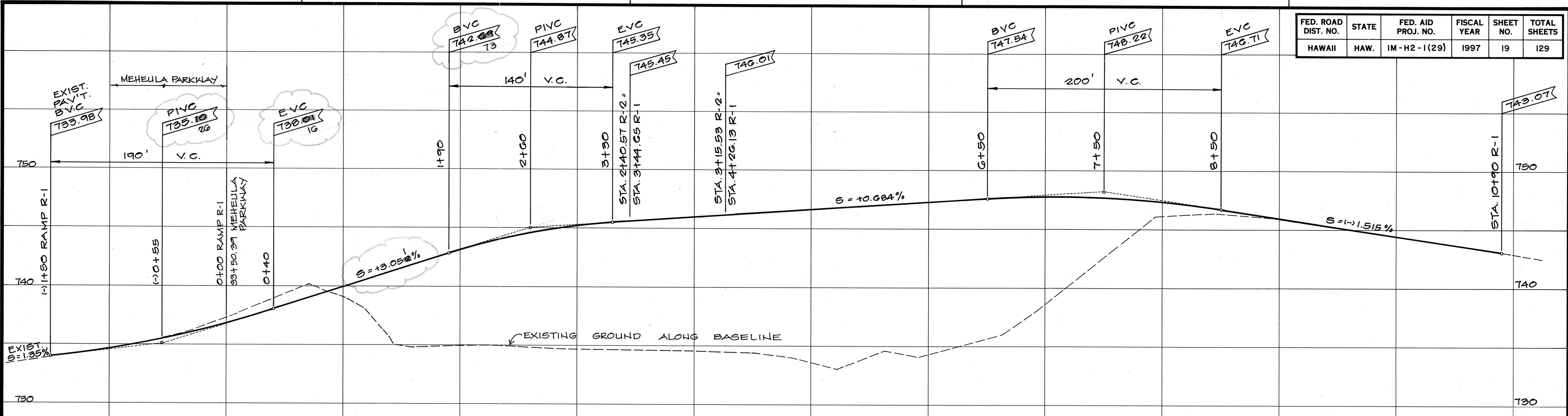
PROFILE - RAMP R-1 SCALE: HORIZ. 1" = 40' VERT. 1" = 4'
