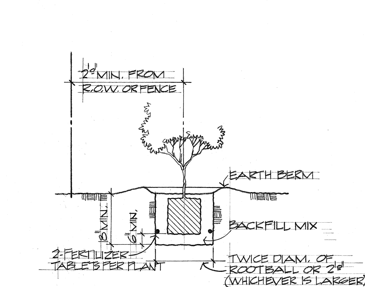
TYP. SHRUB PLANTING DETAIL NO SCALE
