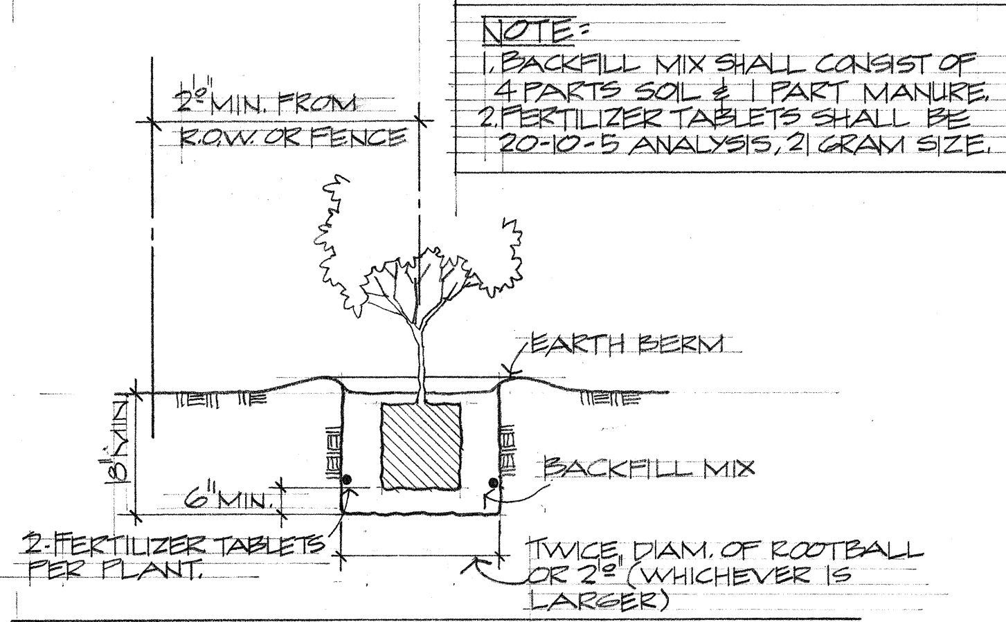
TYPICAL SHRUB PLANTING DETAIL NO SCALE
