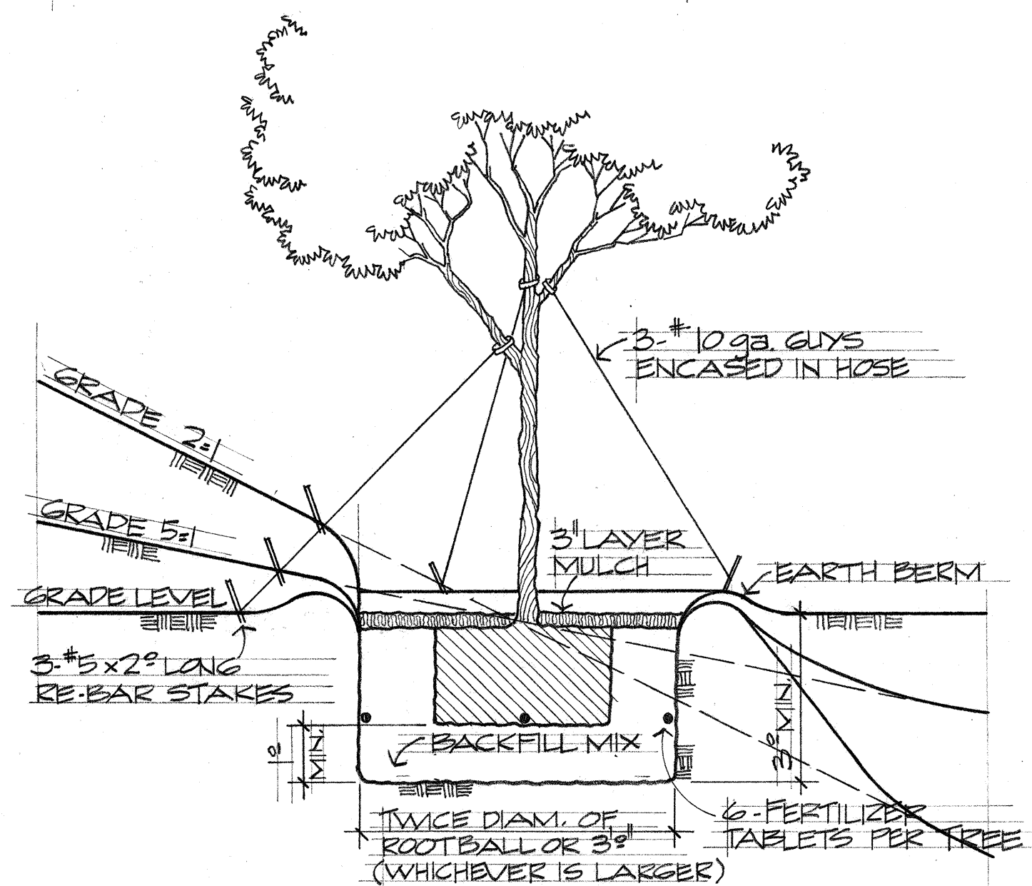
TYP. 25 GAL. TREE PLANTING DETAIL NO SCALE
