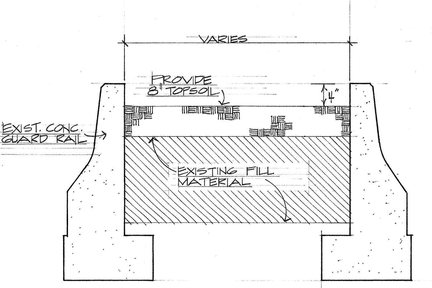
(A) CONCRETE PLANTER BOX SECTION SCALE: 3/4" = 1'-0"
