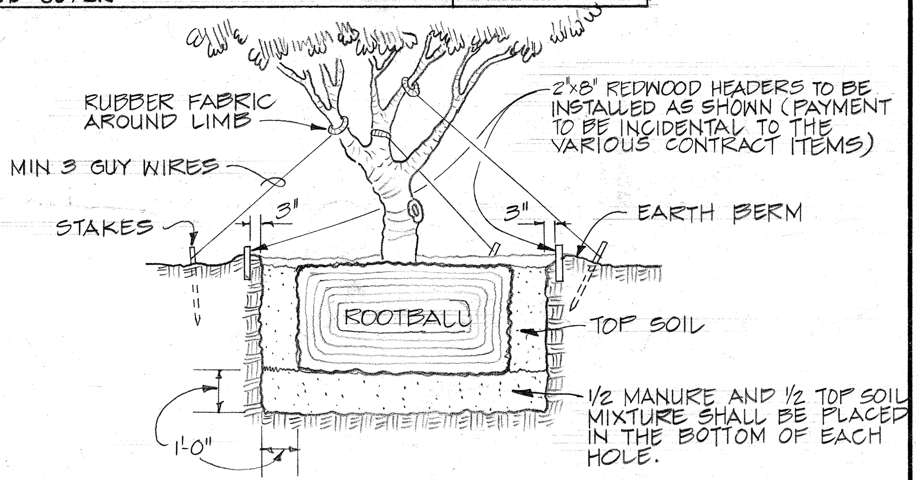
DETAIL FOR TRANSPLANTED TREE NO SCALE
