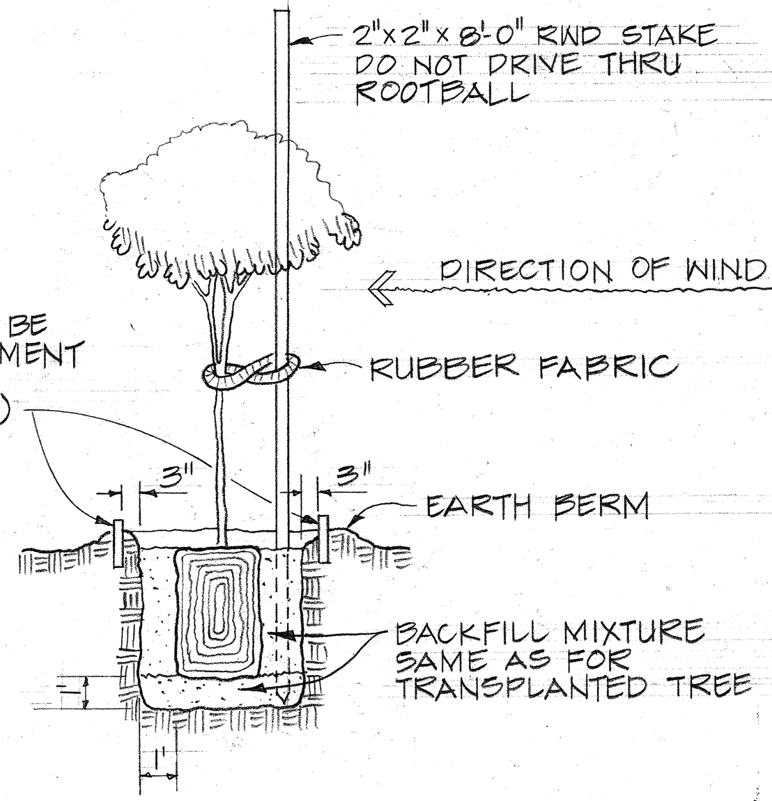
DETAIL FOR CONTAINER TREES NO SCALE
