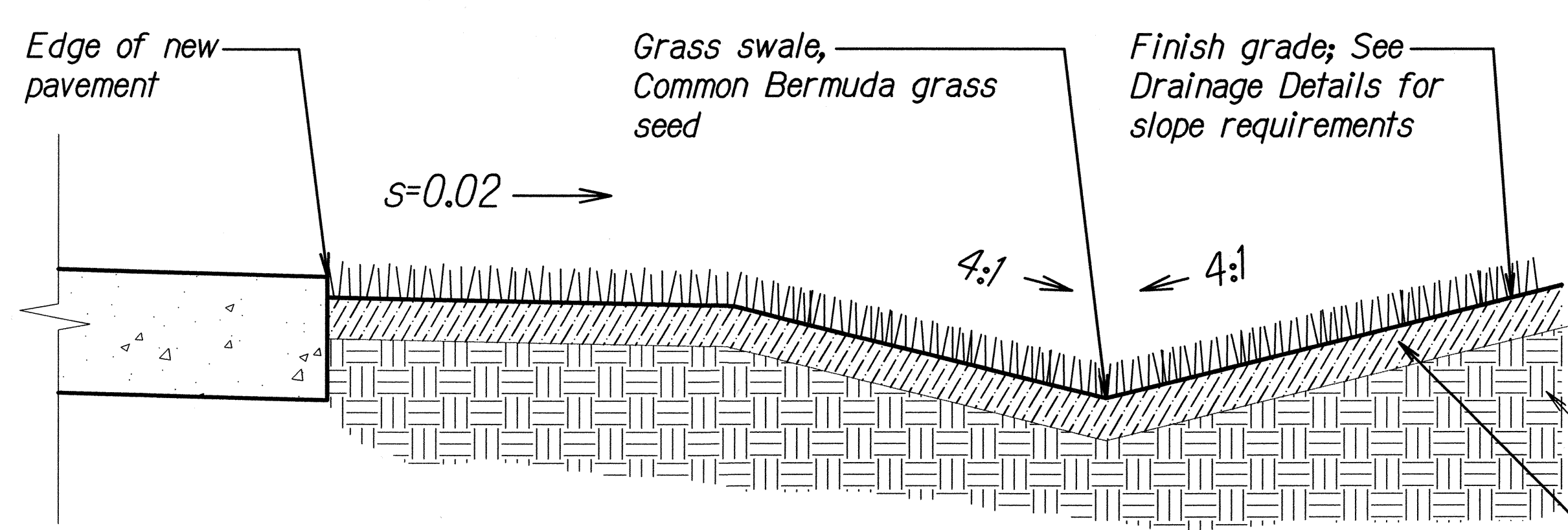
2 SECTION THRU GRASS SWALE Scale: 1" = 1'-0"
