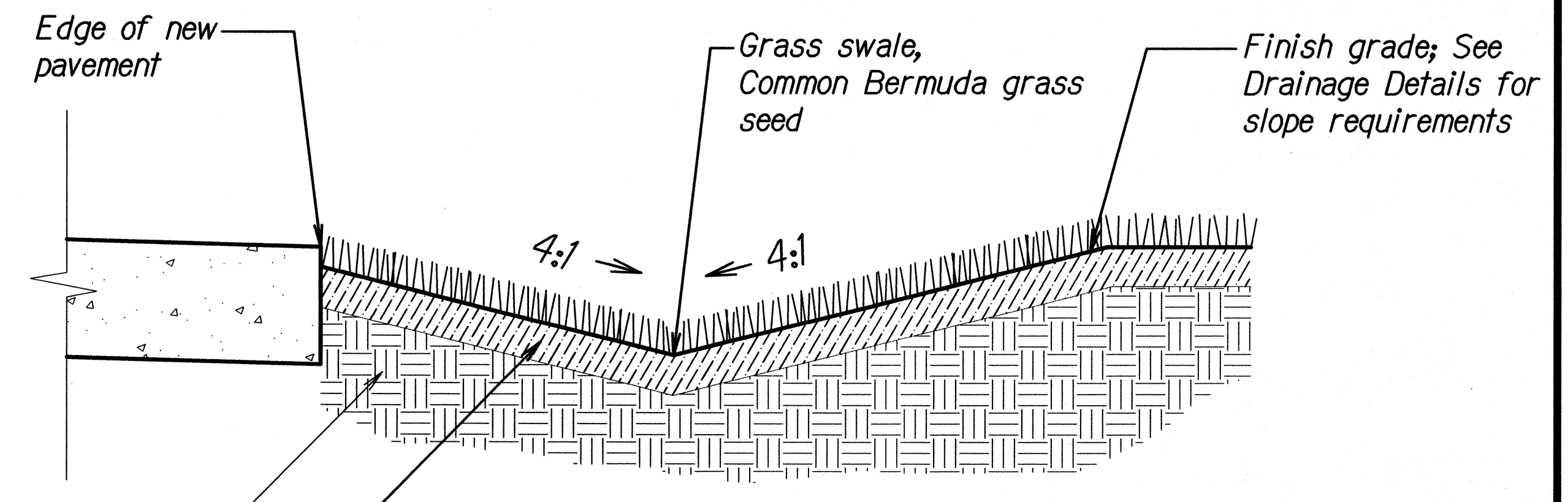
1 SECTION THRU GRASS SWALE Scale: 1" = 1'-0"
