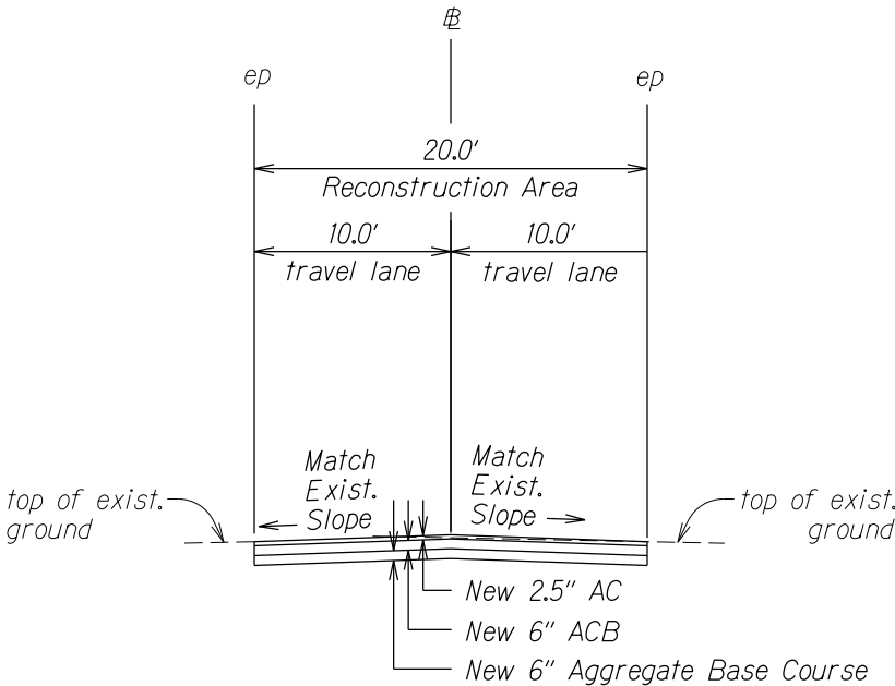
SECOND ST. # STA. 2+95 TO # STA. 4+10 Not to Scale
