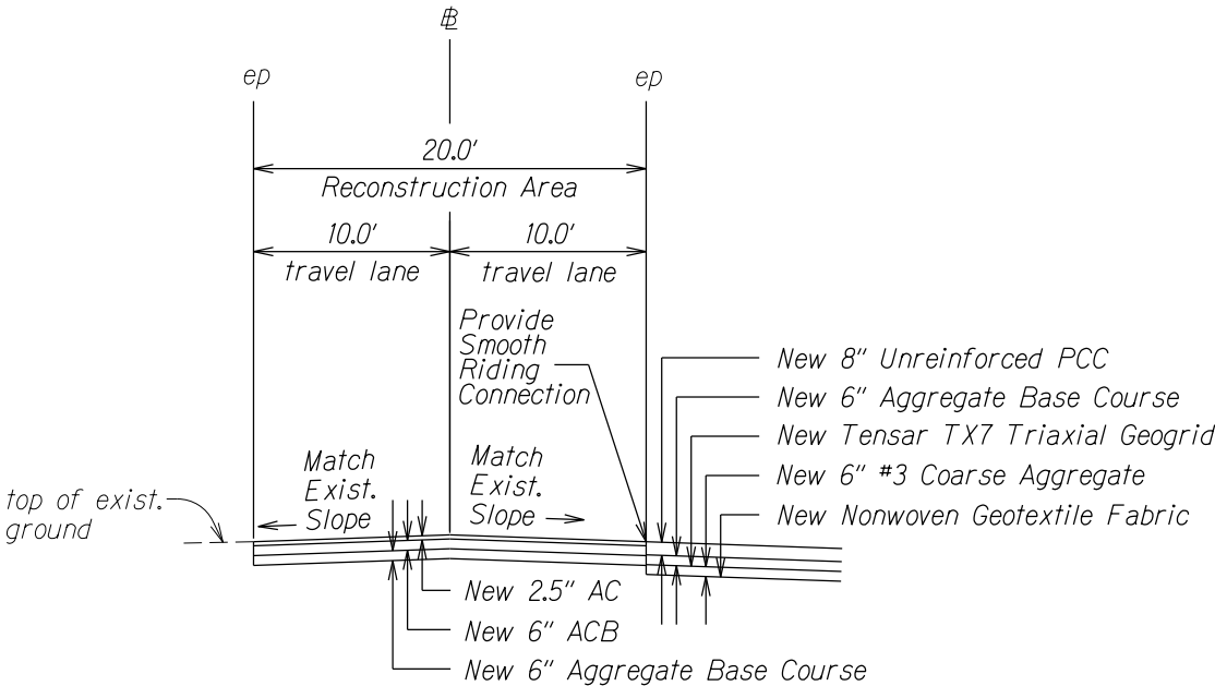
SECOND ST. # STA. 2+50 TO # STA. 2+95 Not to Scale
