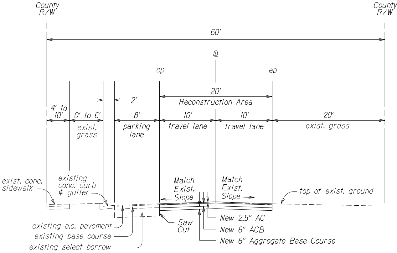
SECOND ST. # STA. 4+10 TO # STA. 5+40 Not to Scale
