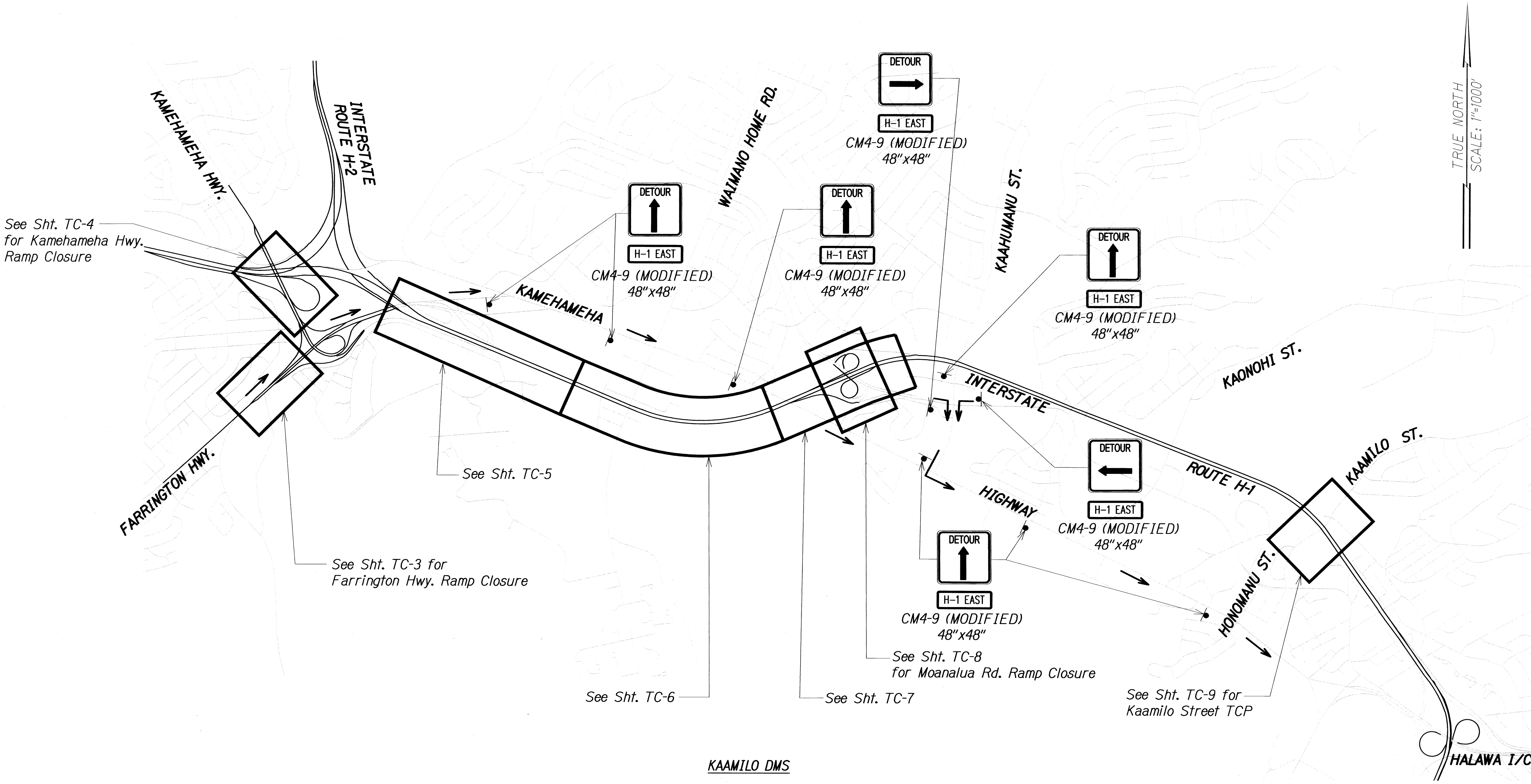
FREEWAY CLOSURE AND DETOUR ROUTE PLANS Scale: 1"=1000'
