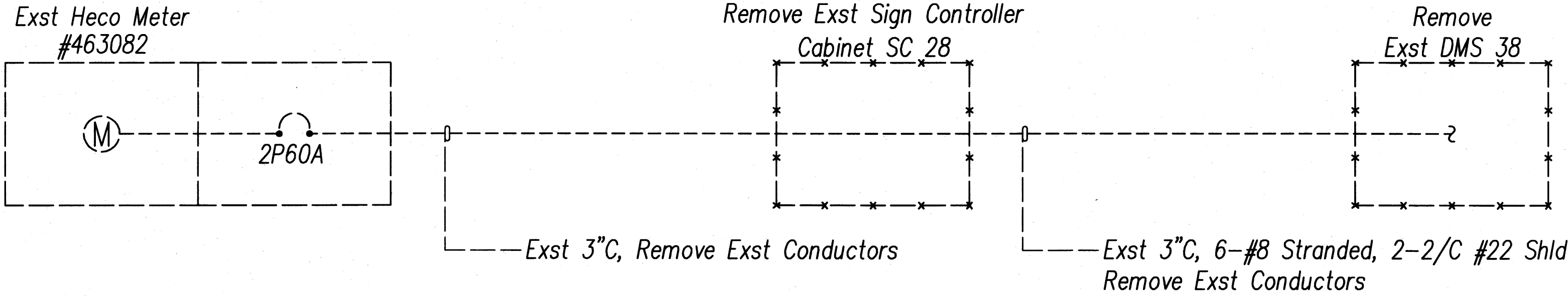
KAAMILO DMS DEMOLITION ONELINE DIAGRAM
