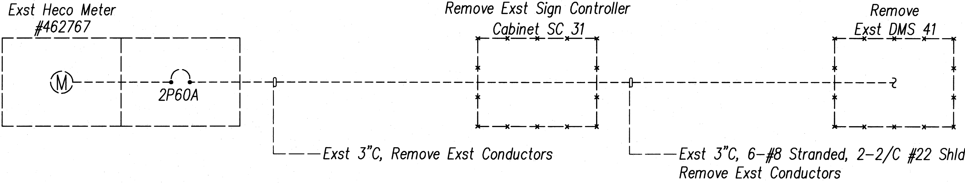
LILIHA DMS DEMOLITION ONELINE DIAGRAM
