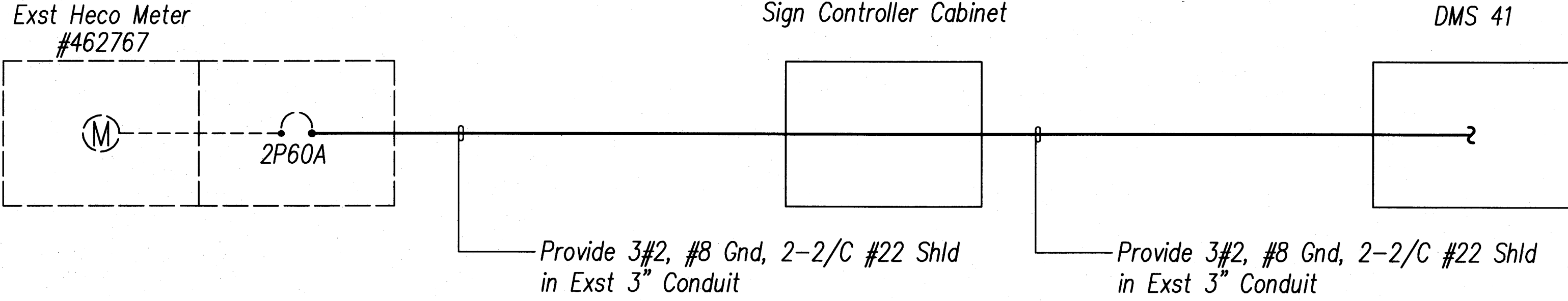
LILIHA DMS ONELINE DIAGRAM
