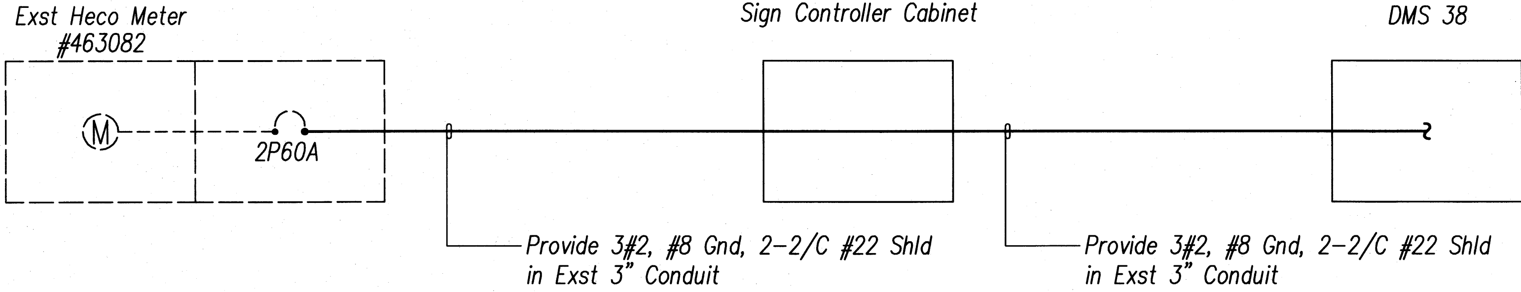
KAAMILO DMS ONELINE DIAGRAM
