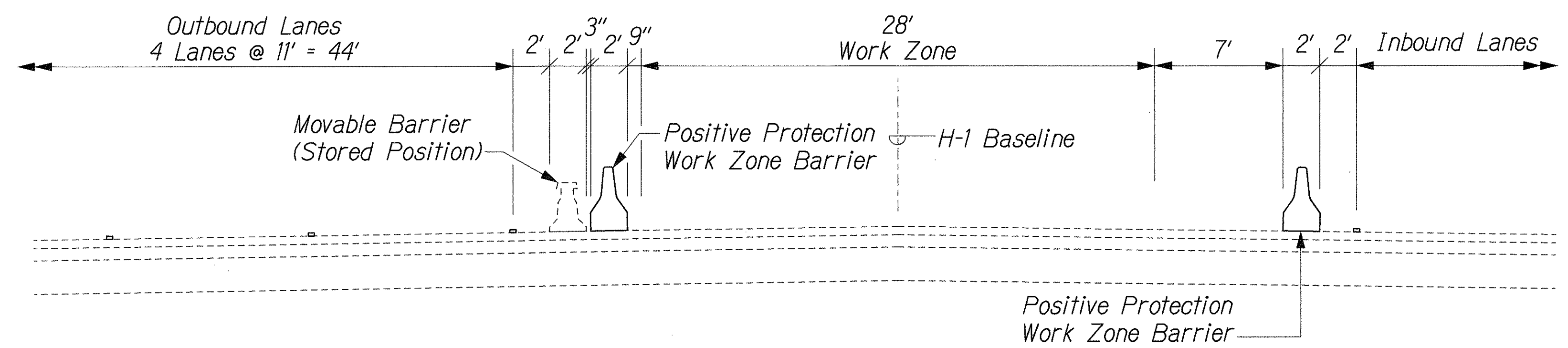
TYPICAL SECTION (STA. 67+50 to 73+10) Not to Scale
