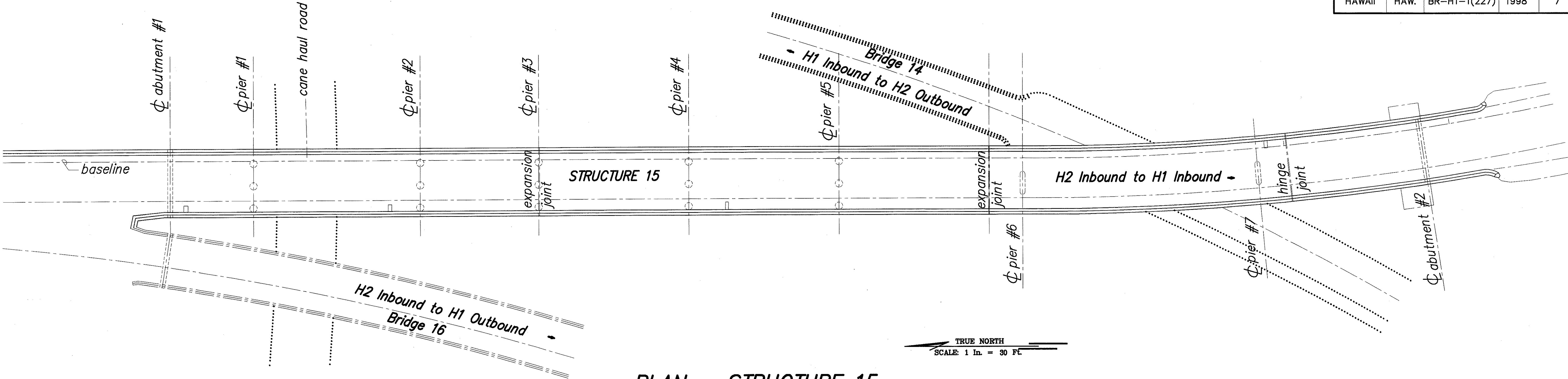
PLAN – STRUCTURE 15 SCALE: 1" = 30' 749.00'
