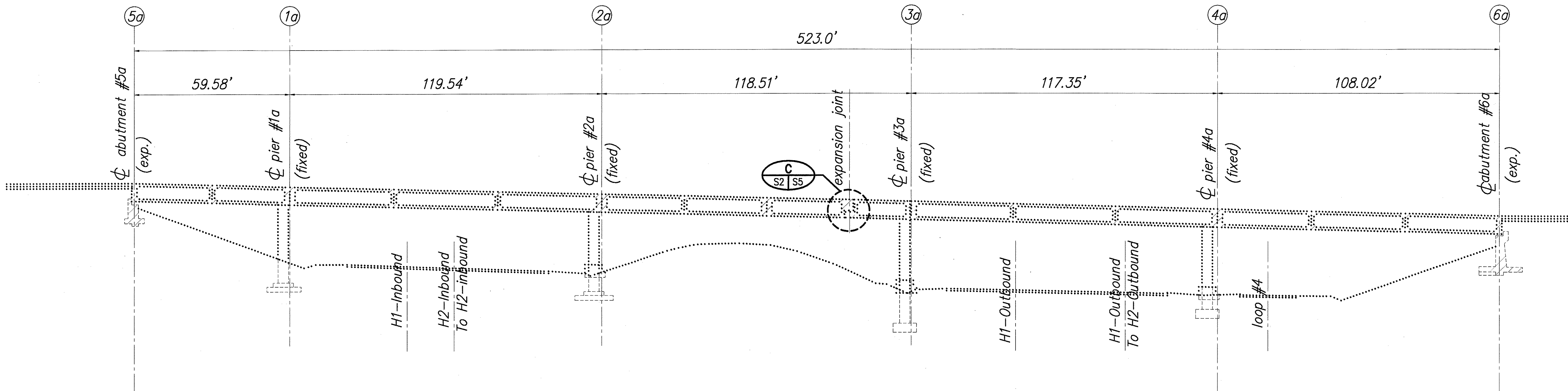
LONGITUDINAL SECTION – BRIDGE 3A (FARRINGTON HIGHWAY OUTBOUND) SCALE: 1" = 20'
