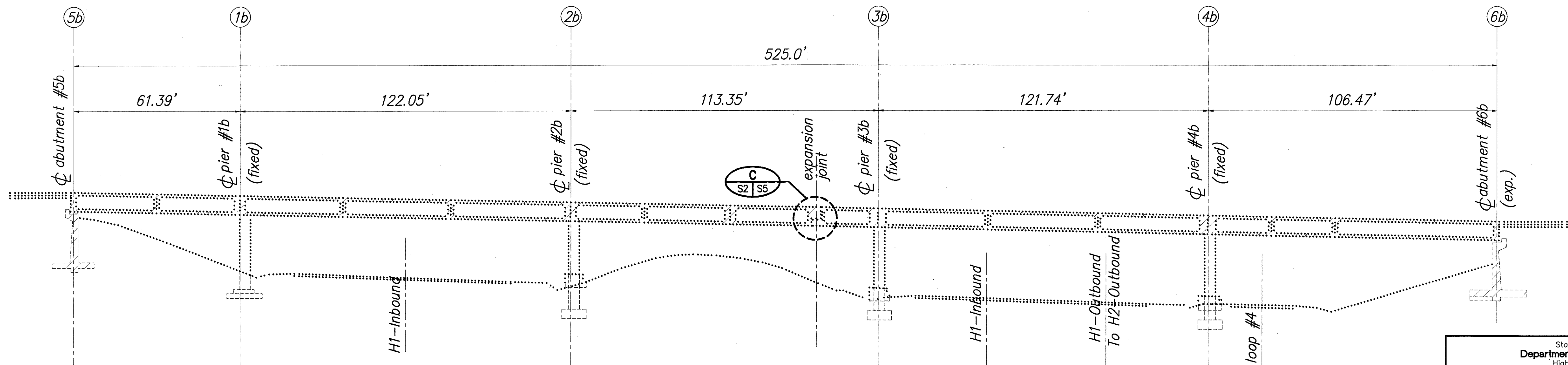
LONGITUDINAL SECTION – BRIDGE 3B (FARRINGTON HIGHWAY INBOUND) SCALE: 1" = 20'
