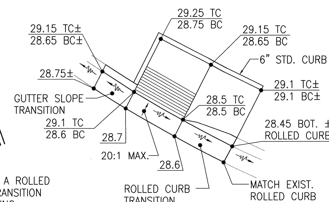
DETAIL RAC SCALE: 1"=5' CURB RAMP-TYPE "B" MODIFIED
