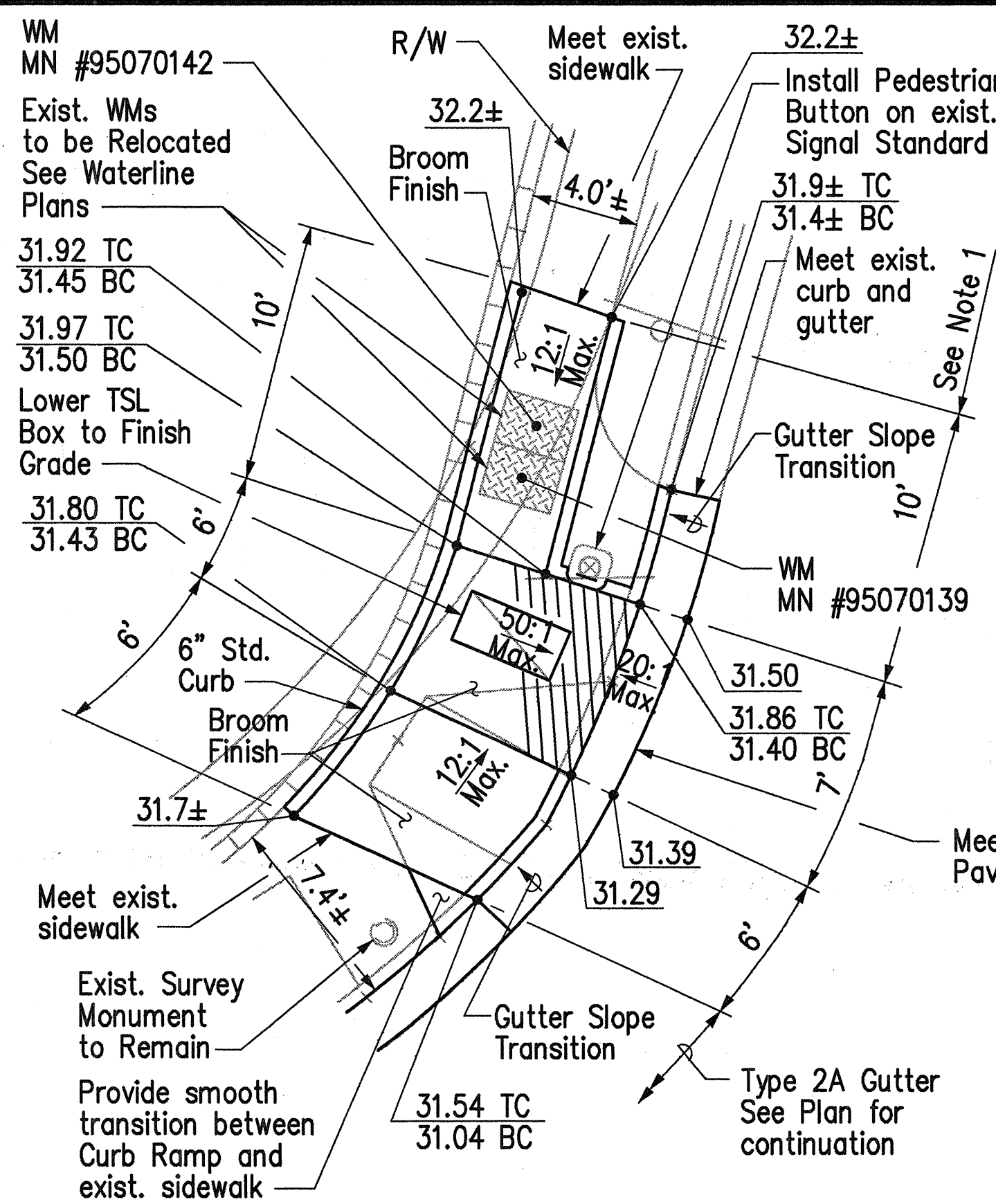
DETAIL A
