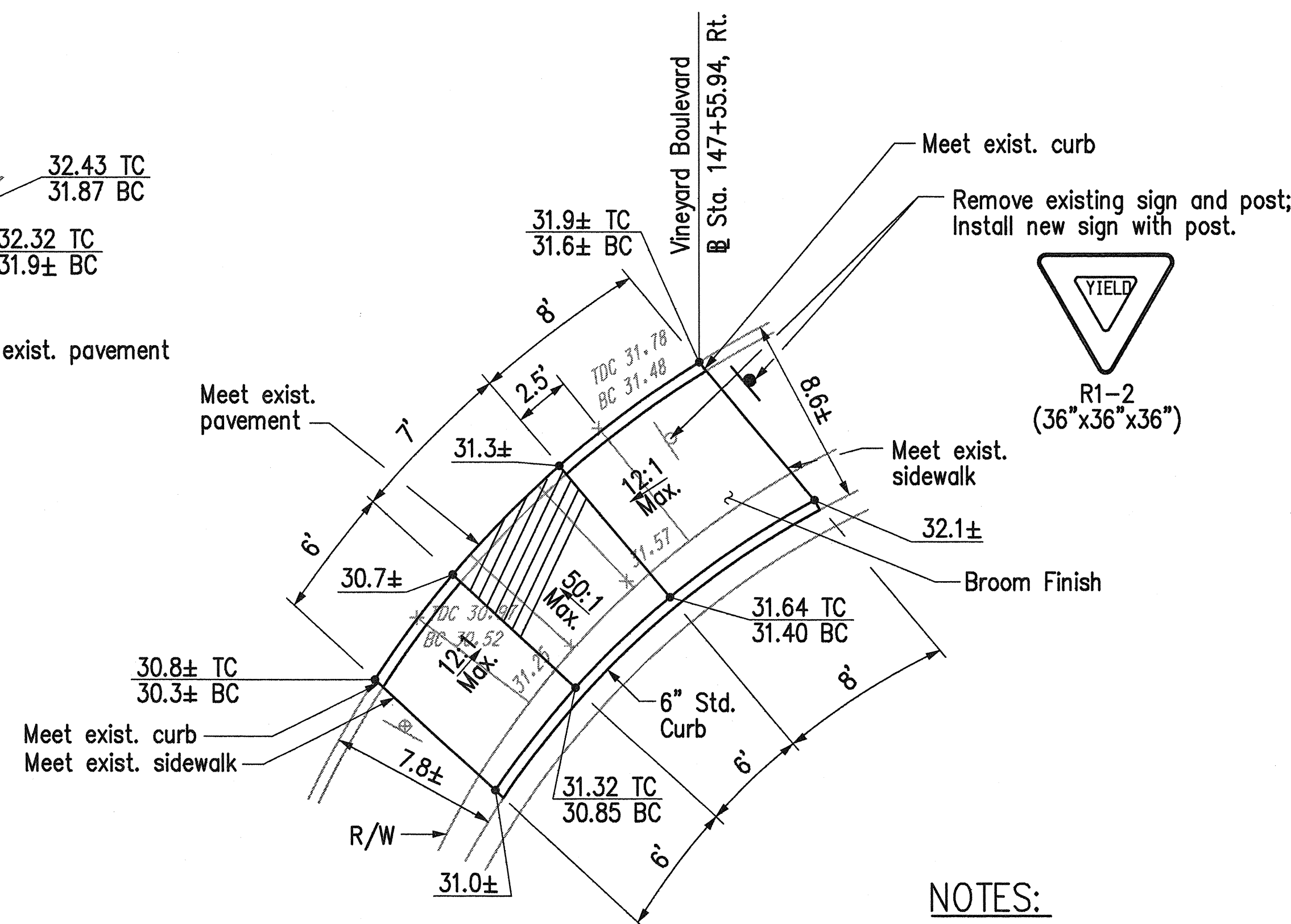
DETAIL L
