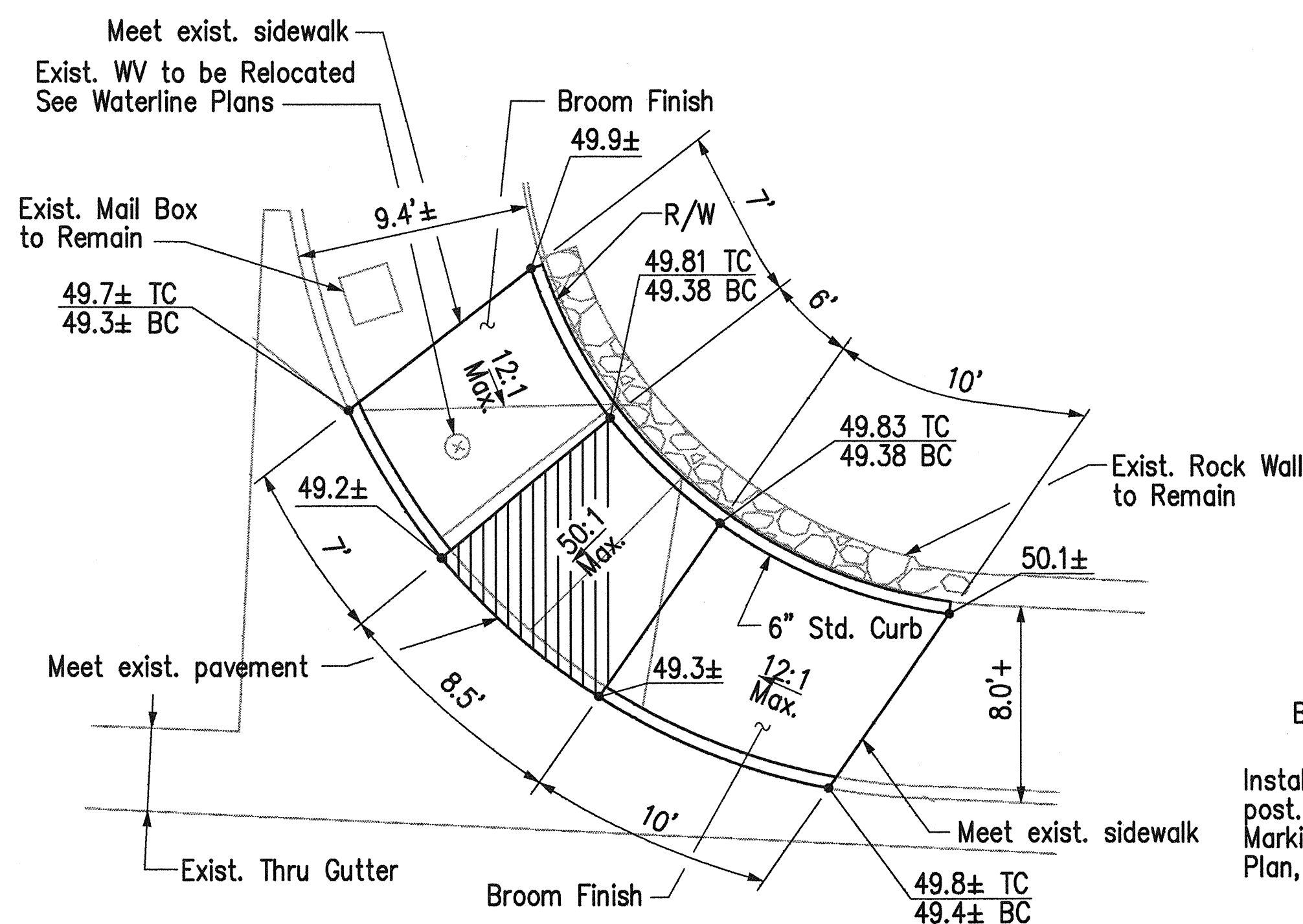
DETAIL A Curb Ramp - Type "B"
