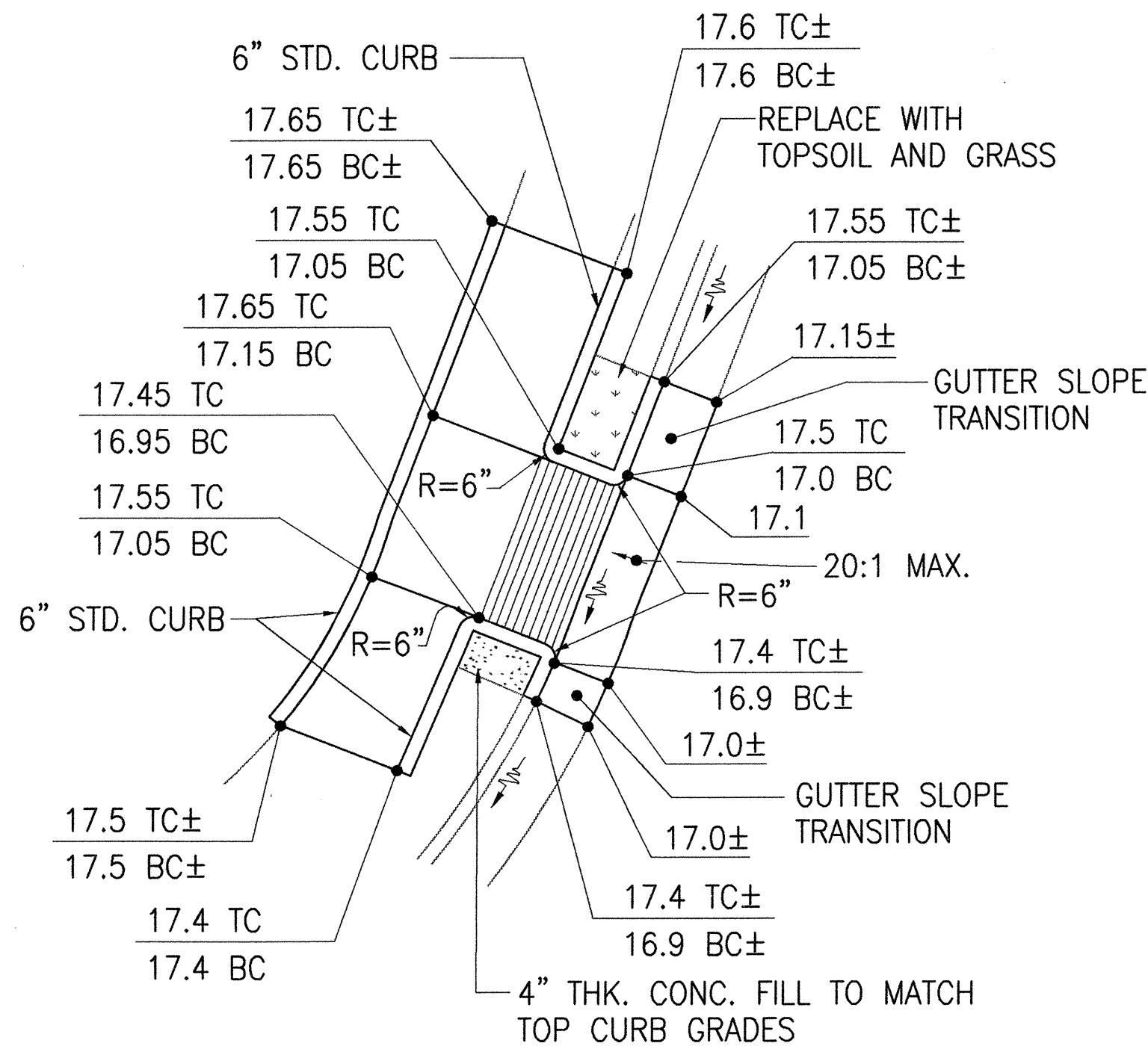
DETAIL RO SCALE: 1"=5' CURB RAMP-TYPE "B" MODIFIED
