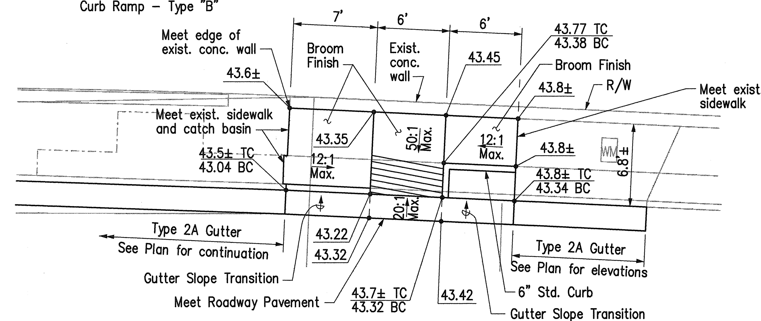
DETAIL E Curb Ramp - Type "B"
