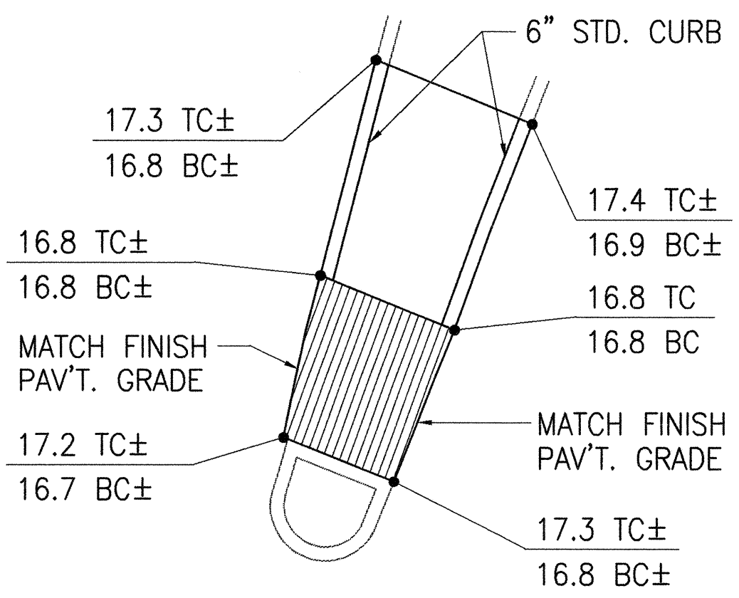
DETAIL RP SCALE: 1"=5' CURB RAMP-MODIFIED TYPE "C"
