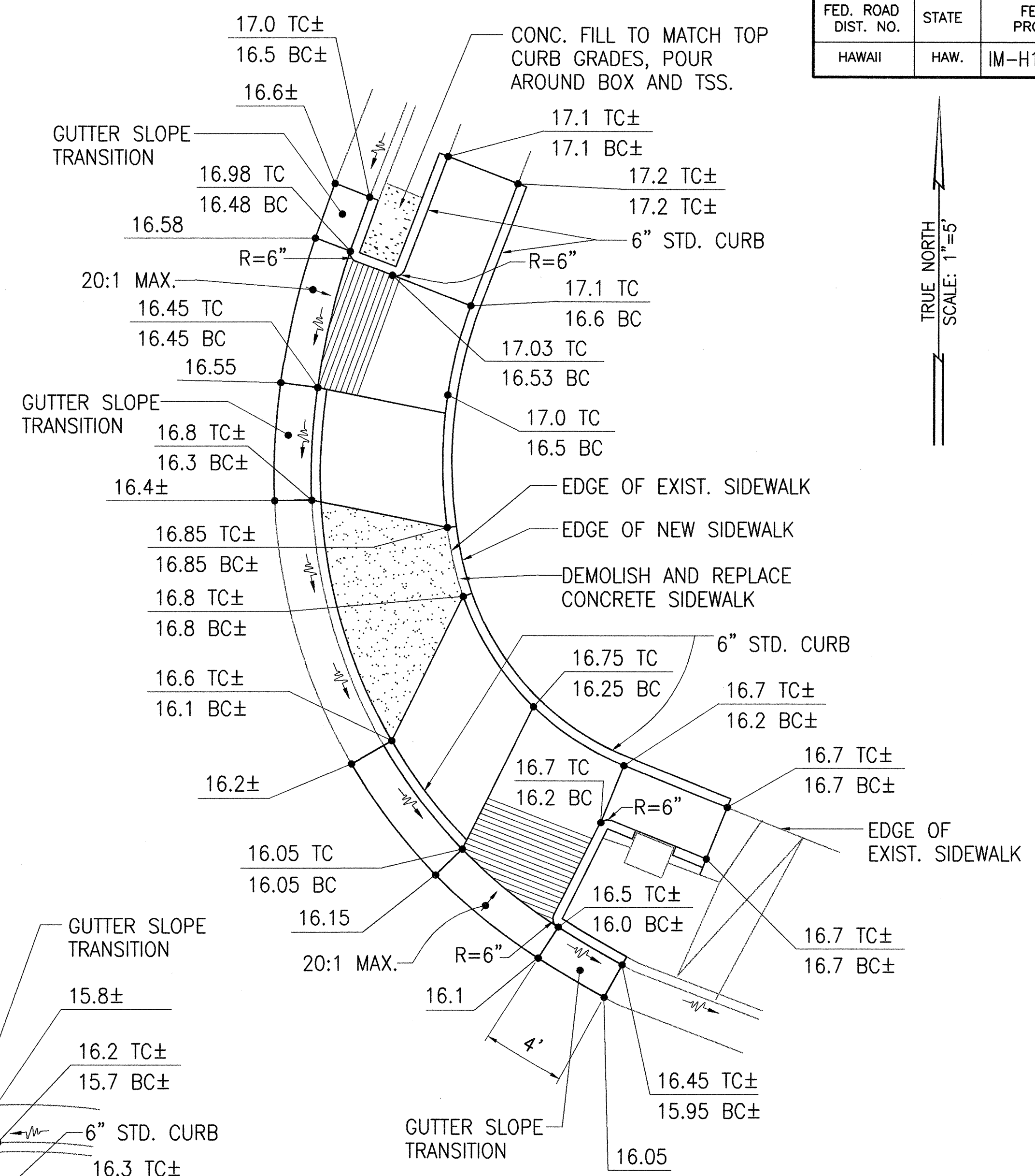
DETAIL RQ SCALE: 1"=5' CURB RAMP-TYPE "B" MODIFIED
