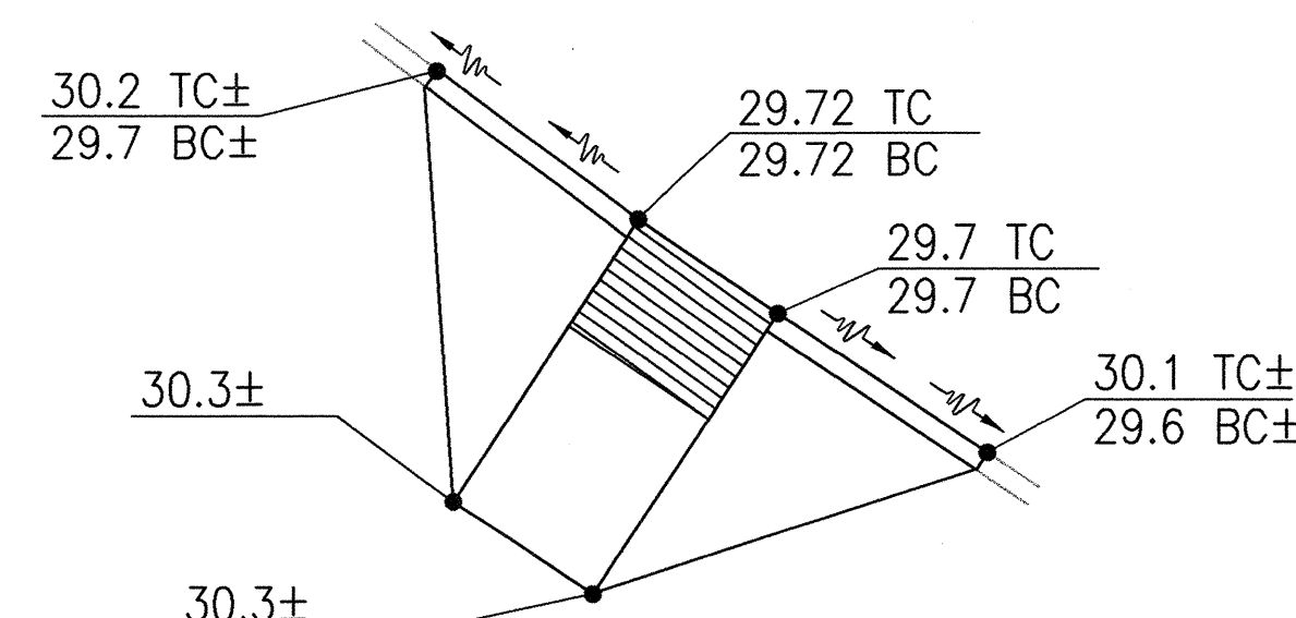
DETAIL RAD SCALE: 1"=5' CURB RAMP-TYPE "A"
