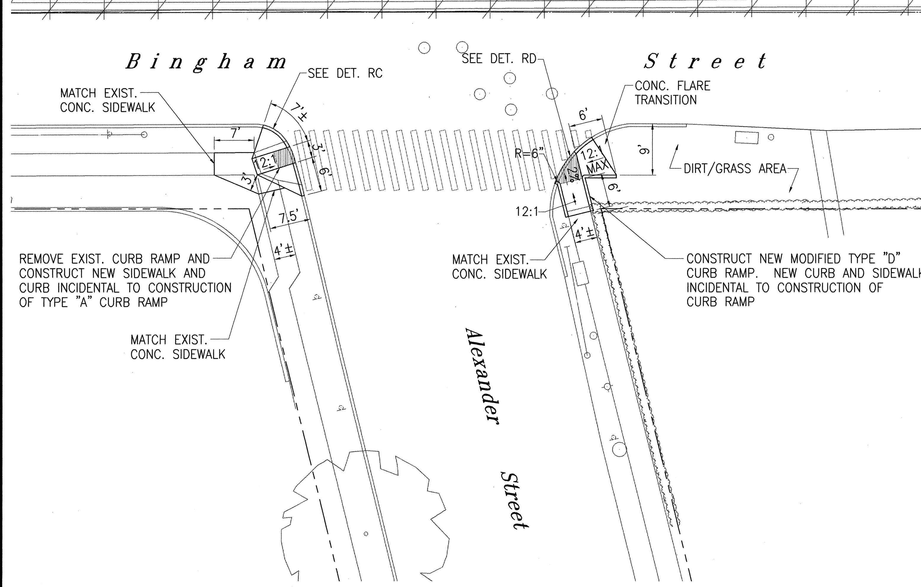
DETAILED ROADWAY PLAN BINGHAM ST./ALEXANDER ST. SCALE: 1"=10'
