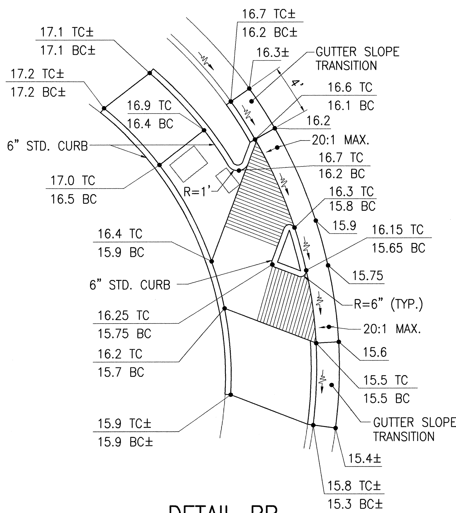
DETAIL RR SCALE: 1"=5' CURB RAMP-TYPE "E" MODIFIED
