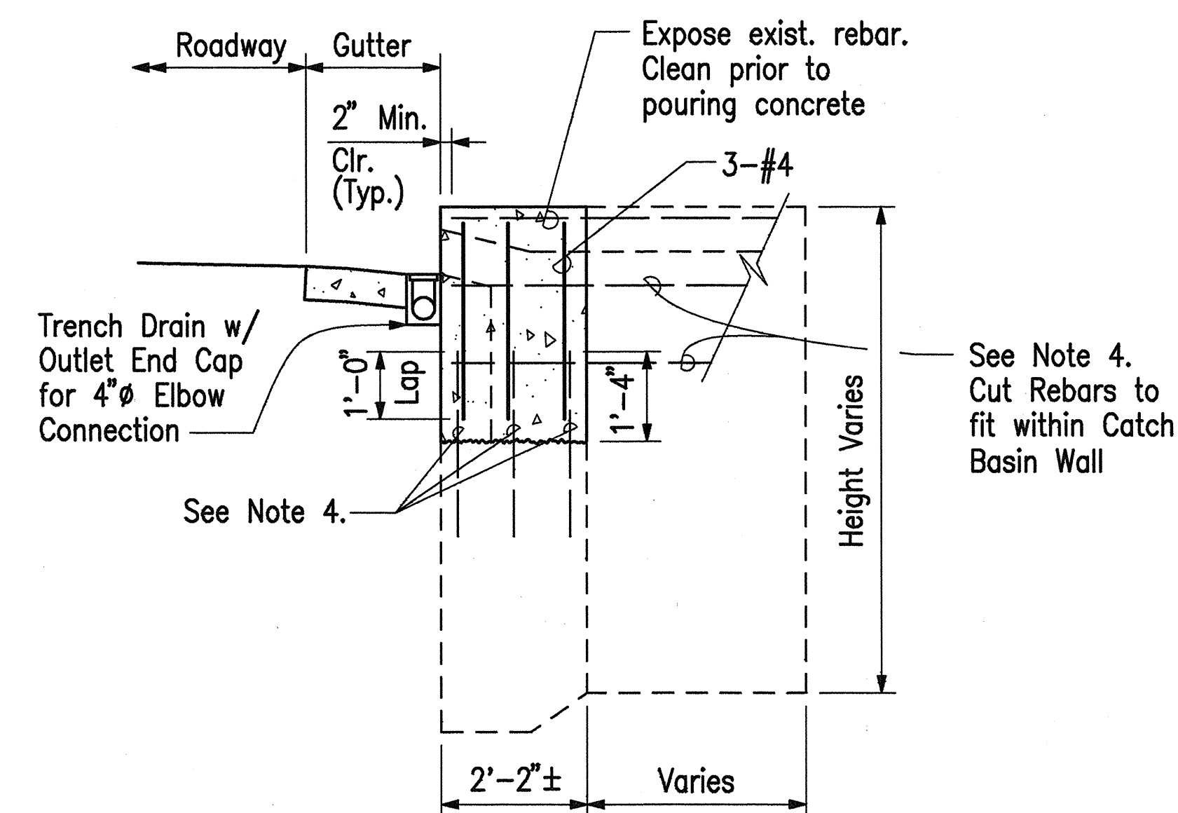
SECTION C Scale: 1/2" = 1'-0" DR19/DR19
