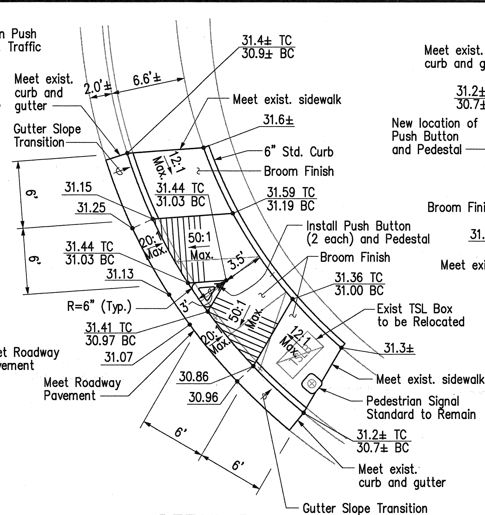
DETAIL B
