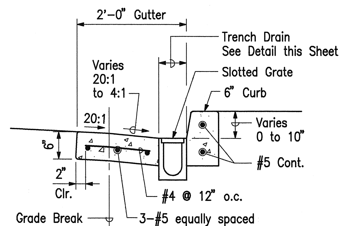
SECTION B Scale: 1" = 1'-0" DR19/DR19
