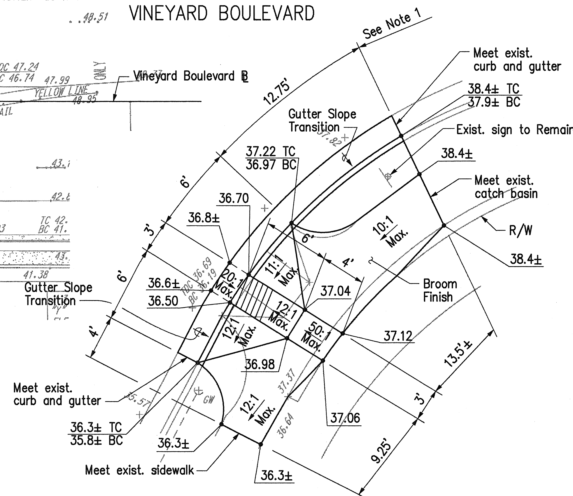
DETAIL C Curb Ramp - Type "A" Scale: 1" = 5'
