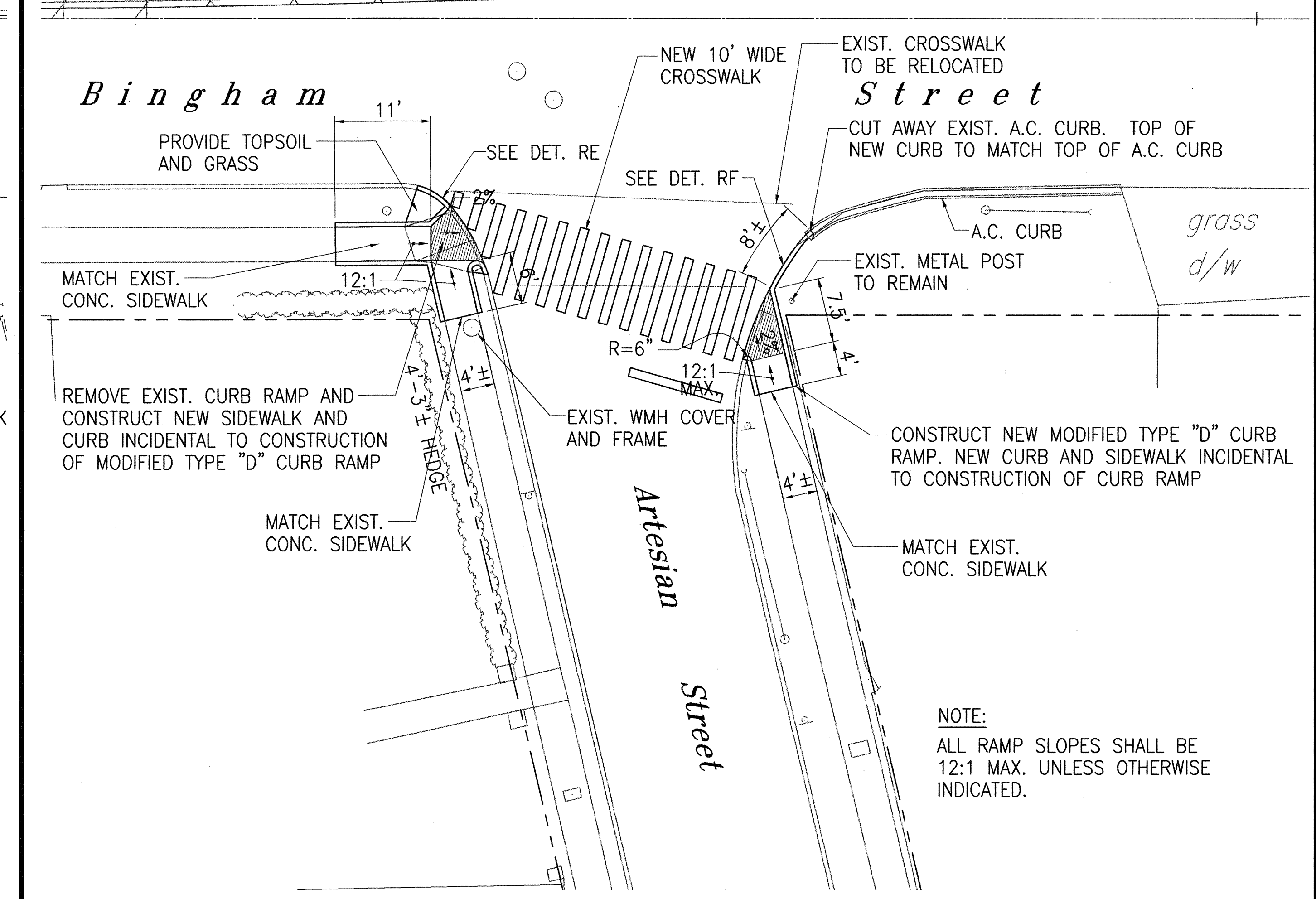
DETAILED ROADWAY PLAN BINGHAM ST./ARTESIAN ST. SCALE: 1"=10'
