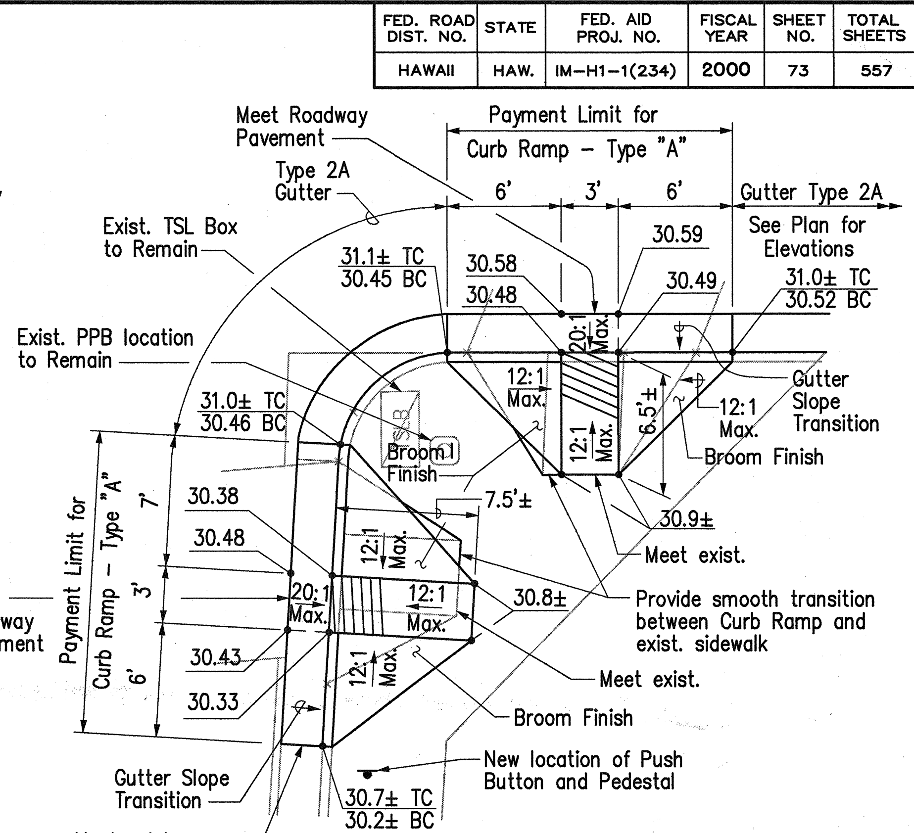
DETAIL D
