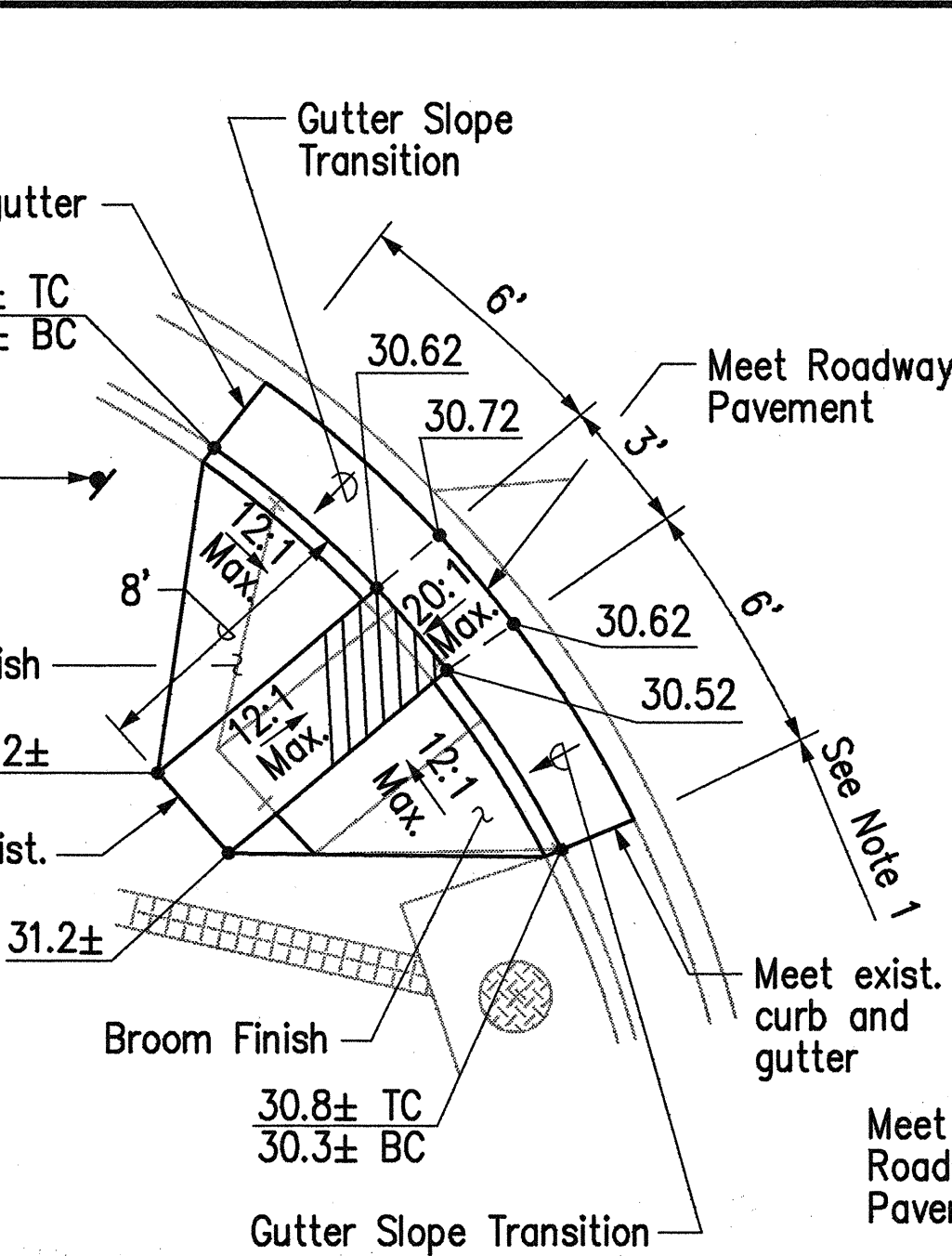
DETAIL C
