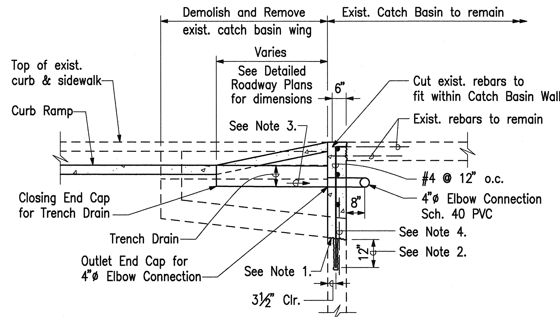
SECTION A Scale: 1/2" = 1'-0" DR19/DR19
