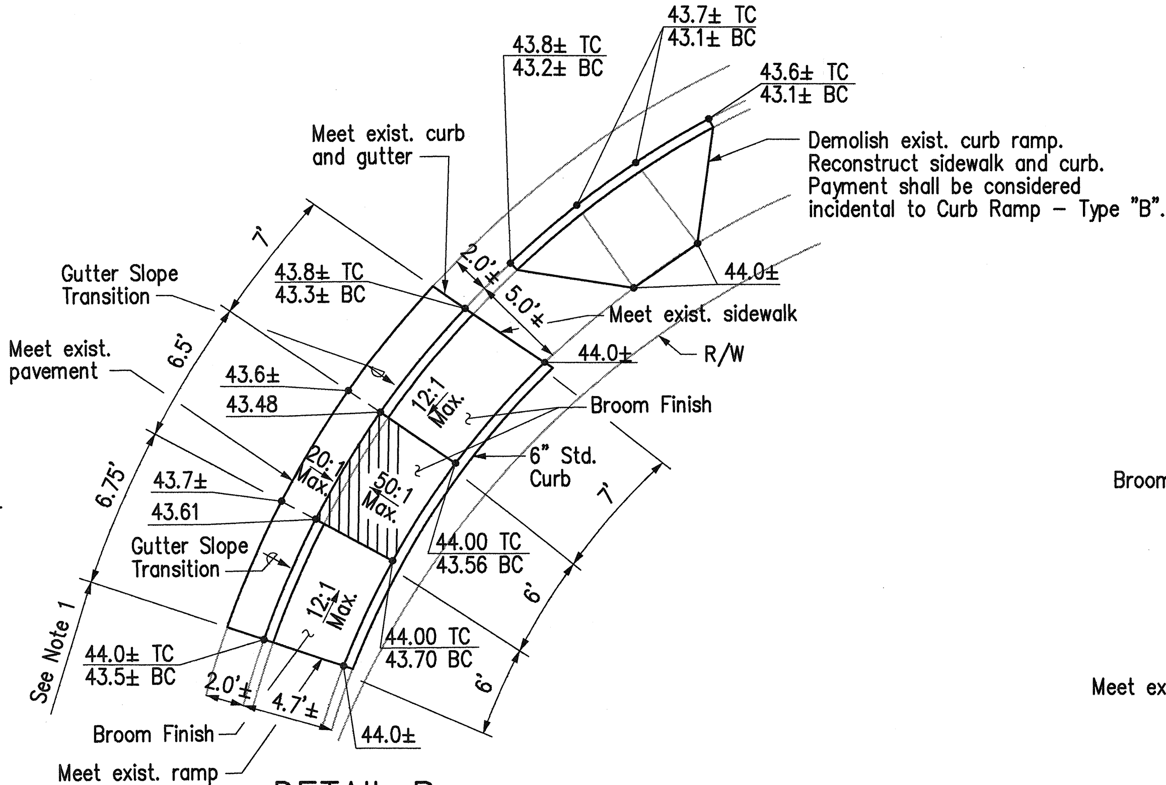
DETAIL B Curb Ramp - Type "B"
