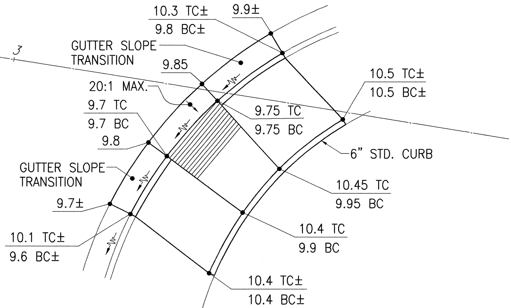
DETAIL RN SCALE: 1"=10' CURB RAMP-TYPE "B" MODIFIED
