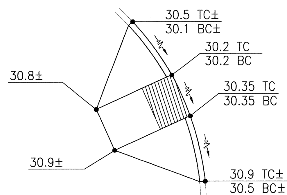
DETAIL RAB SCALE: 1"=5' CURB RAMP-TYPE "A"
