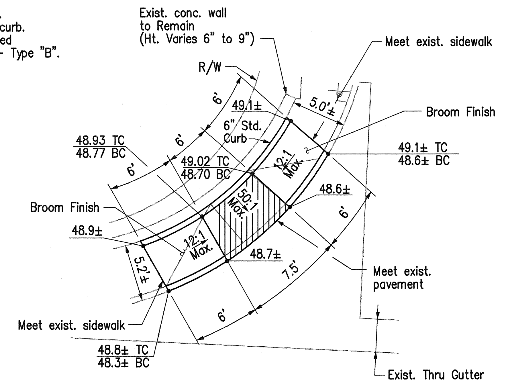
DETAIL C Curb Ramp - Type "B"
