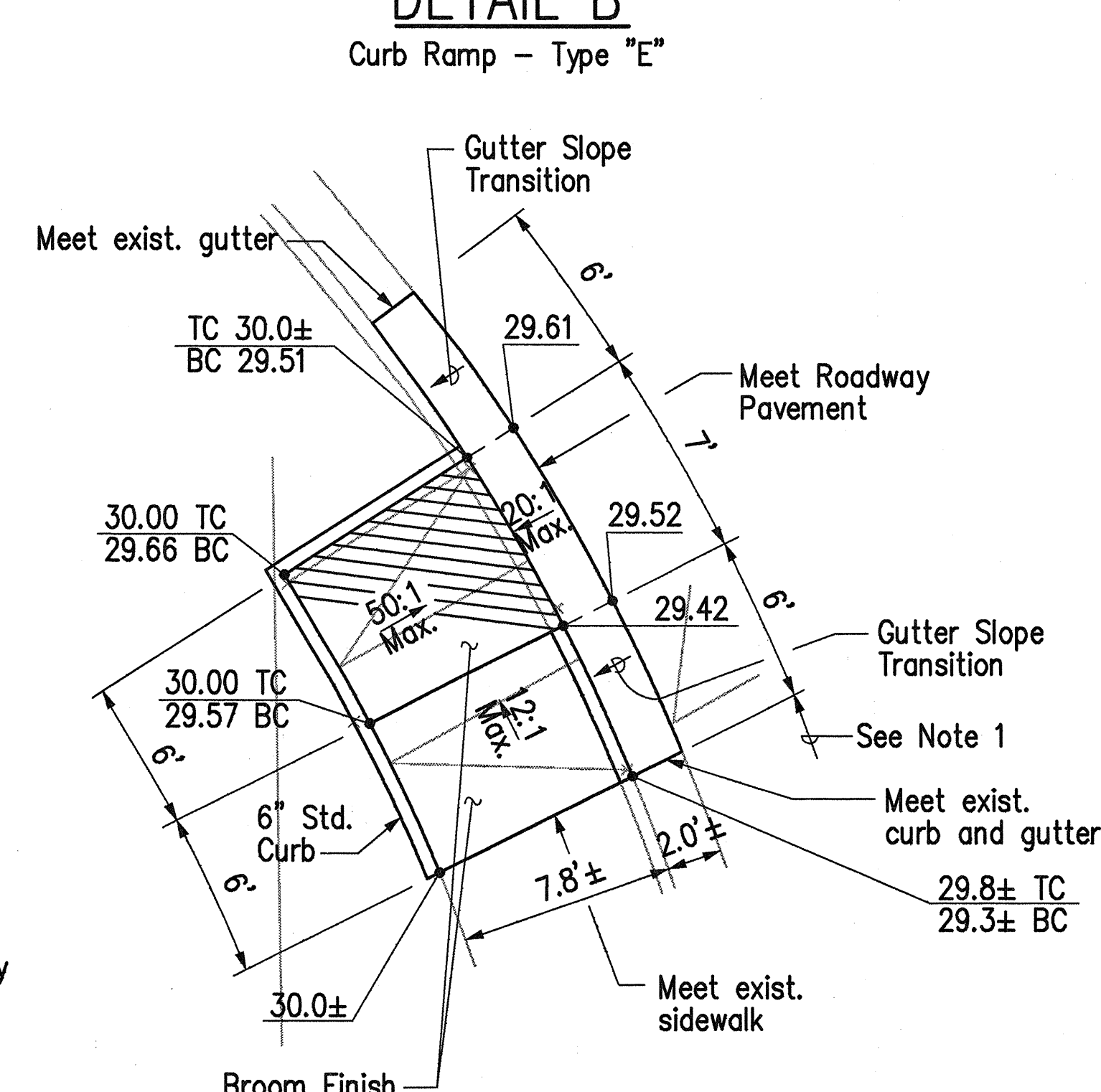
DETAIL B
