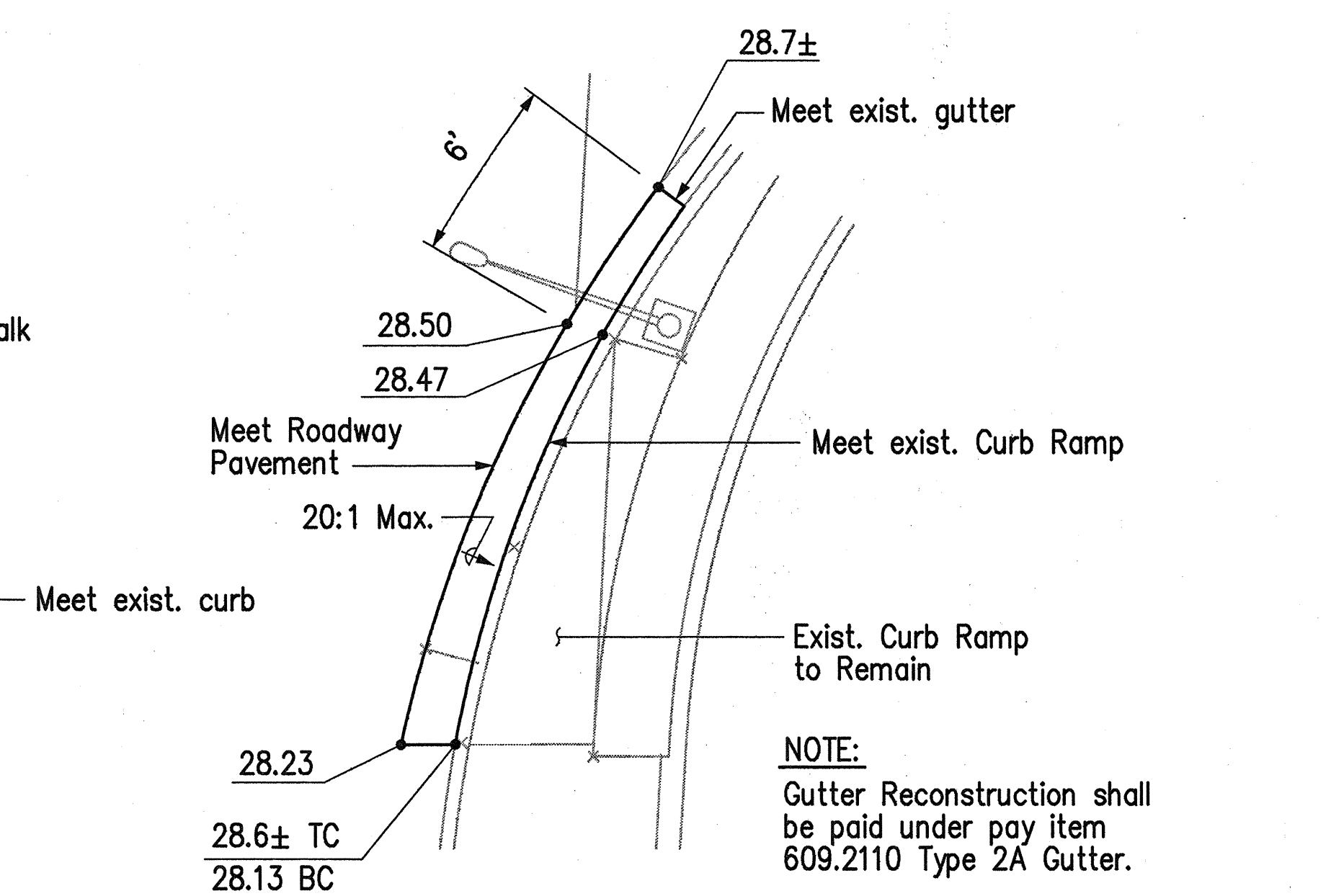
DETAIL H
