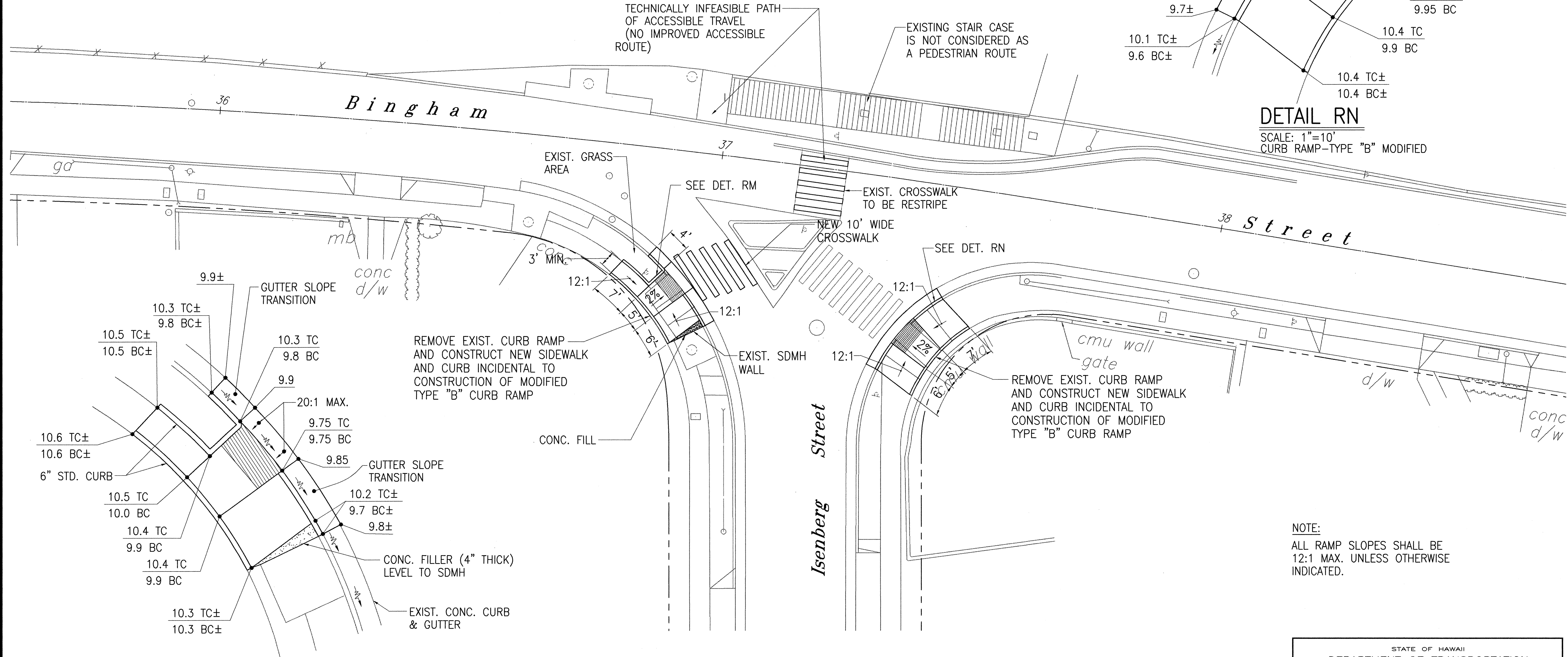
DETAIL RM SCALE: 1"=10' CURB RAMP-TYPE "B" MODIFIED
