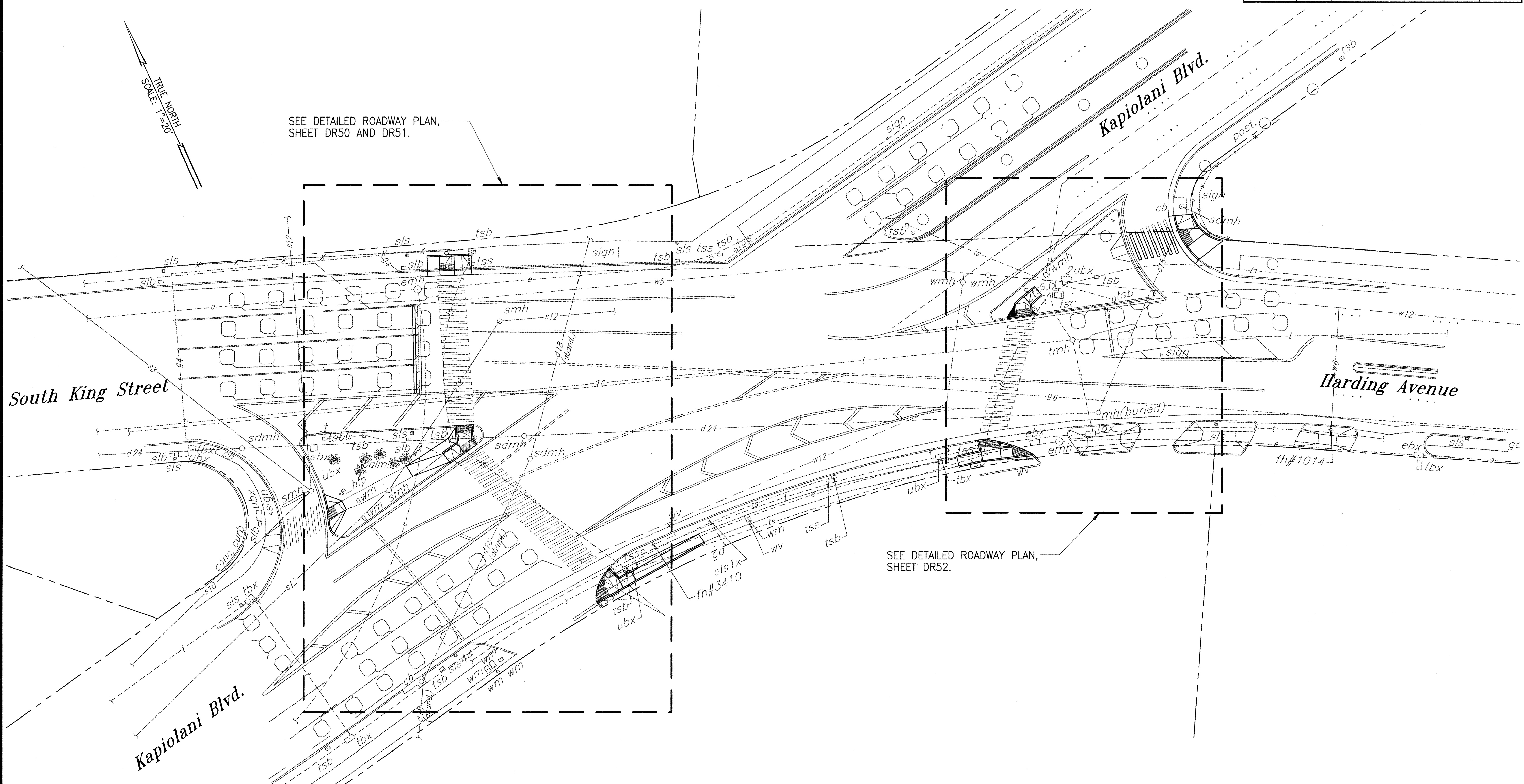
DETAILED ROADWAY PLAN SCALE: 1"=20'
