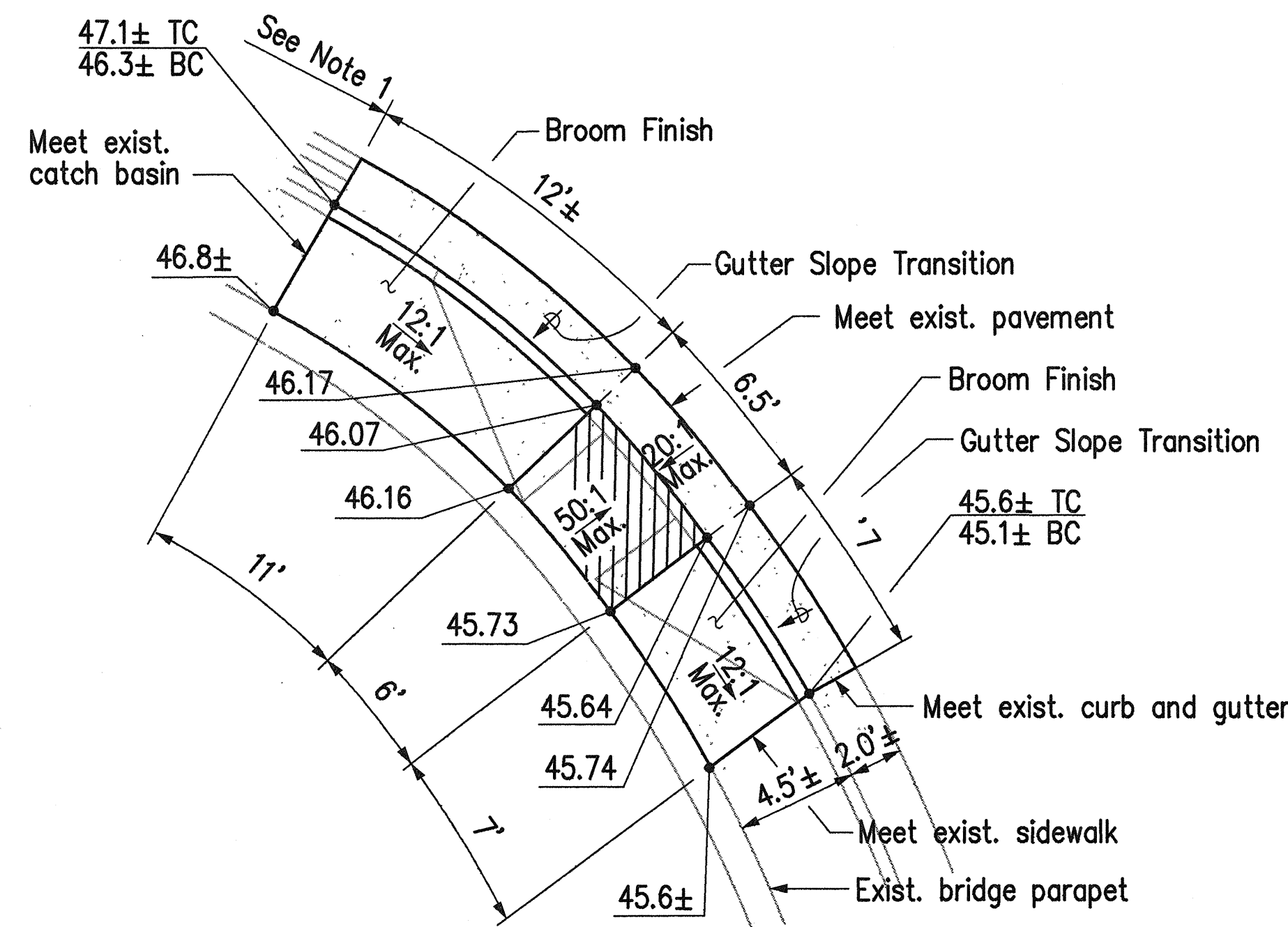
DETAIL A Curb Ramp - Type "B"
