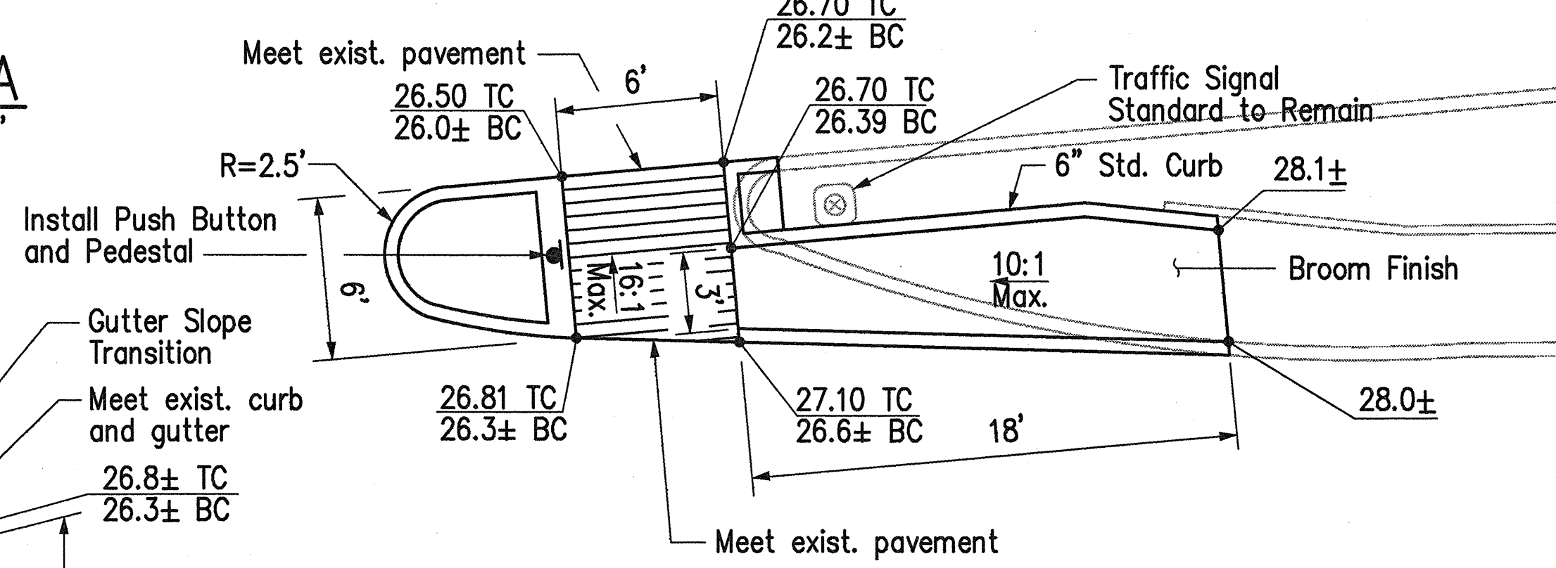
DETAIL D Curb Ramp - Type "C" Scale: 1" = 5'
