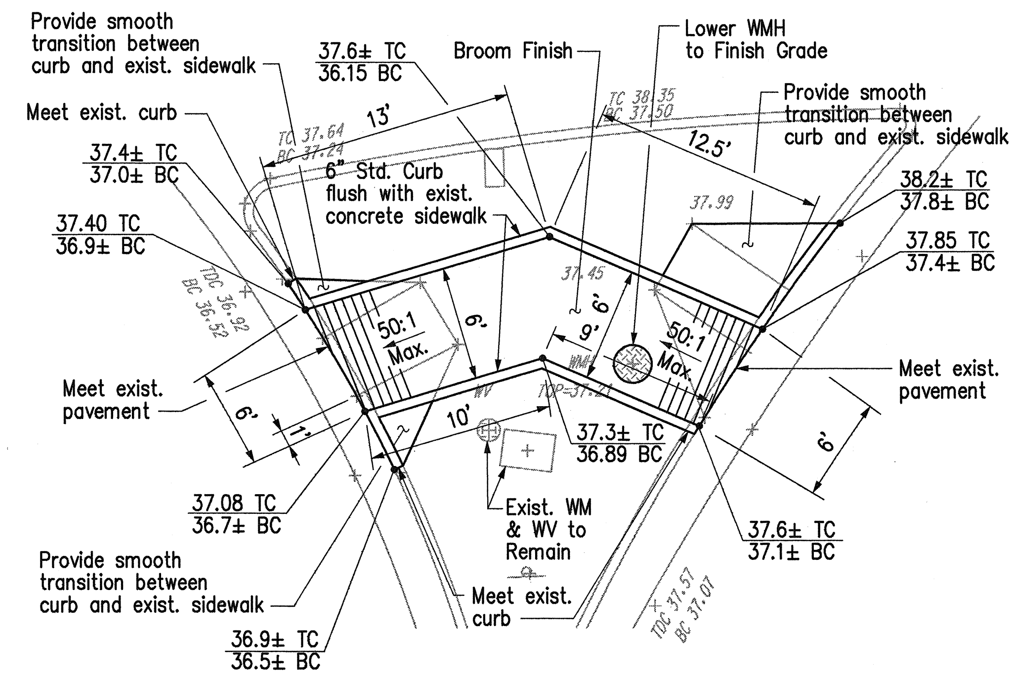
DETAIL B Curb Ramp - Type "C" Modified Scale: 1" = 5'
