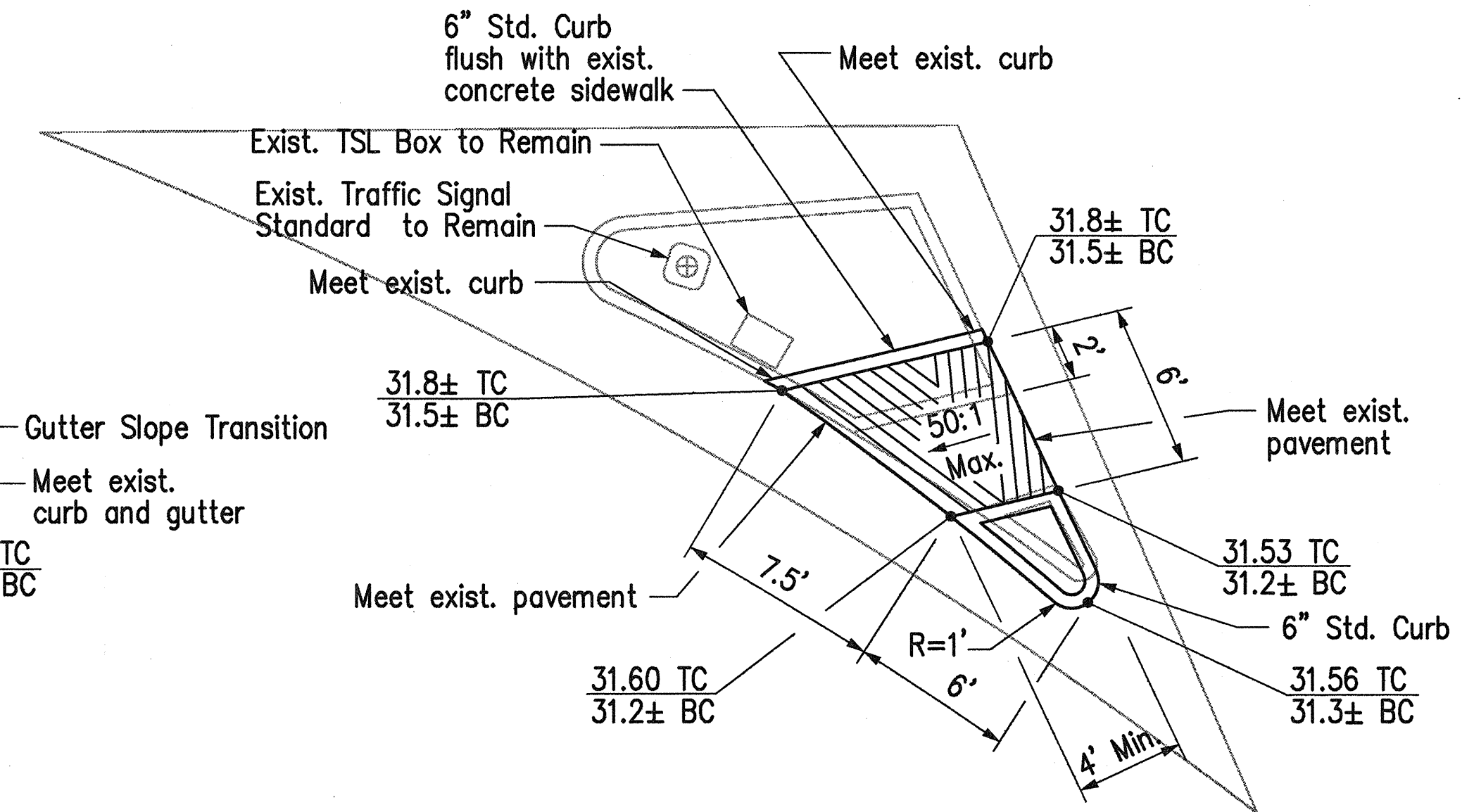
DETAIL J
