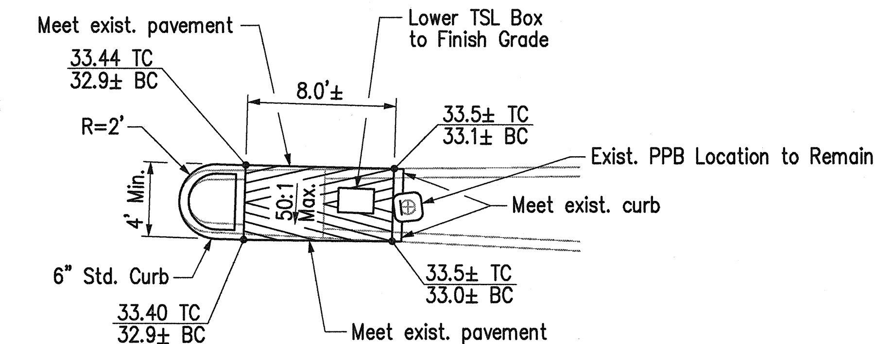
DETAIL M
