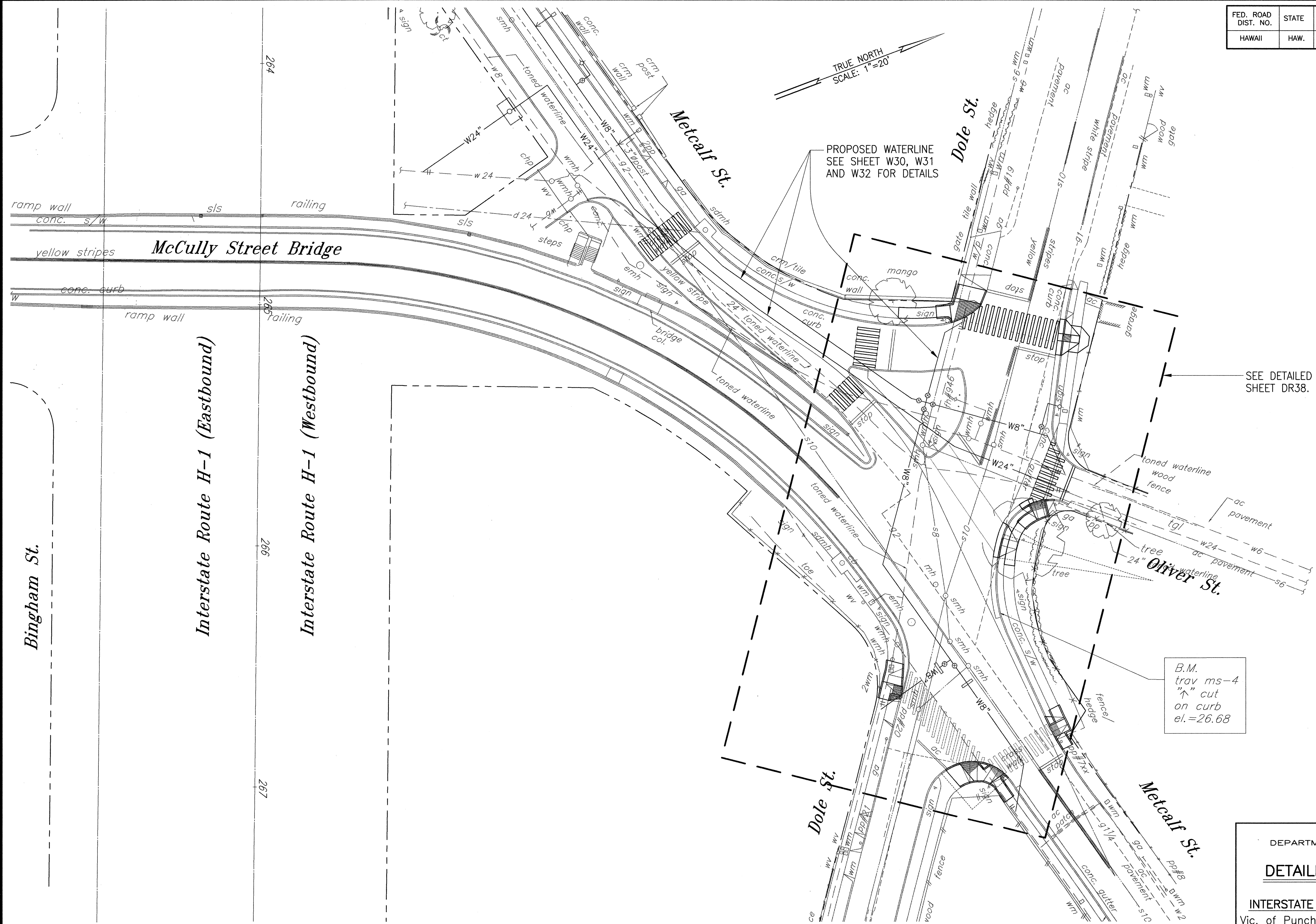
DETAILED ROADWAY PLAN SCALE: 1"=20'
