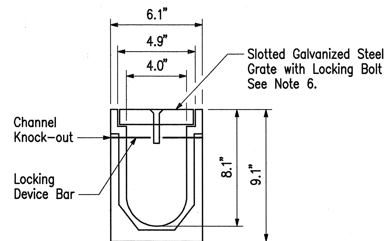
TRENCH DRAIN DETAIL Not to Scale
