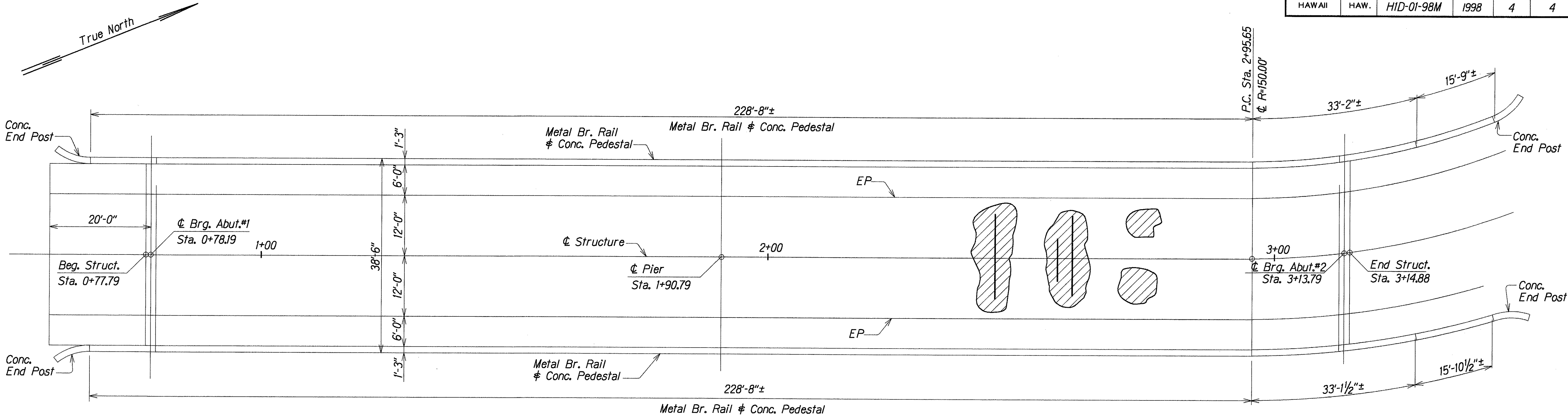
LAYOUT PLAN Scale : 1" = 10'-0"
