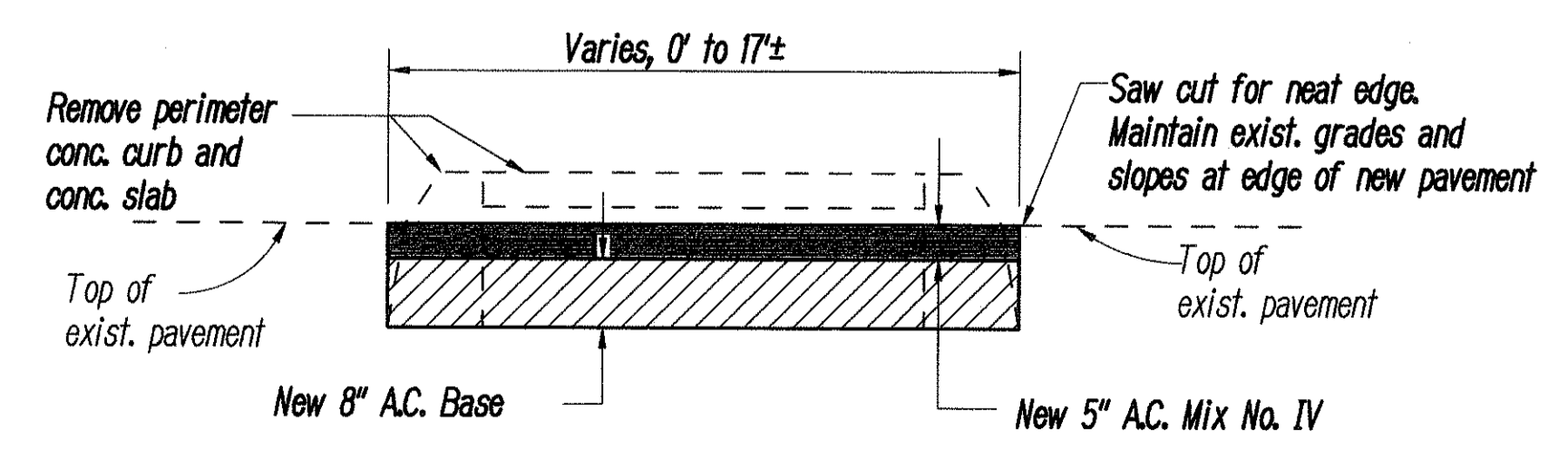
SECTION THROUGH EXISTING ISLAND Not to Scale
