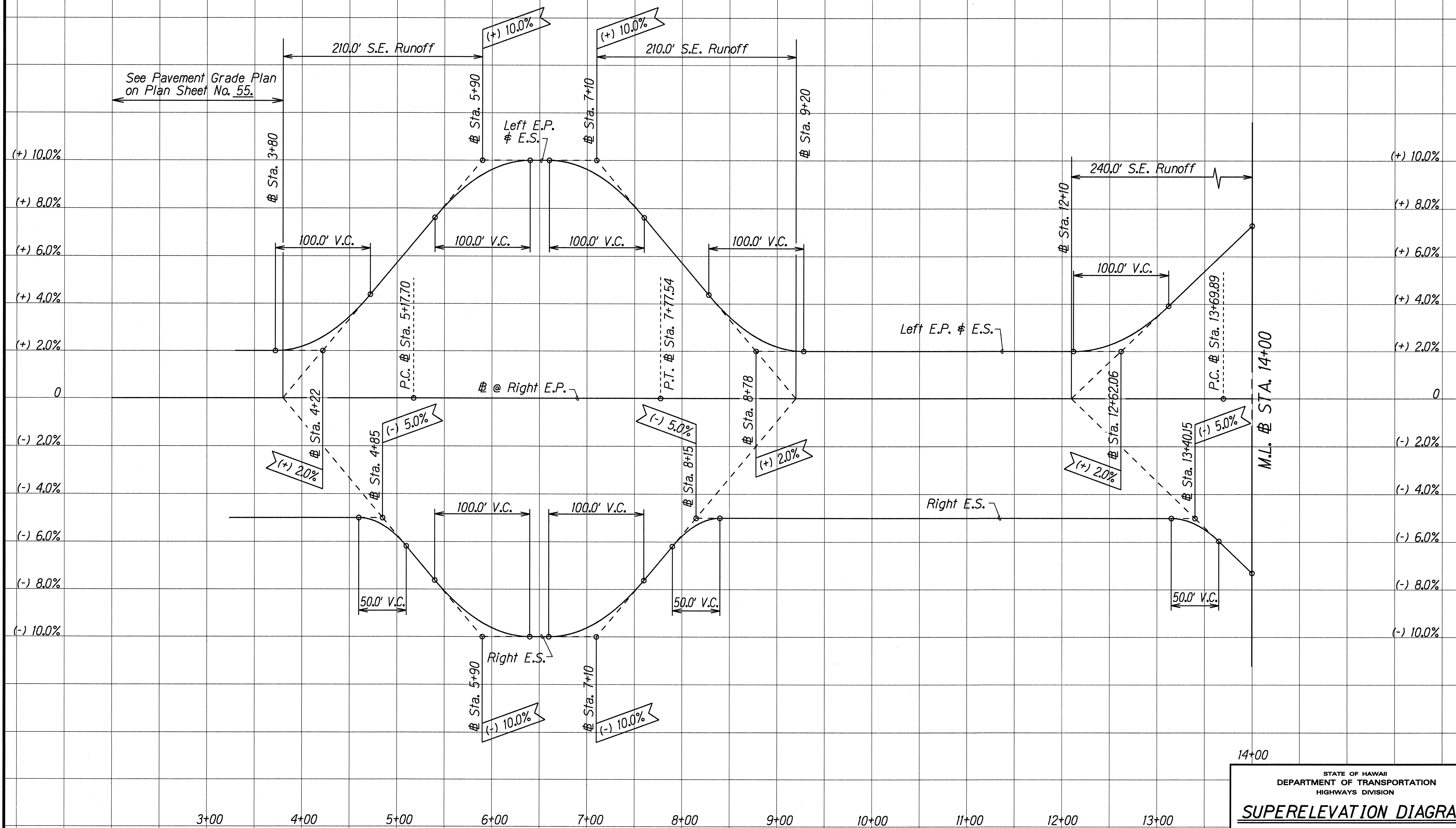
SUPERELEVATION DIAGRAM - RAMP HE
