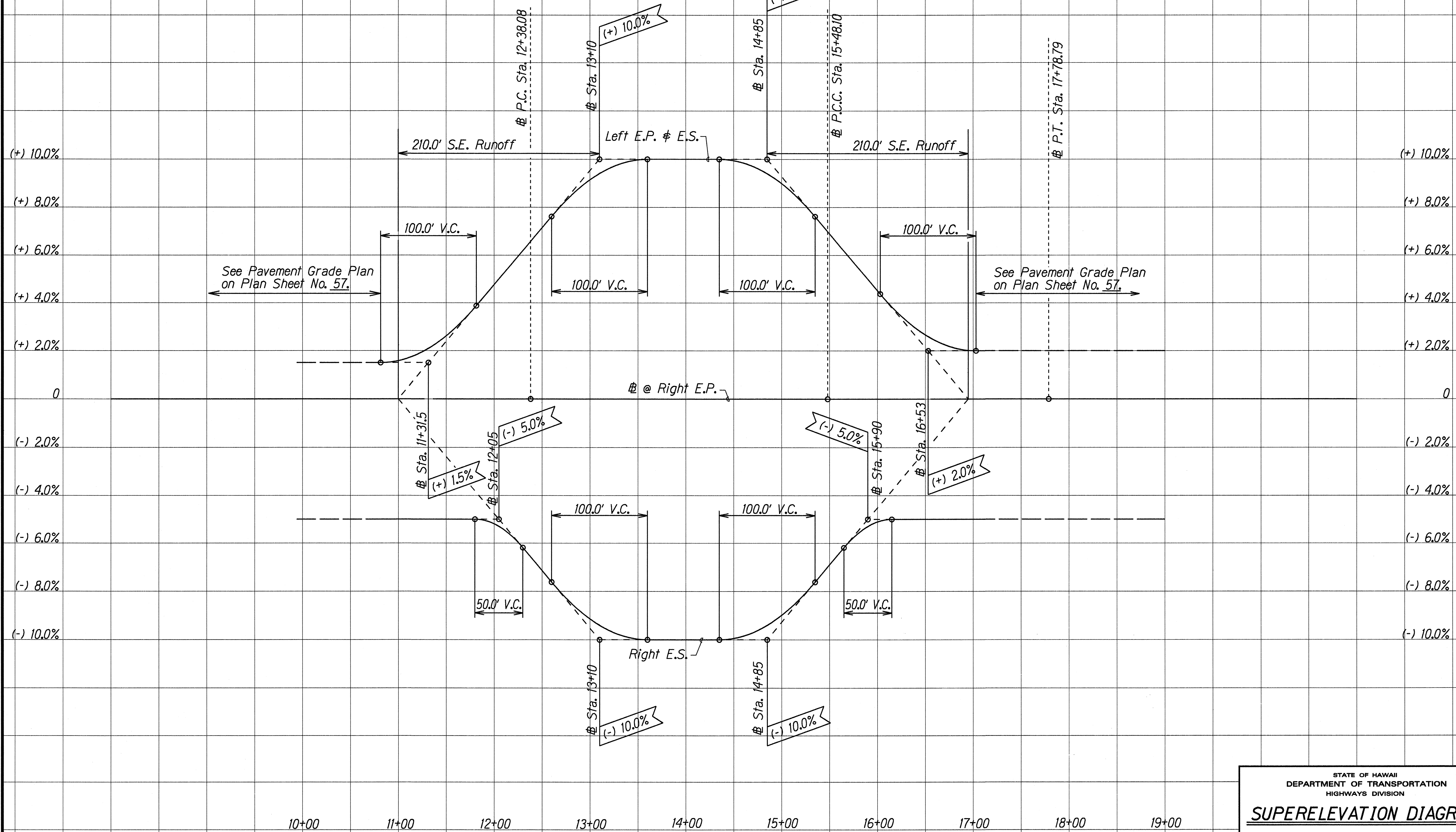
SUPERELEVATION DIAGRAM - RAMP WE
