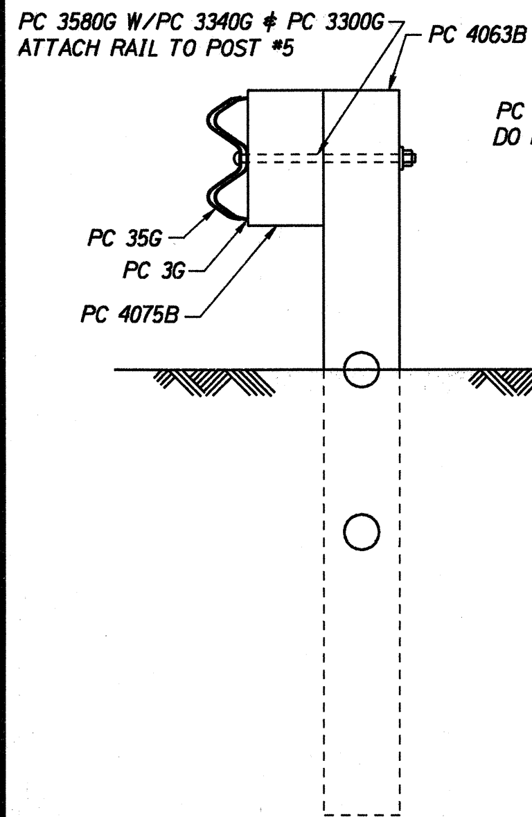
SECTION "D-D" (@ POST #5)
