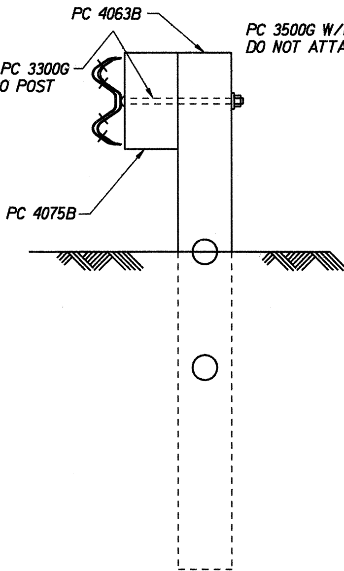
SECTION "B-B" (@ POSTS #3 & #7)
