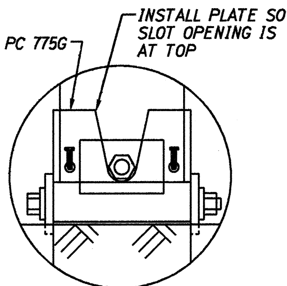
BEARING PLATE ORIENTATION
