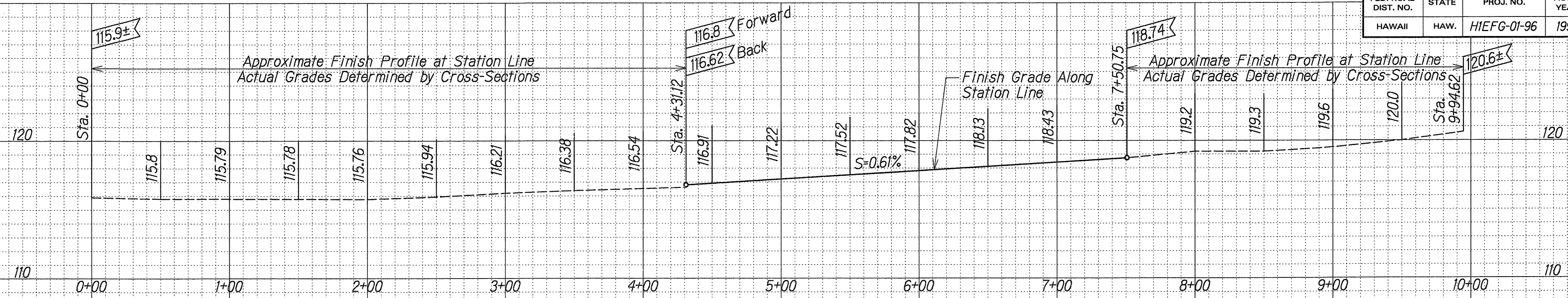
§ PROFILE - CROSS-OVER NO. 1 Scale: Horiz. 1"= 40'-0" Vert. 1"= 4'-0"
