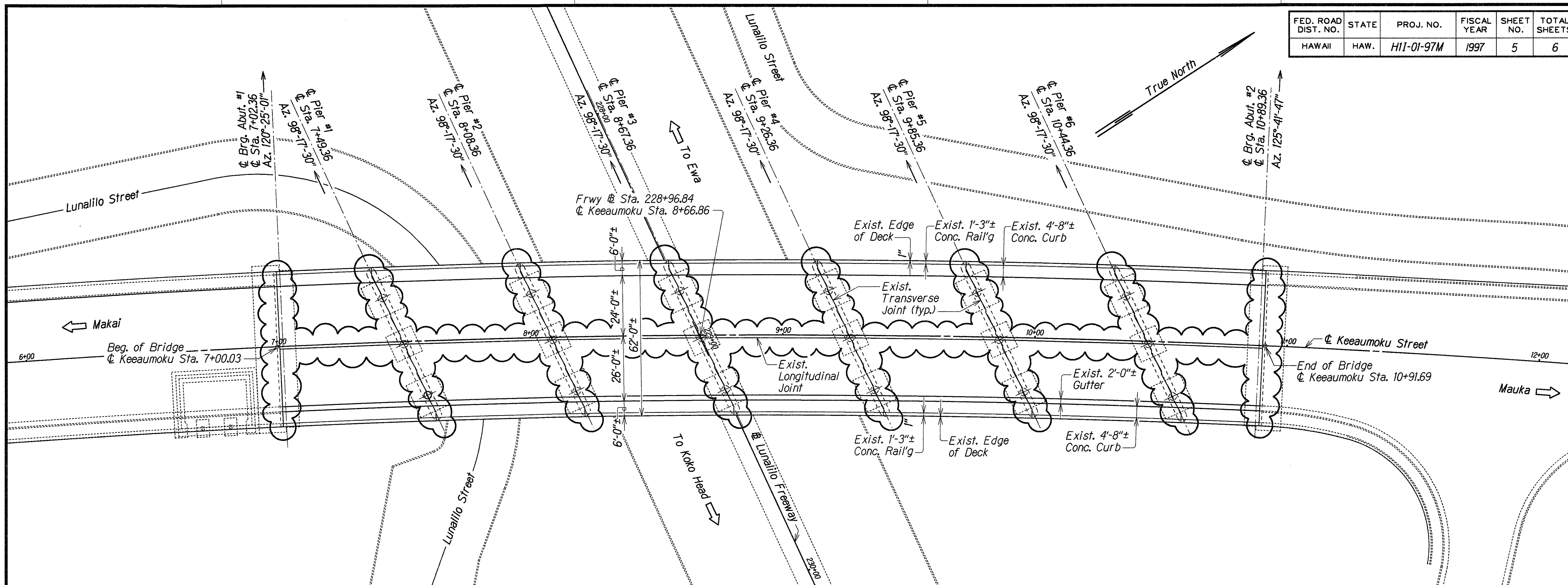
LAYOUT PLAN--KEEAUMOKU STREET SEPARATION Scale: 1" = 20'-0"
