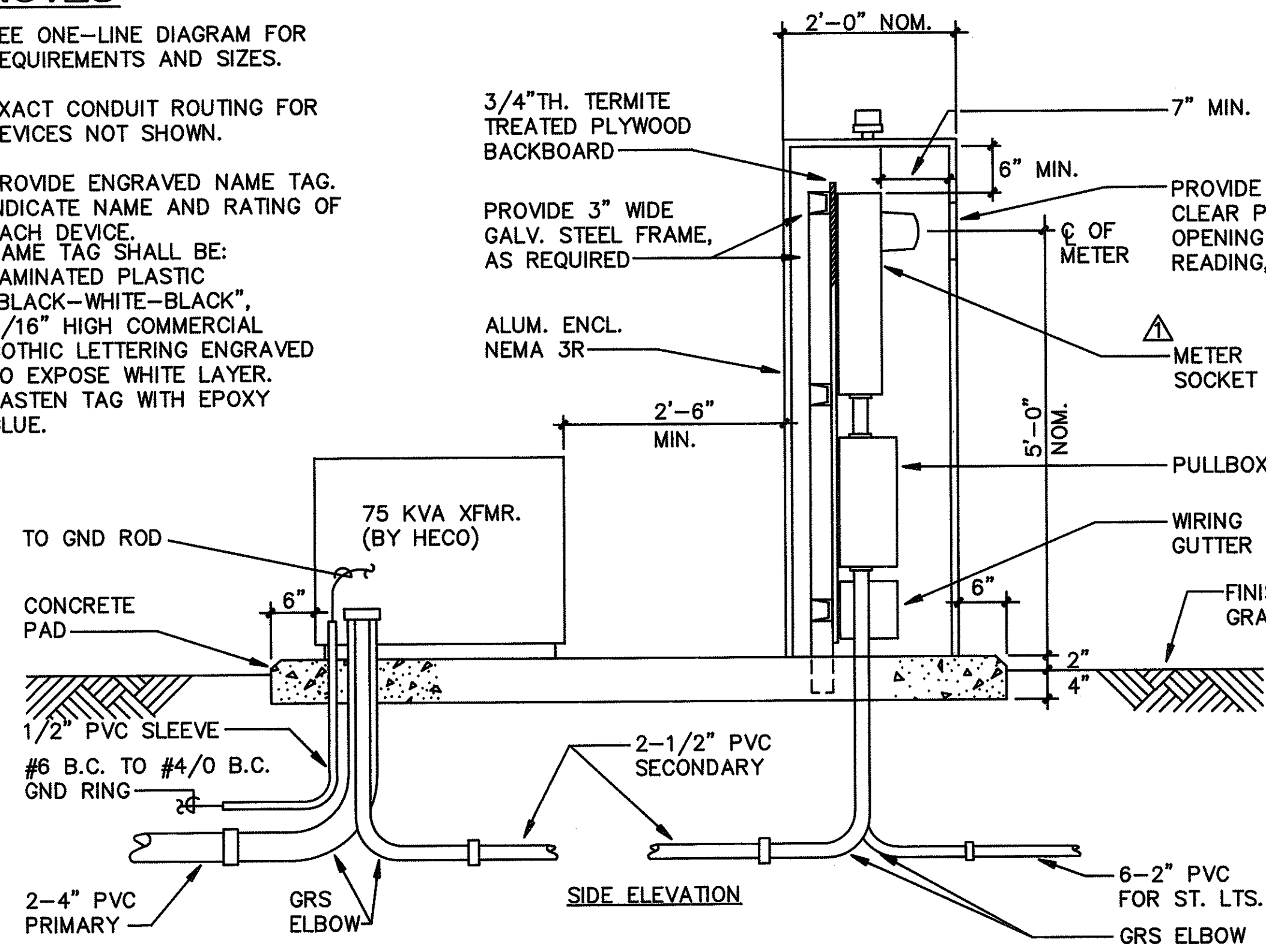
DISTRIBUTION CENTER "A" NOT TO SCALE
