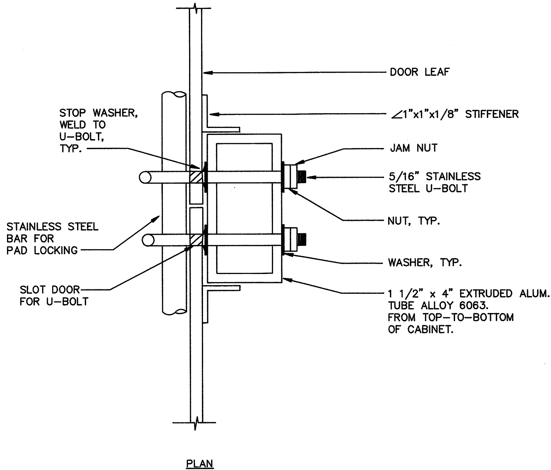
PLAN
