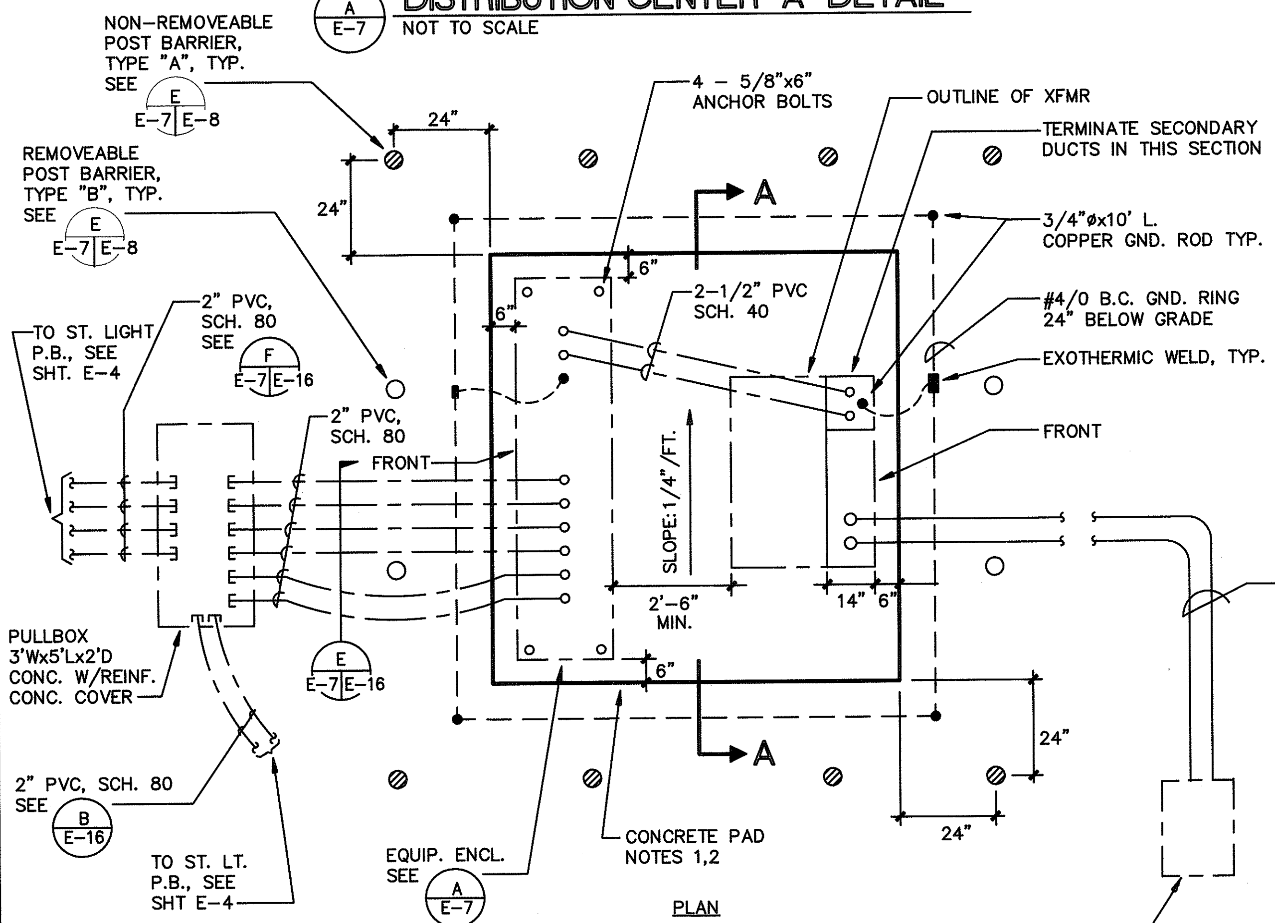
STREET LIGHT TRANS. & EQUIP. ENCL. NOT TO SCALE
