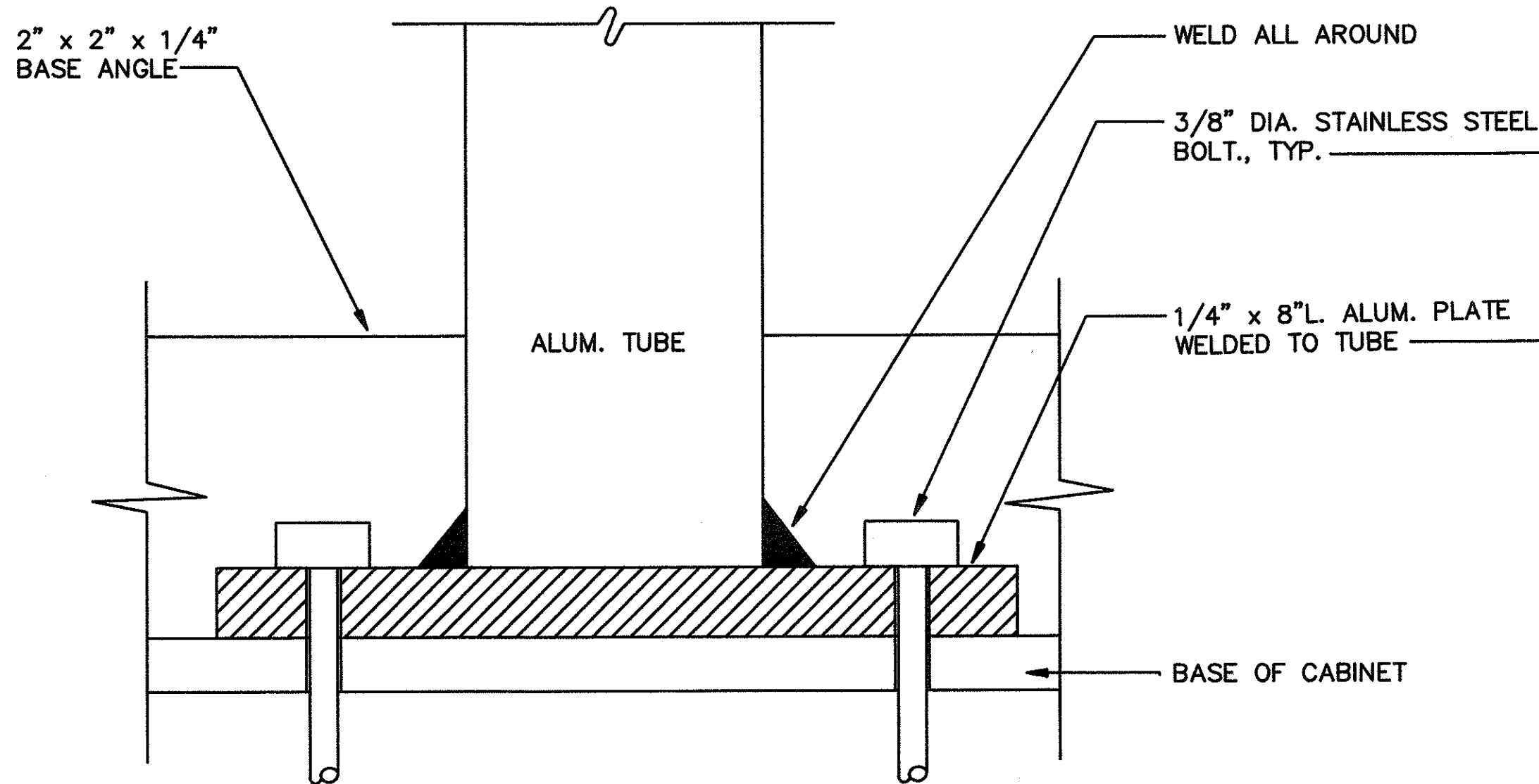
FRONT ELEVATION
