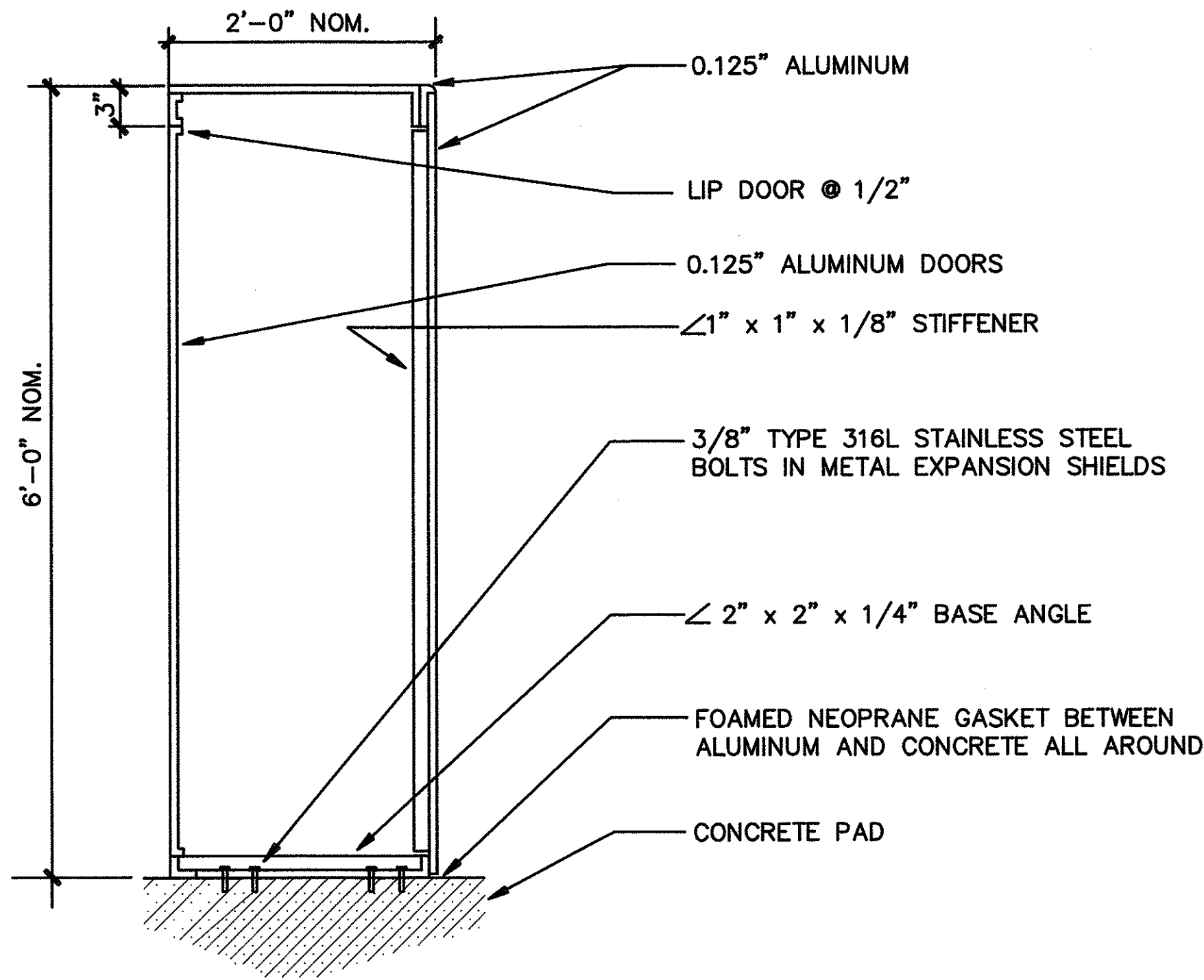
SECTION
