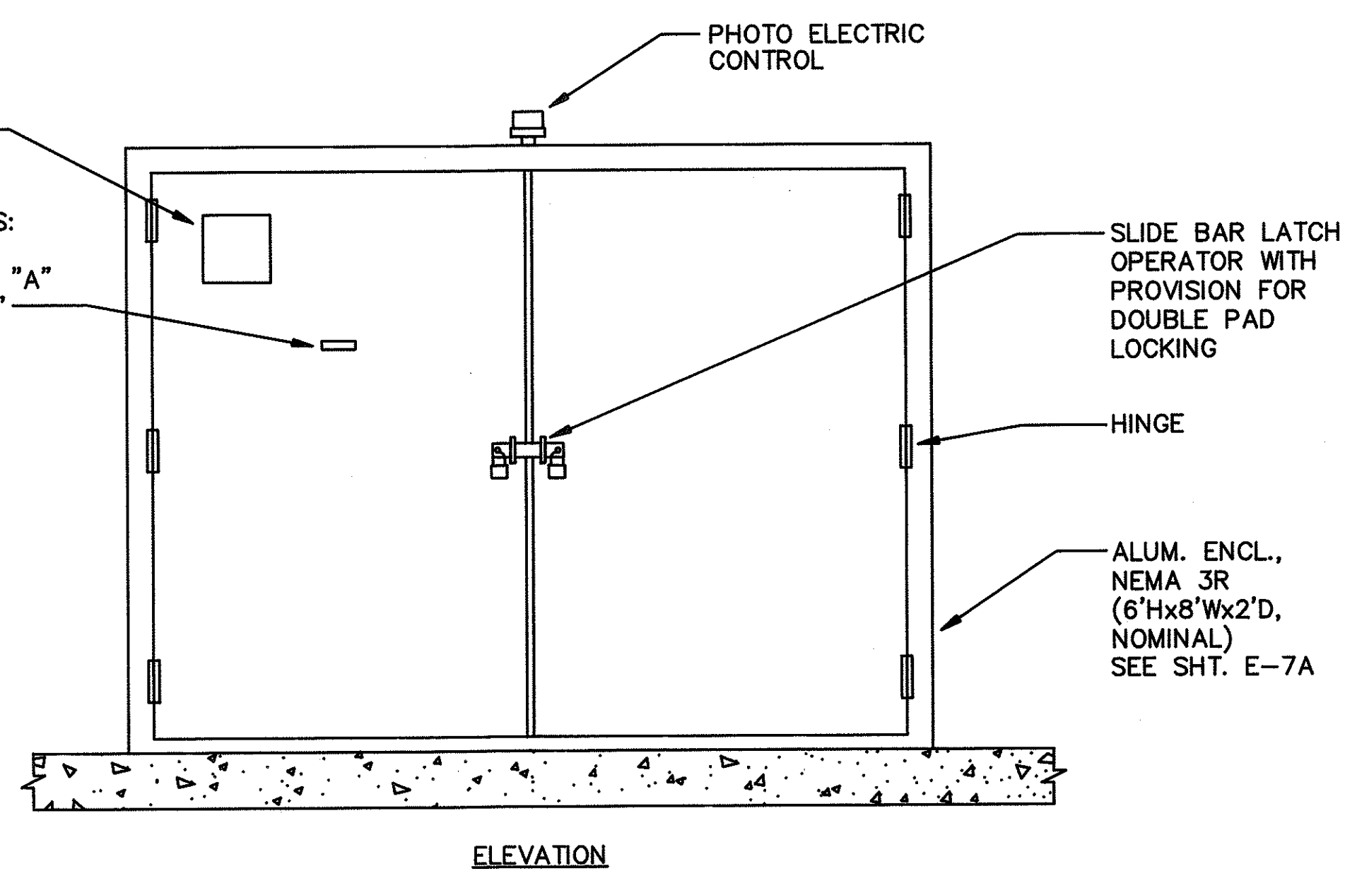
EQUIPMENT ENCLOSURE NOT TO SCALE
