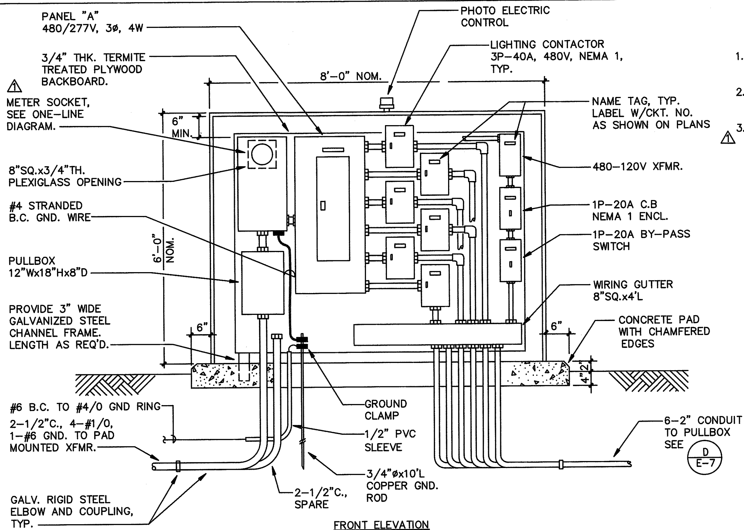
DISTRIBUTION CENTER "A" DETAIL NOT TO SCALE
