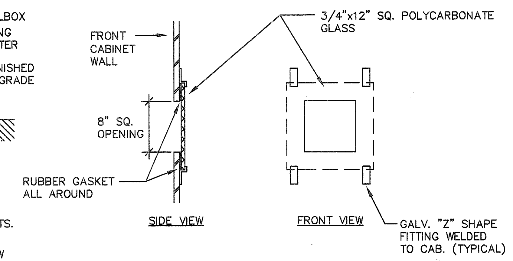
METER WINDOW DETAIL NOT TO SCALE
