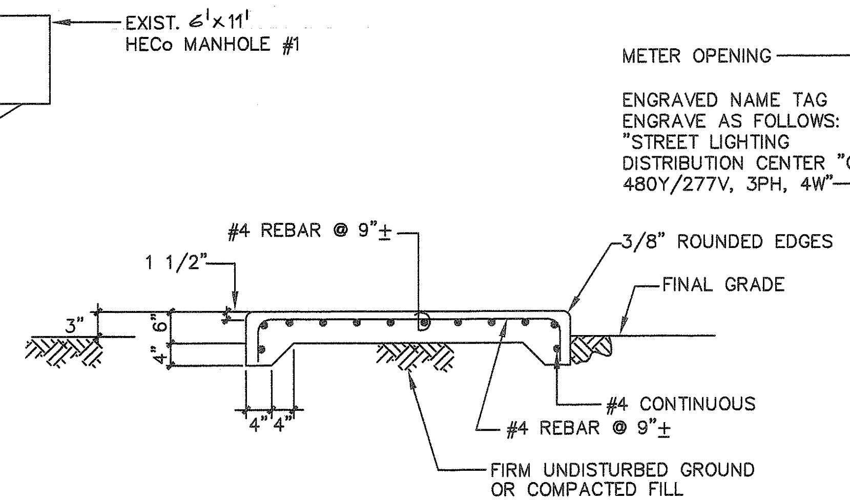
DISTRIBUTION CENTER "C" NOT TO SCALE
