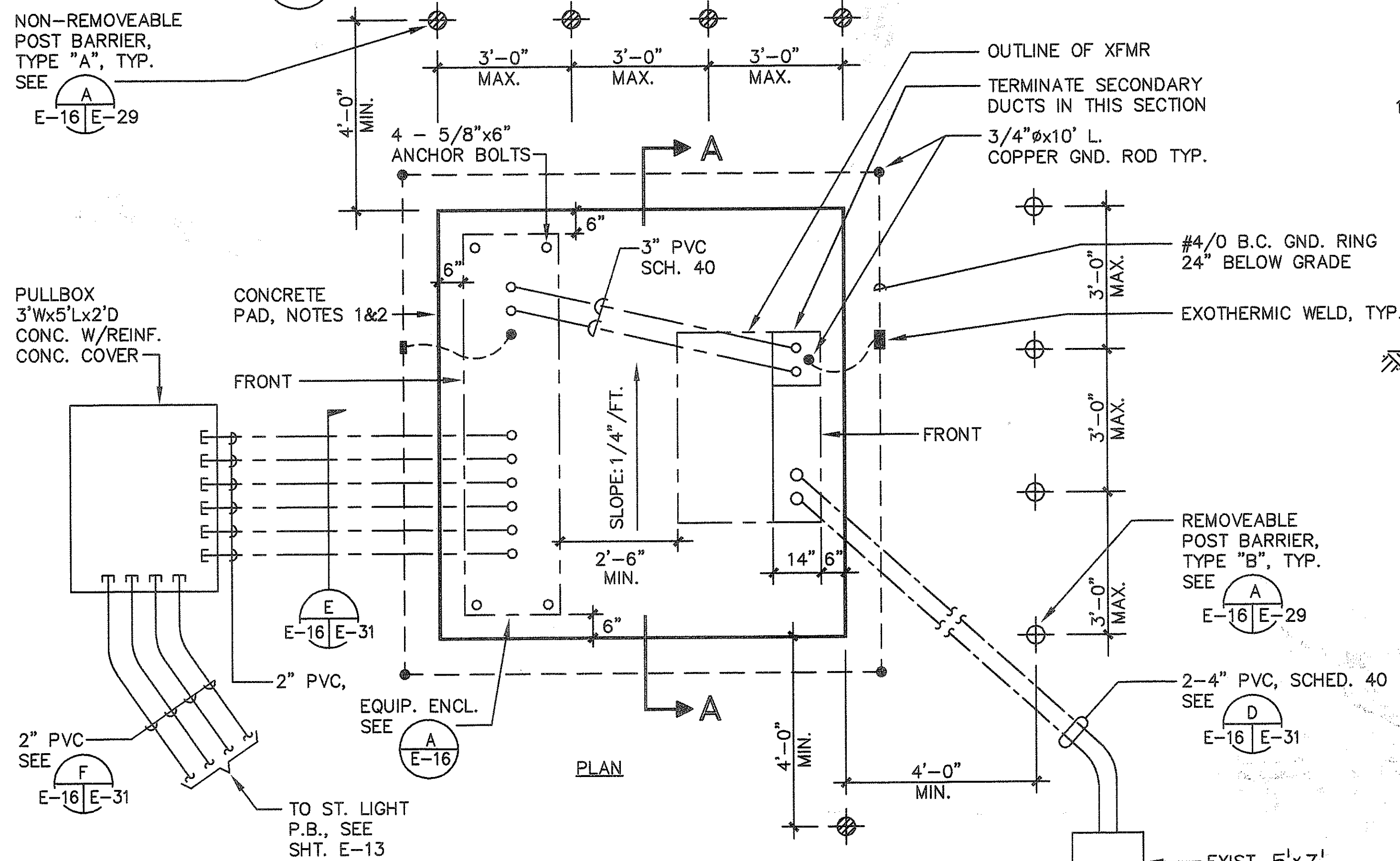
STREET LIGHT XFMR & EQUIP. ENCL. NOT TO SCALE
