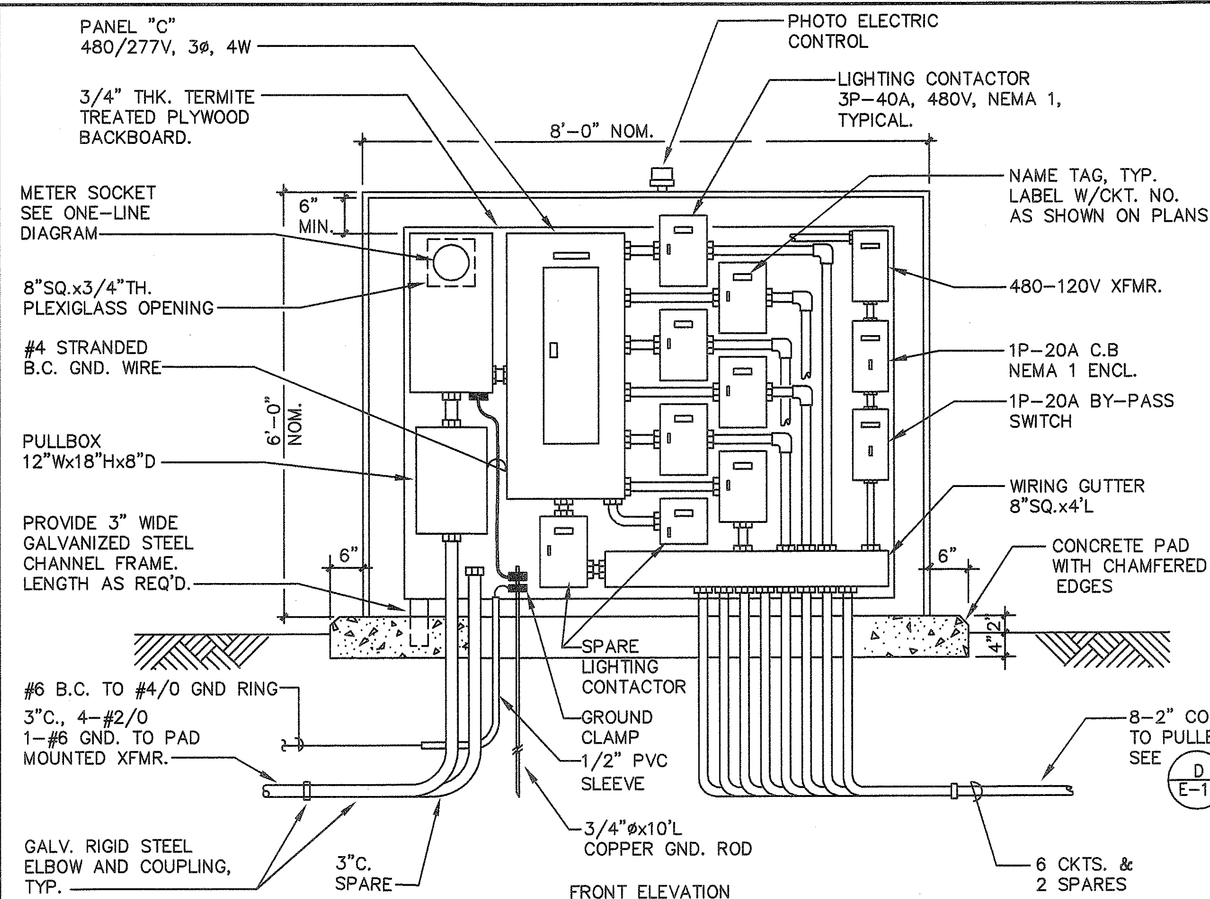
DISTRIBUTION CENTER "C" NOT TO SCALE
