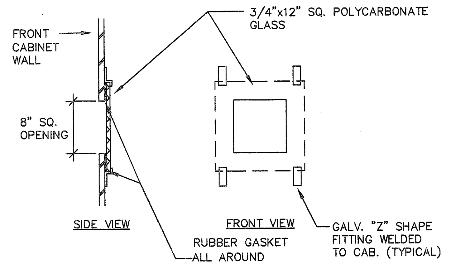
METER WINDOW DETAIL NOT TO SCALE
