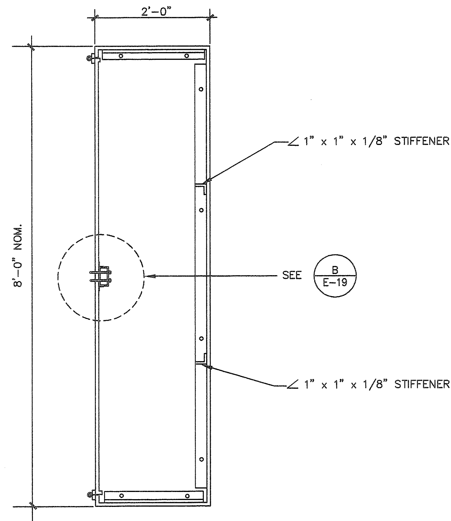
PLAN
