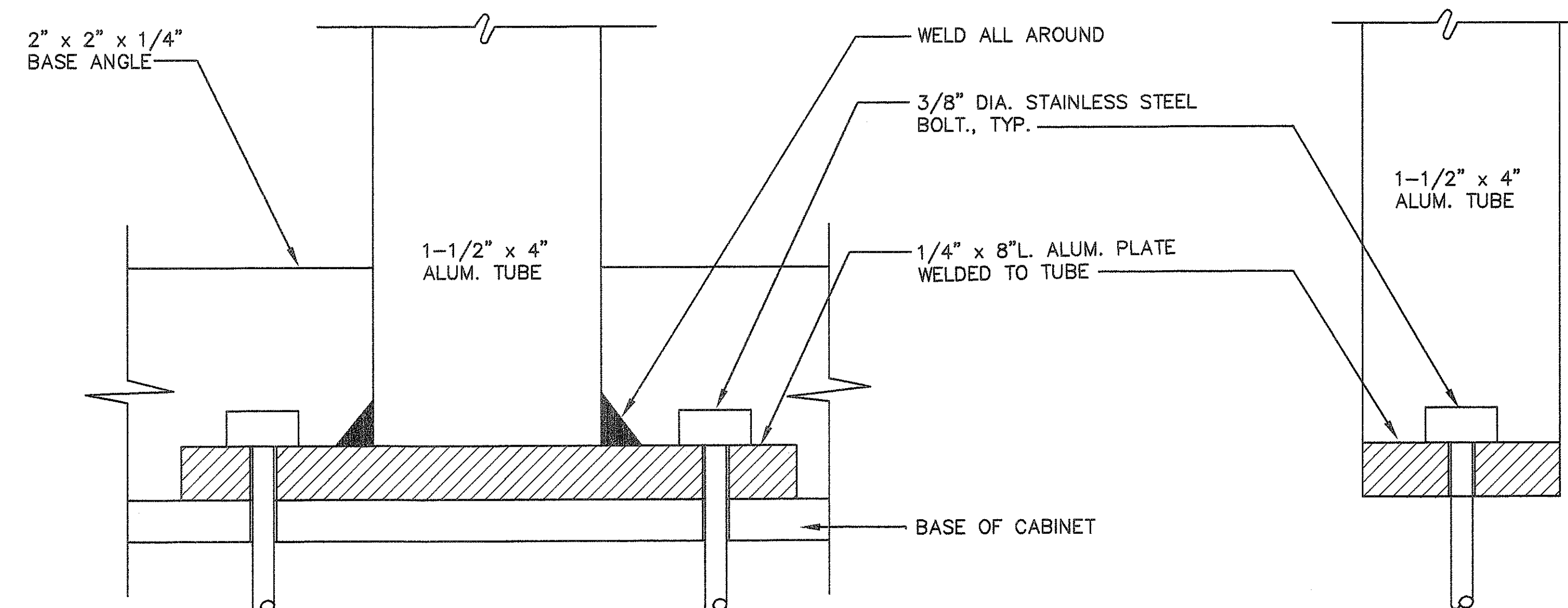
SIDE ELEVATION
