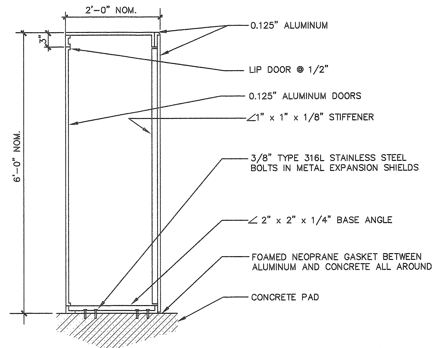
SECTION
