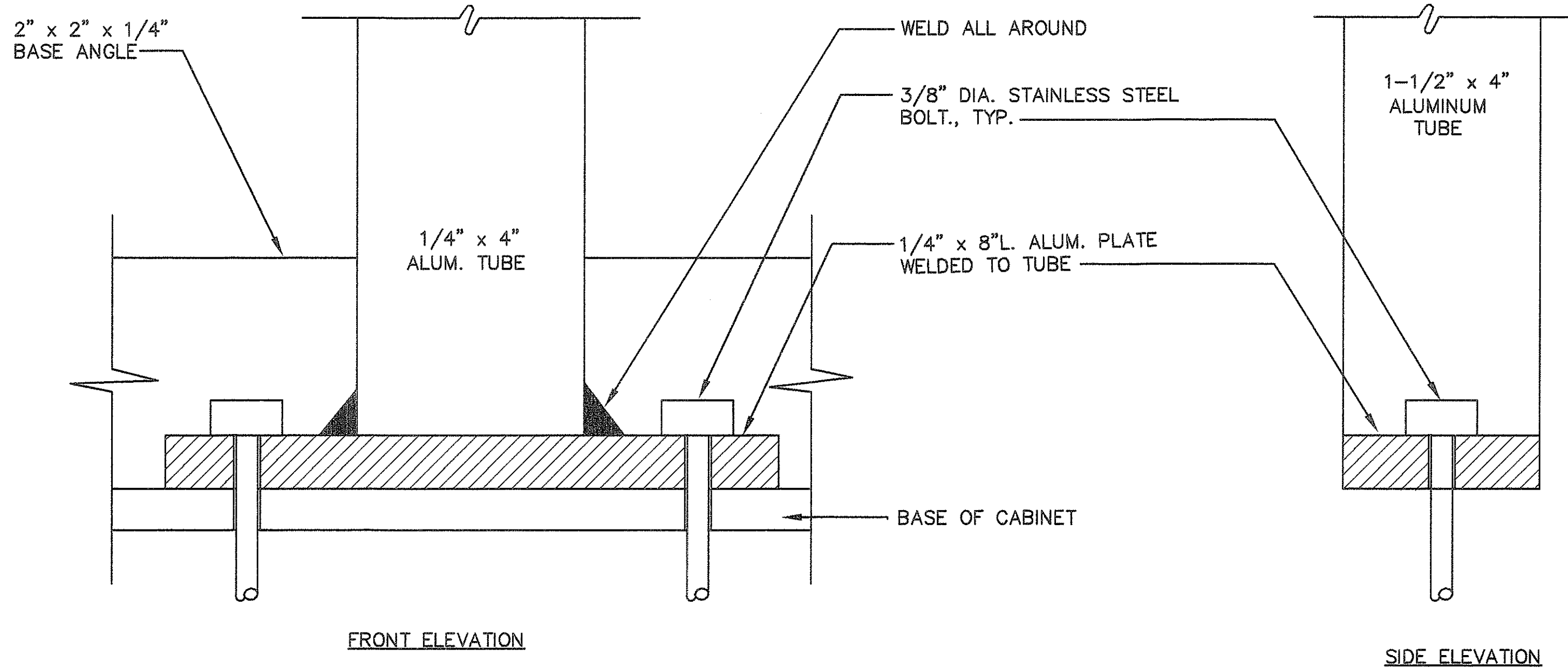
ALUMINUM TUBE BASE NOT TO SCALE
