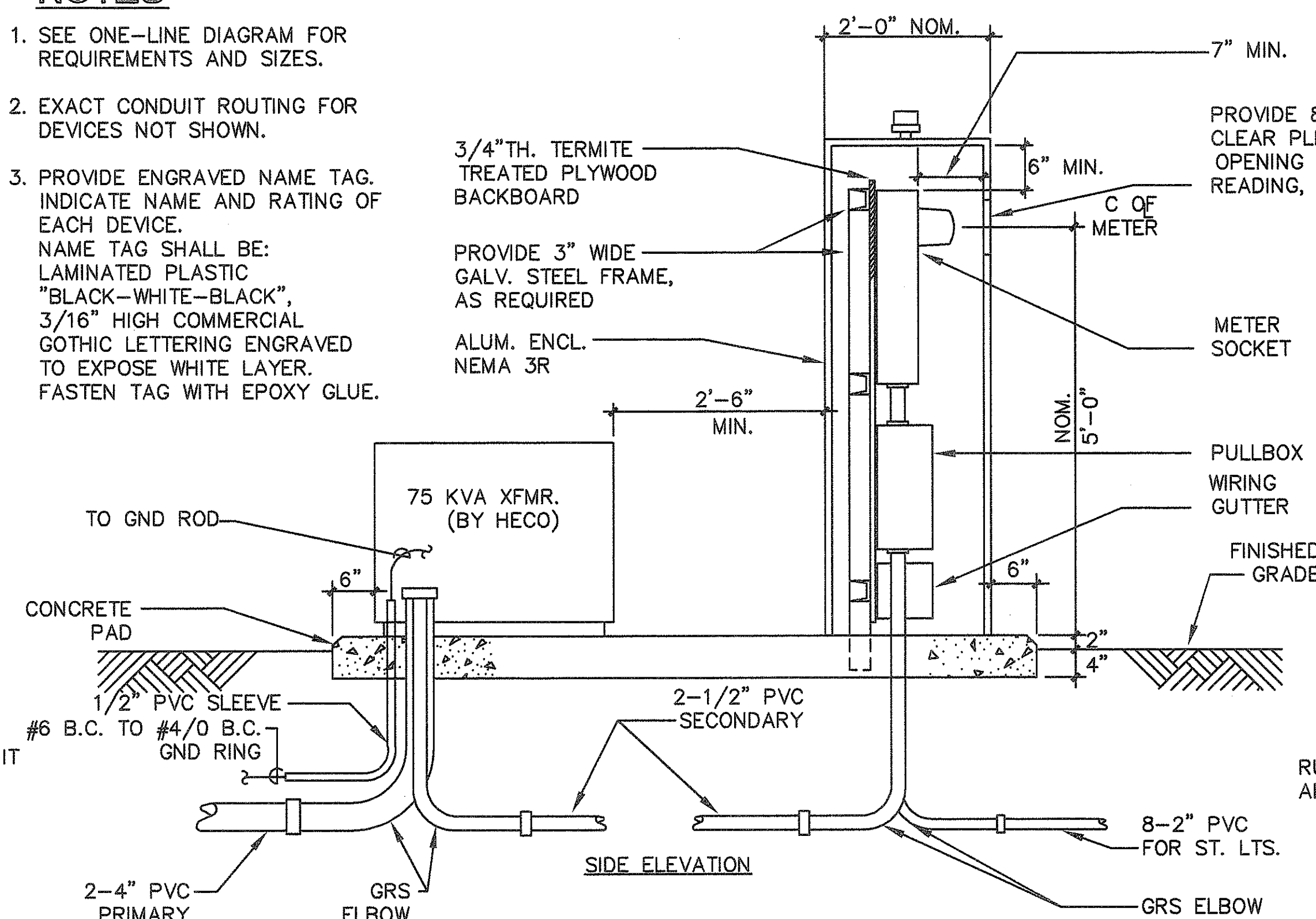
DISTRIBUTION CENTER "C" NOT TO SCALE
