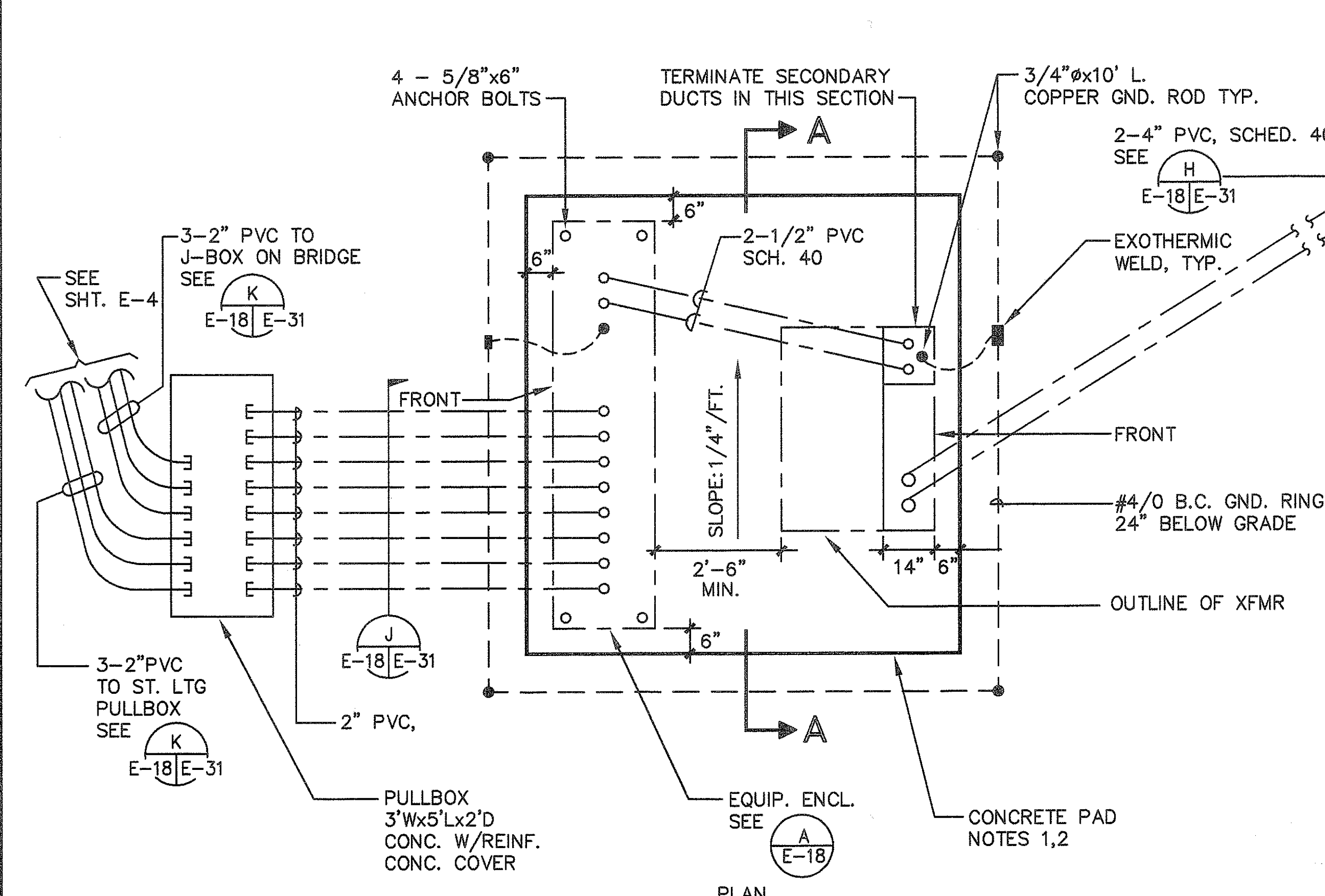
STREET LIGHT TRANS. & EQUIP. ENCL. NOT TO SCALE
