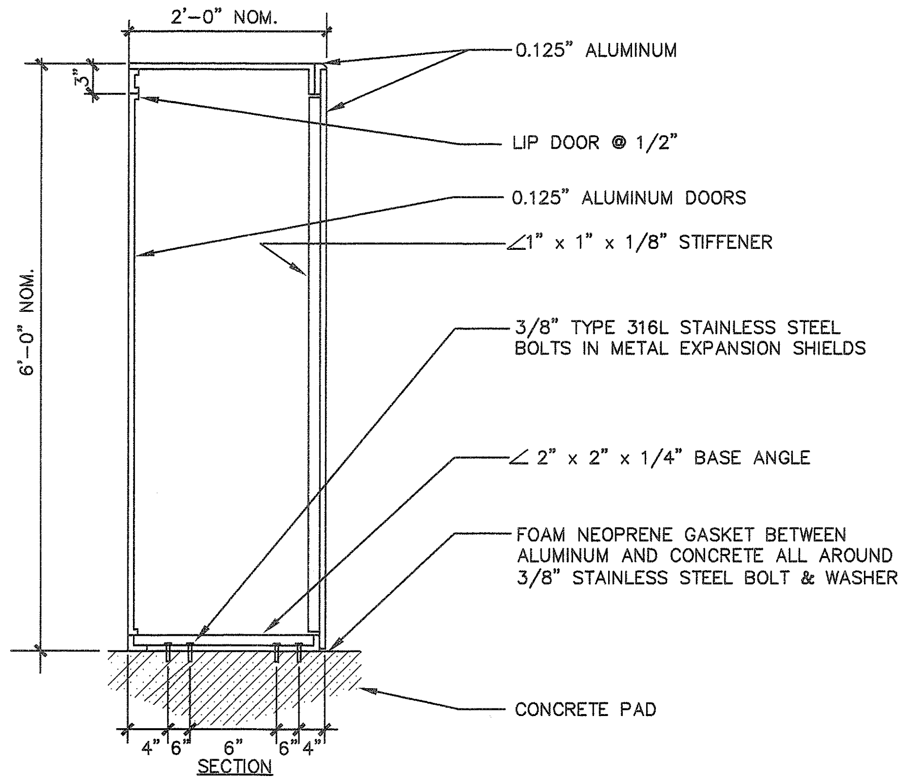
EQUIPMENT ENCLOSURE (DIST. CENTER "B") NOT TO SCALE
