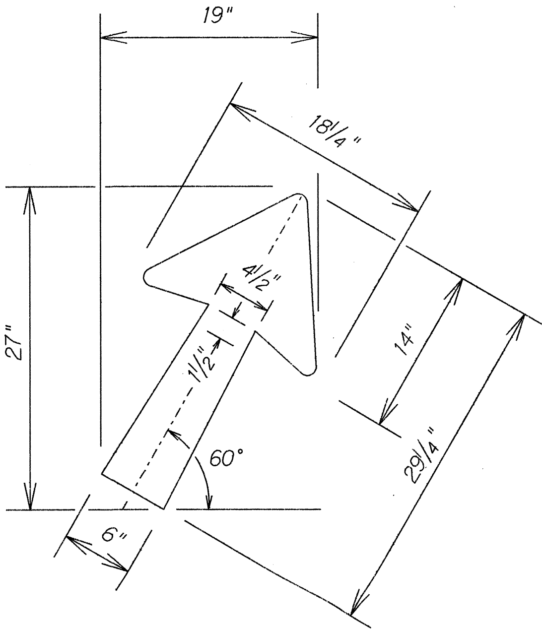
TYPE "A" DIAGONAL ARROW DETAIL
