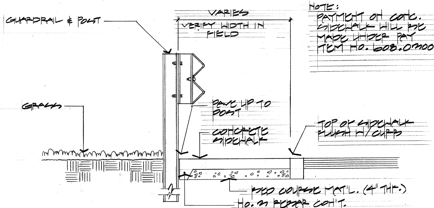
D CONCRETE SIDEWALK AT GUARDRAIL NO SCALE
