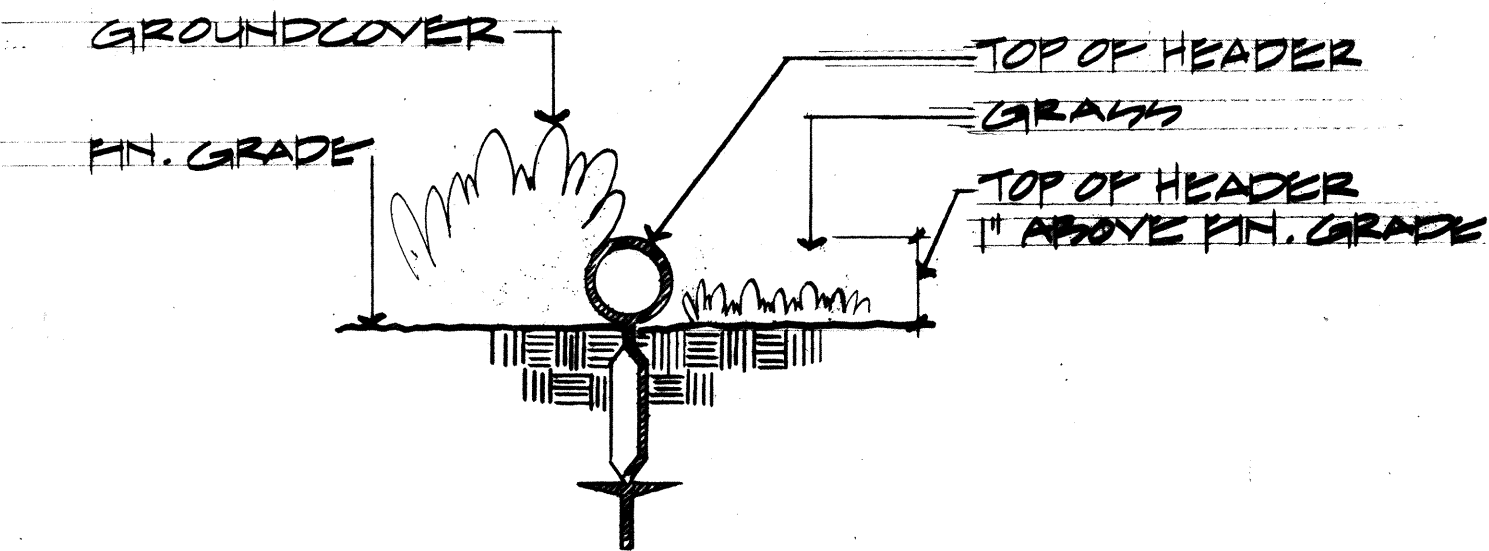
C PLASTIC HEADER DETAIL NO SCALE
