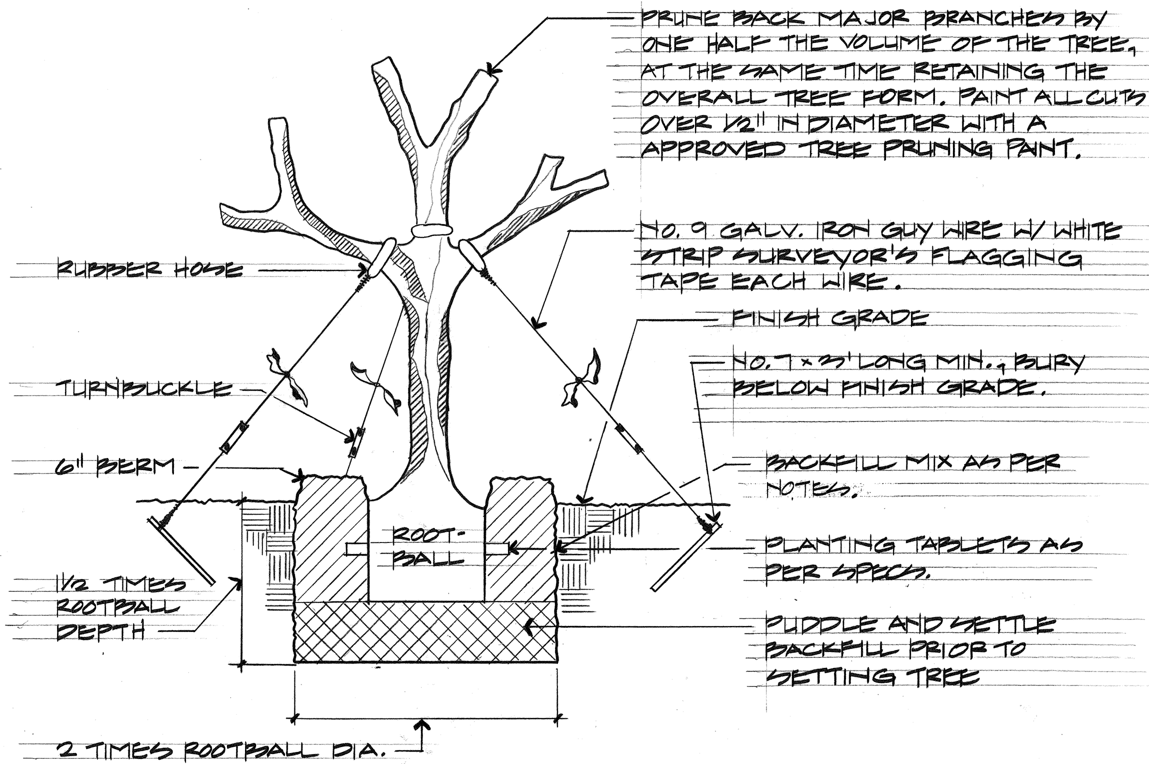
A TREE TRANSPLANTING DETAIL NO SCALE
