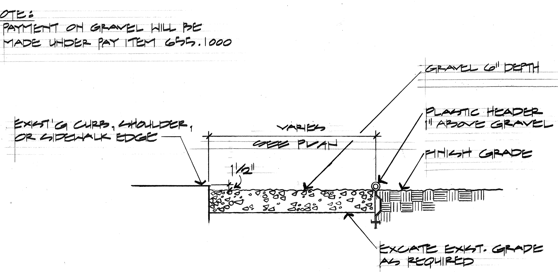
E TYPICAL GRAVEL STRIP NO SCALE
