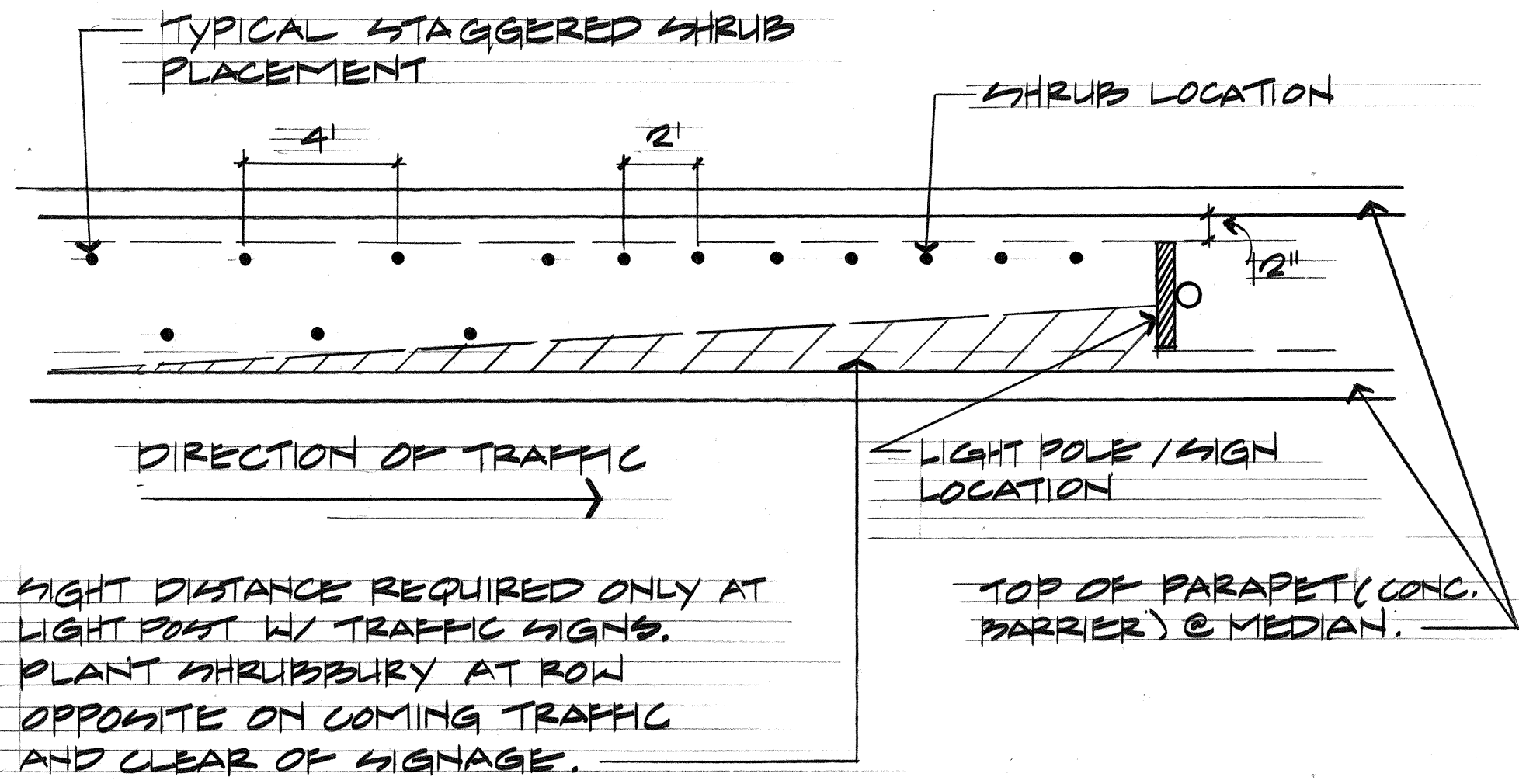
C MEDIAN PLANTING DETAIL NO SCALE
