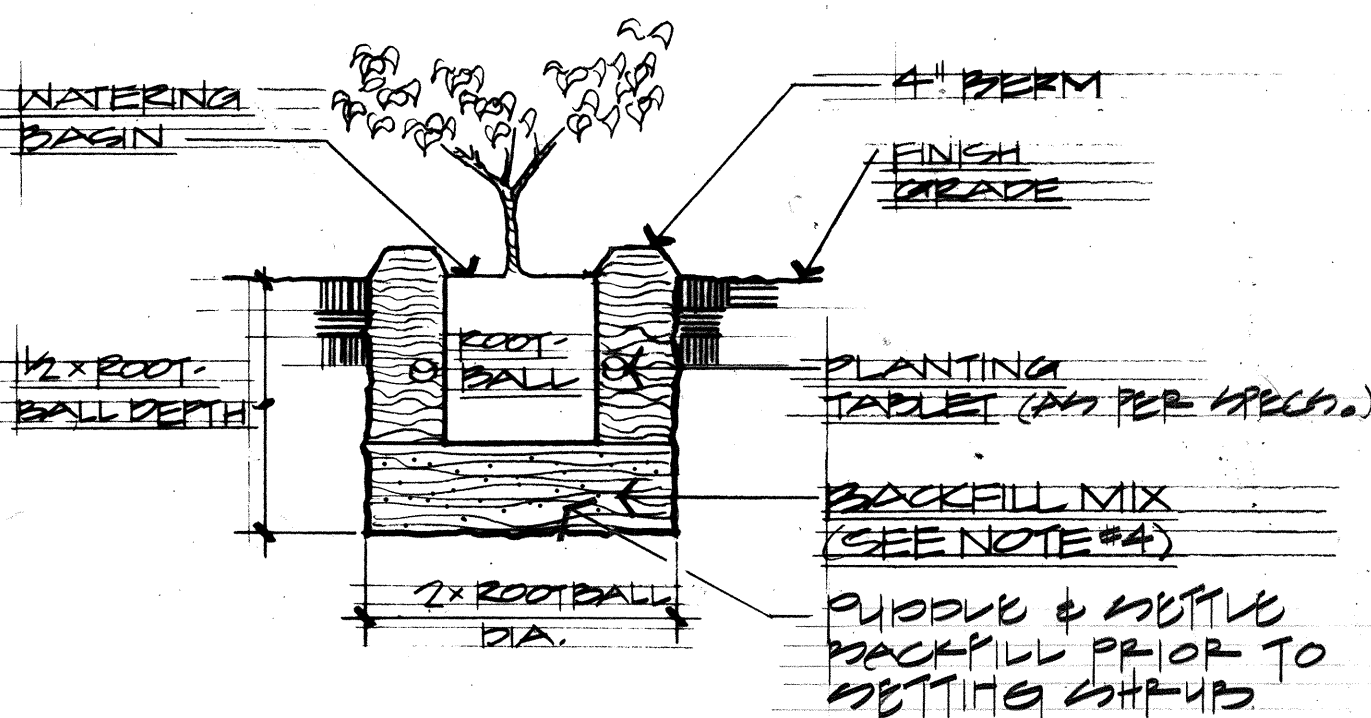
E SHRUB PLANTING DETAIL NO SCALE
