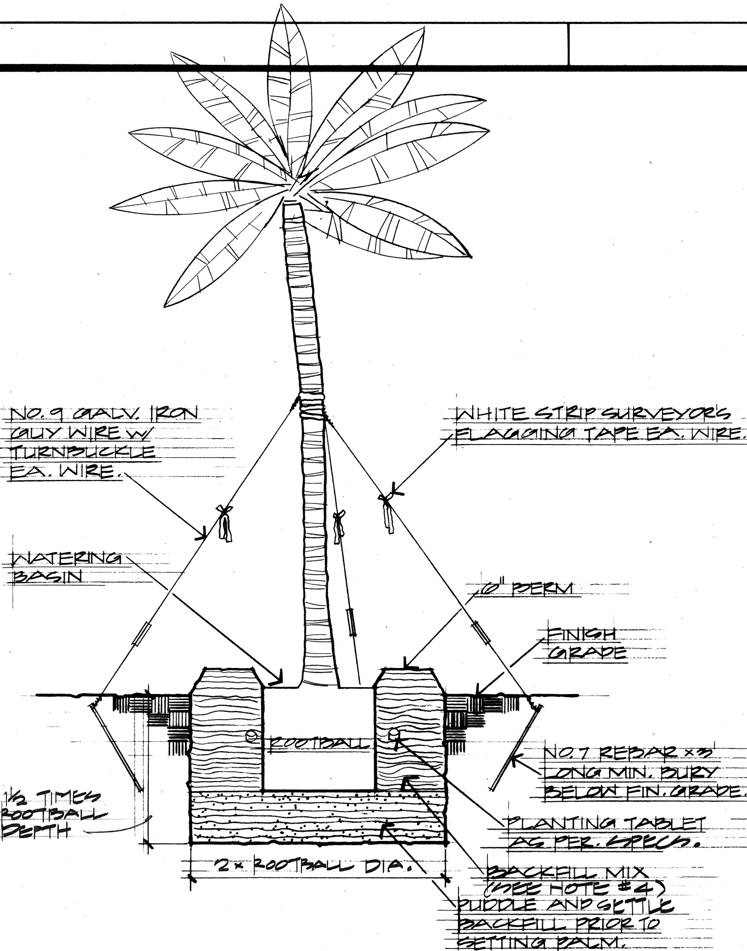
A PALM PLANTING DETAIL NO SCALE
