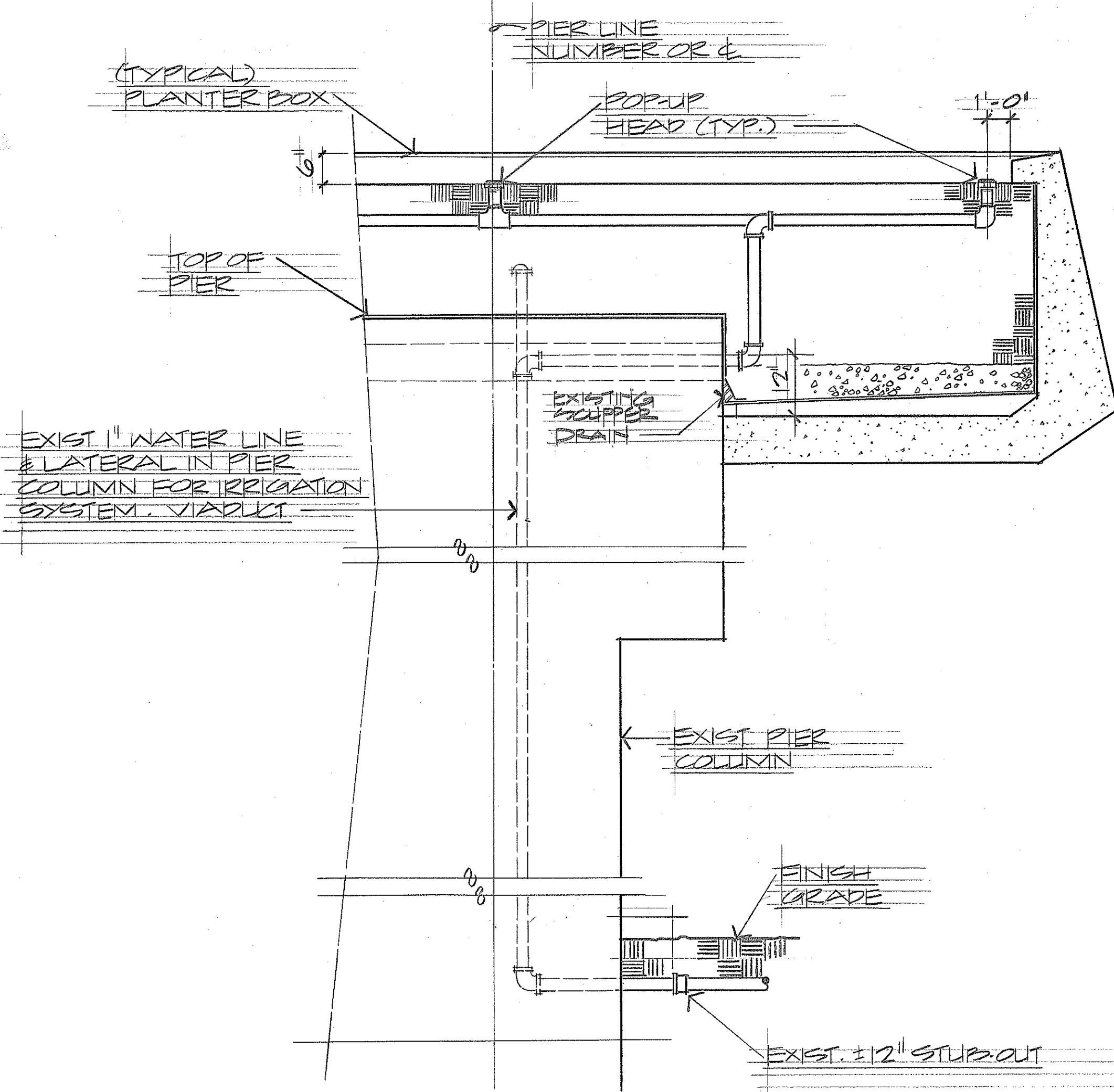
PLANTER BOX DETAIL NO SCALE
