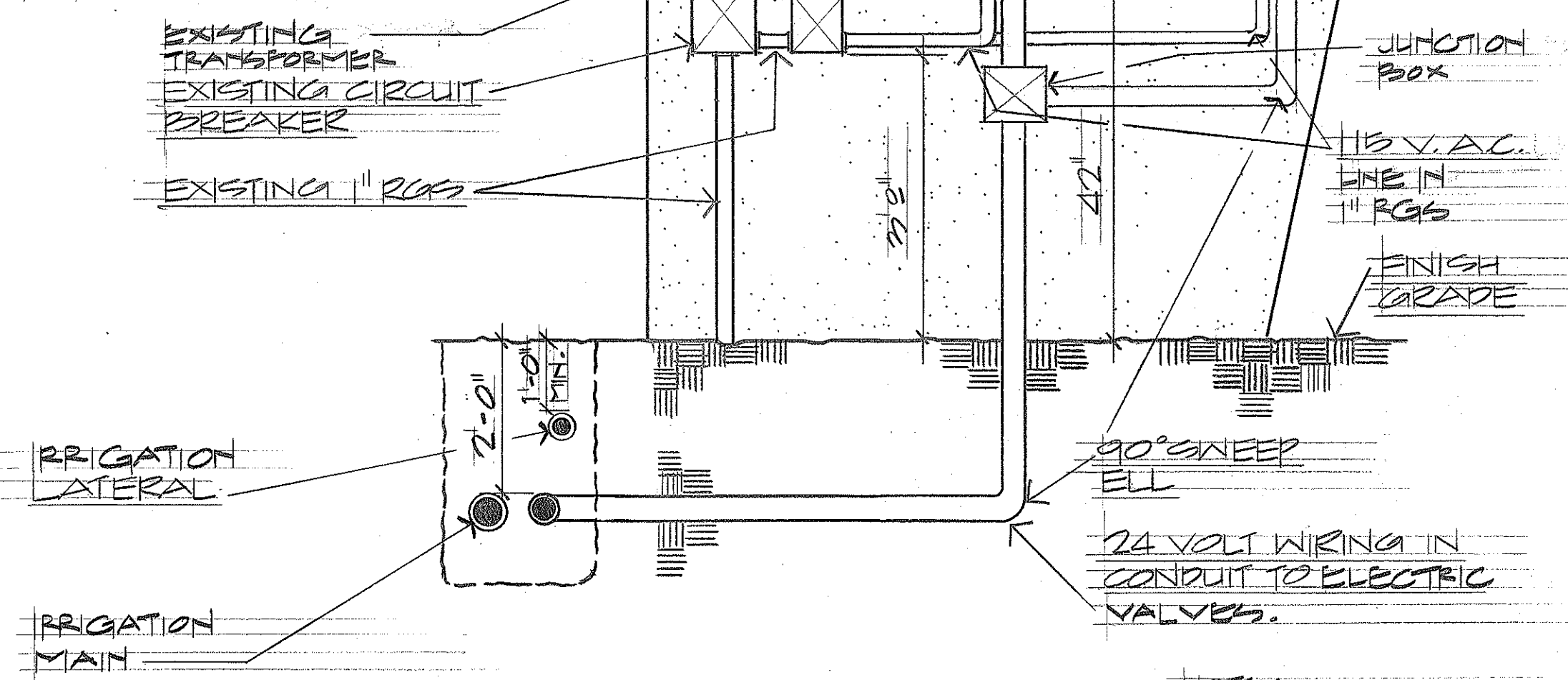
CONTROLLER DETAIL NO SCALE
