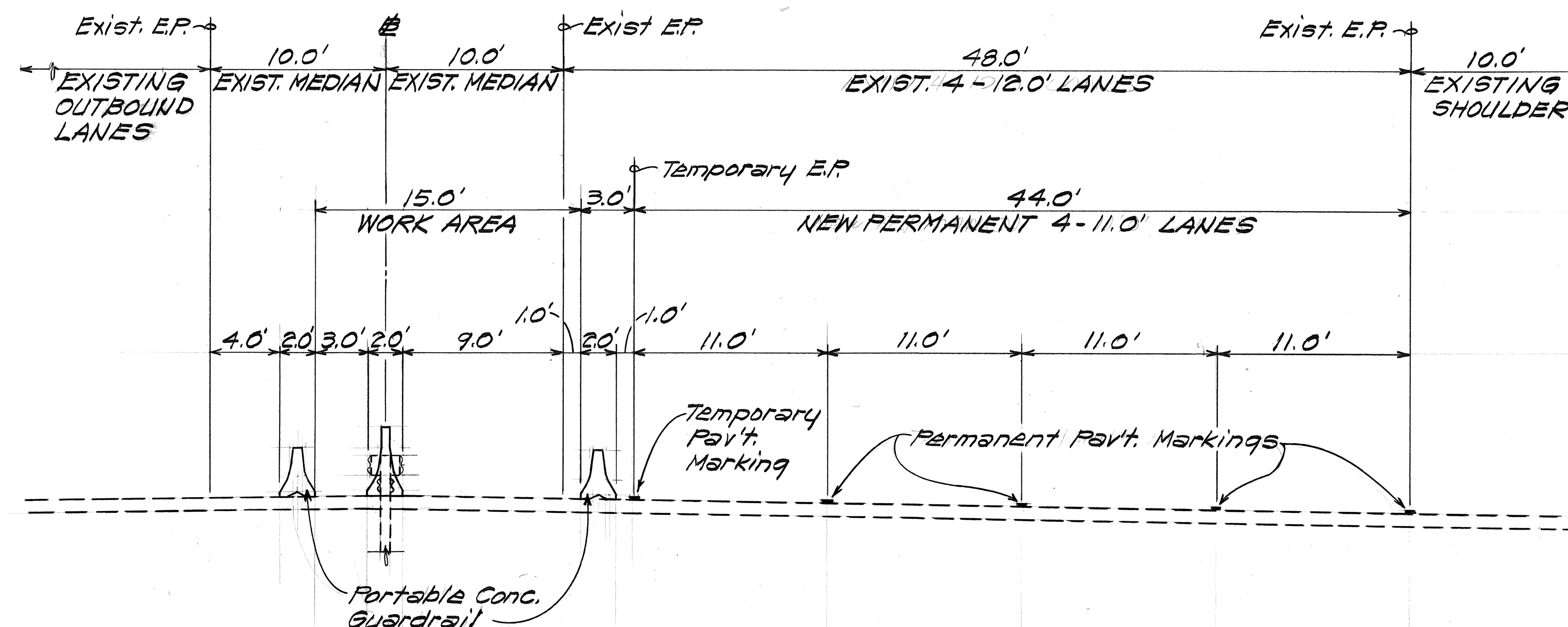
TYPICAL SECTION~ CONSTRUCTION PHASE III Scale: 3/16" = 1'-0"
