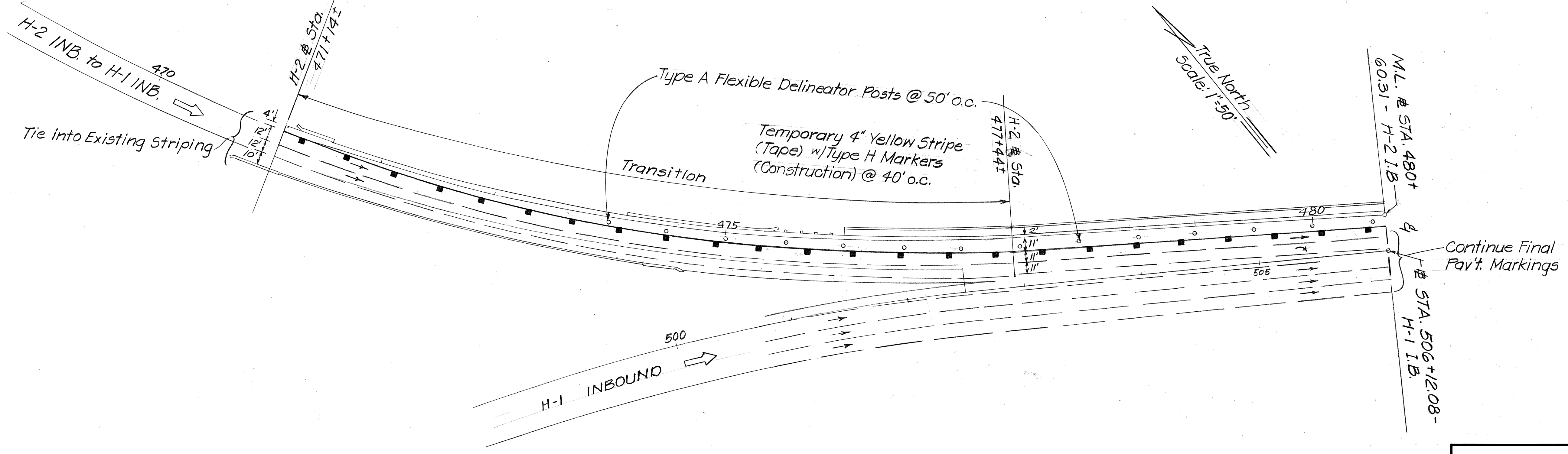
CONSTRUCTION PHASE III - TRAFFIC CONTROL
