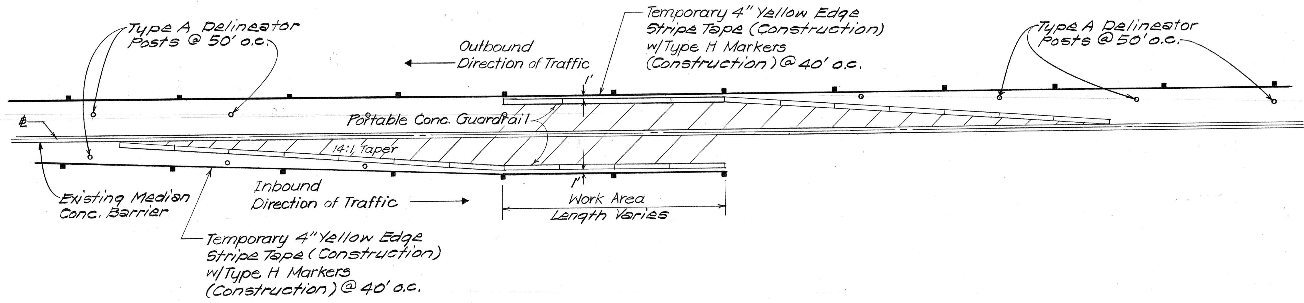
TYPICAL PORTABLE CONCRETE GUARDRAIL @ WORK AREA
