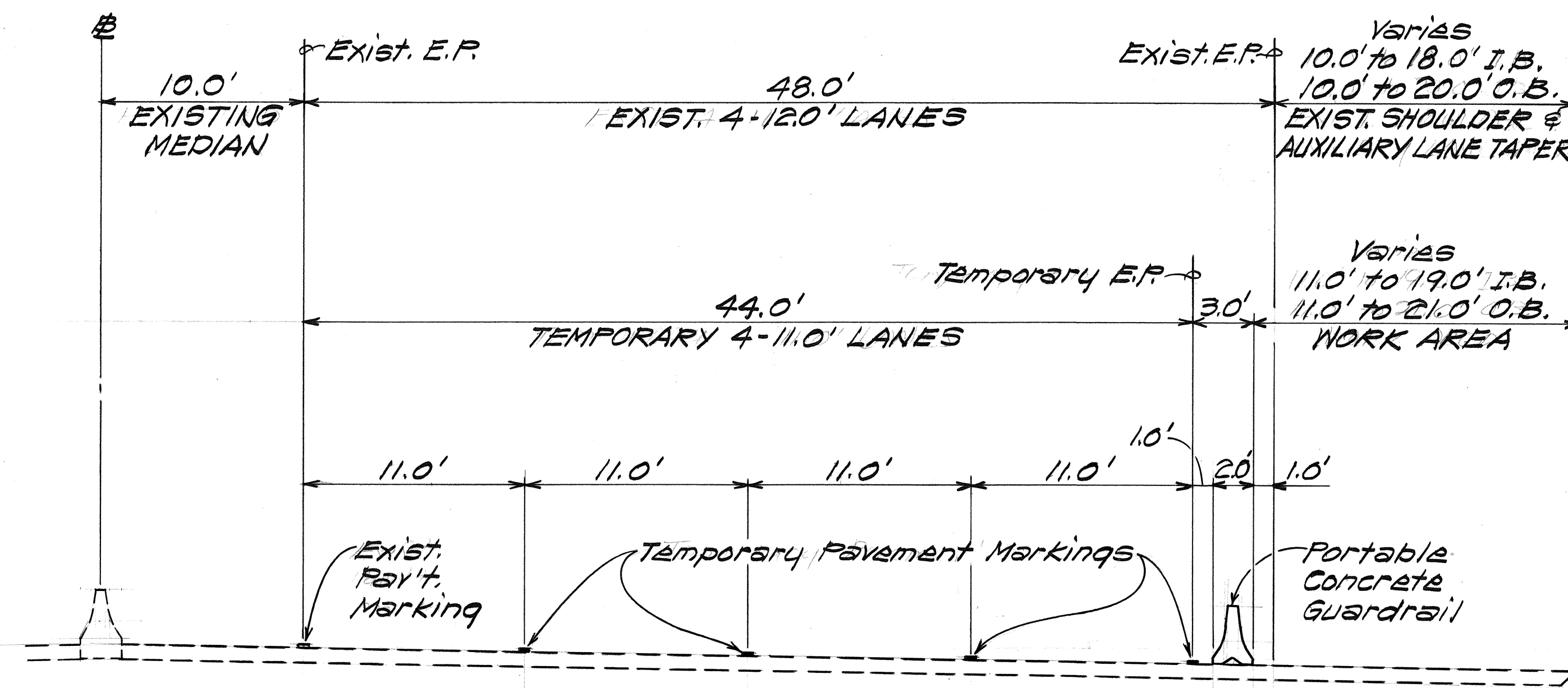
TYPICAL SECTION~ CONSTRUCTION PHASE I Scale: 3/16" = 1'-0"
