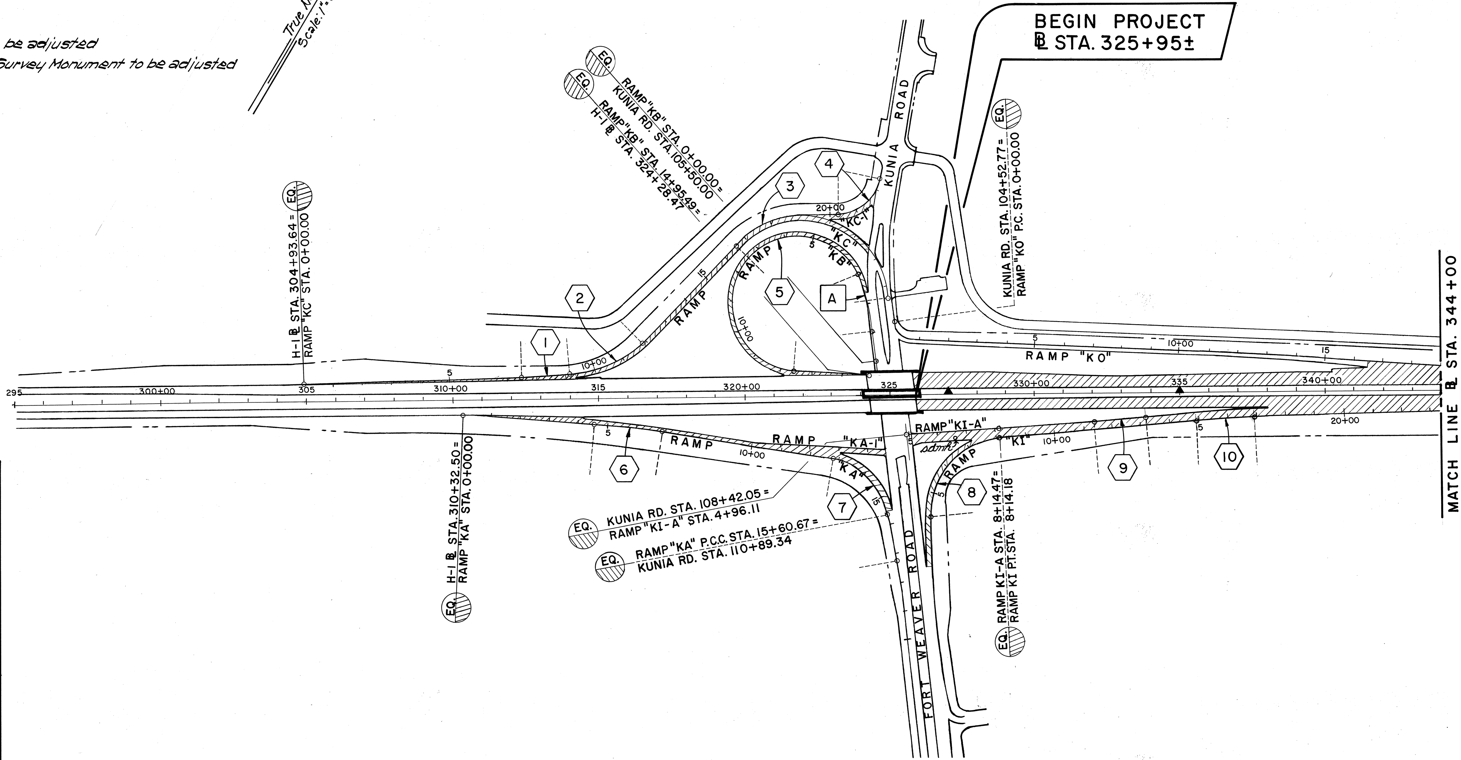
SCHEDULE ~ LOCATIONS FOR ADJUSTING CENTERLINE AND REFERENCE SURVEY MONUMENT
