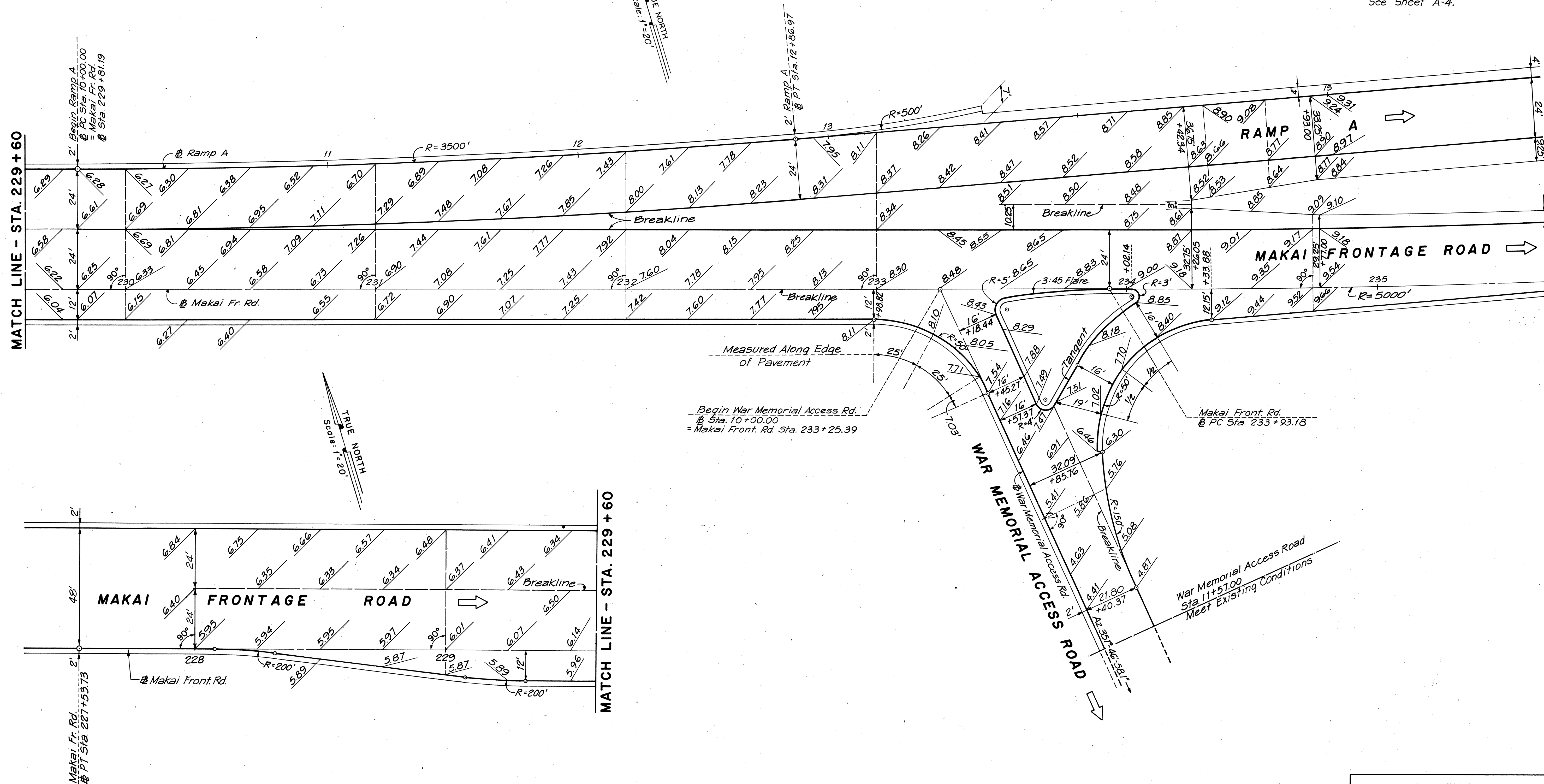
RAMP A & MAKAI FRONTAGE ROAD and WAR MEMORIAL ACCESS ROAD SCALE: 1" = 20'
