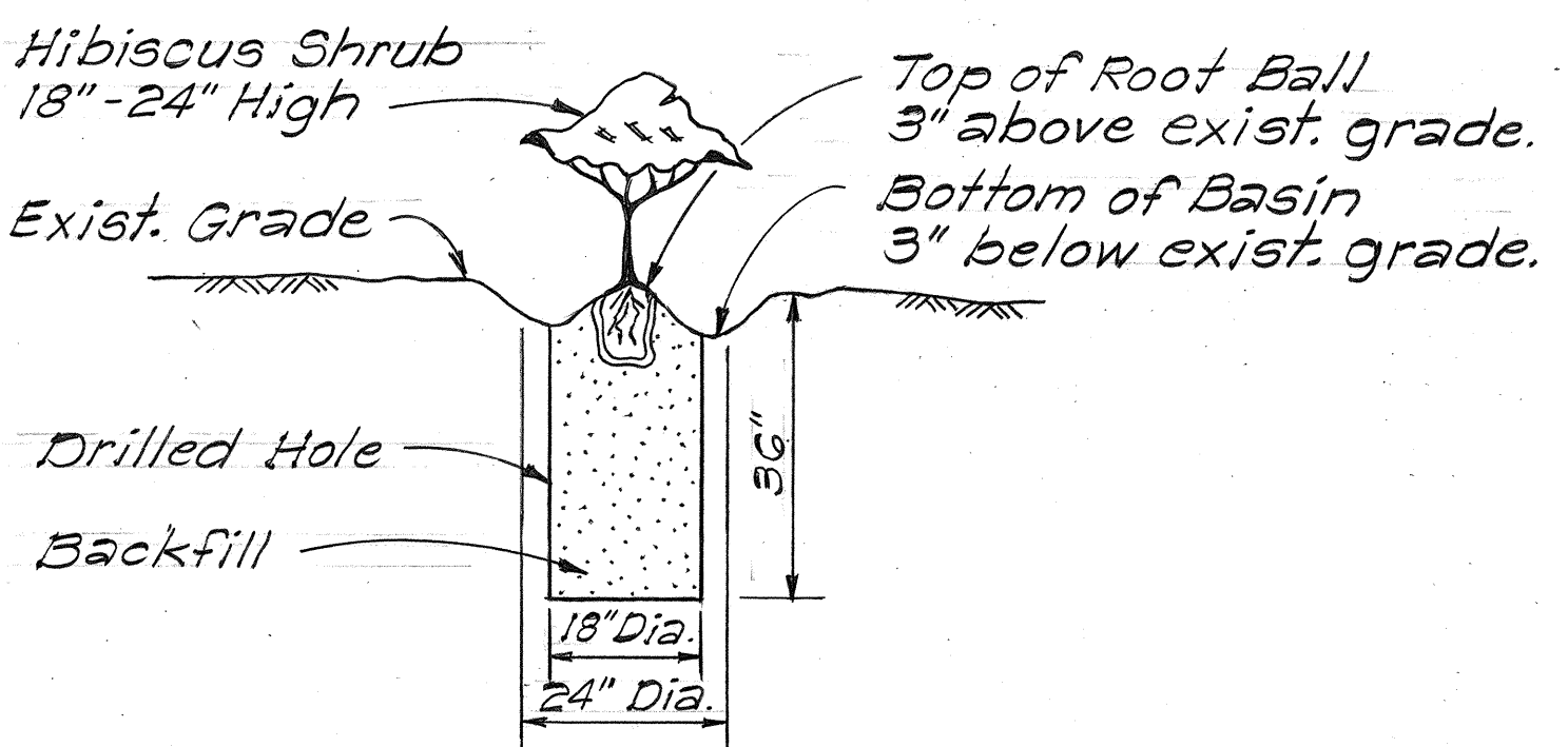
SECTION ROUND BASIN Scale: 1/2" = 1'-0"
