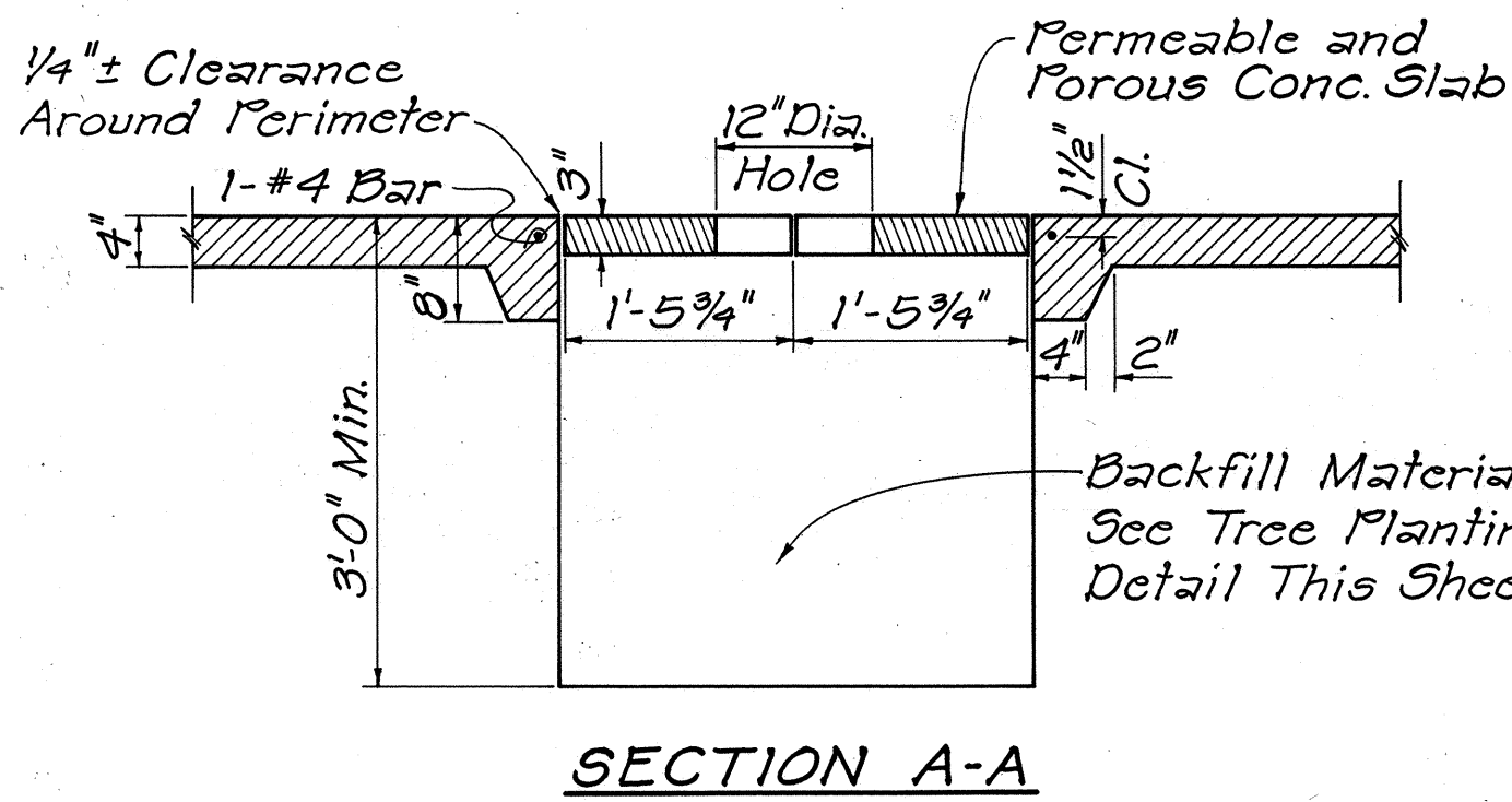
TREE WELL WITH CONCRETE COVER Scale: 3/4" = 1'-0"
