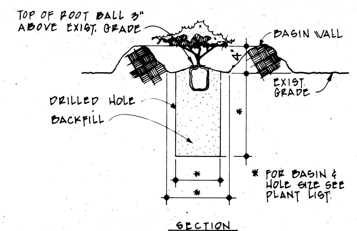
SECTION ROUND BASIN FOR PLANTS WHERE BUBBLE HEAD IS TO BE INSTALLED
