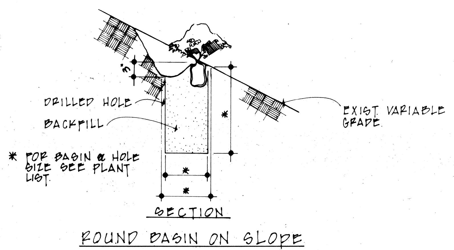
SECTION ROUND BASIN NO SCALE
