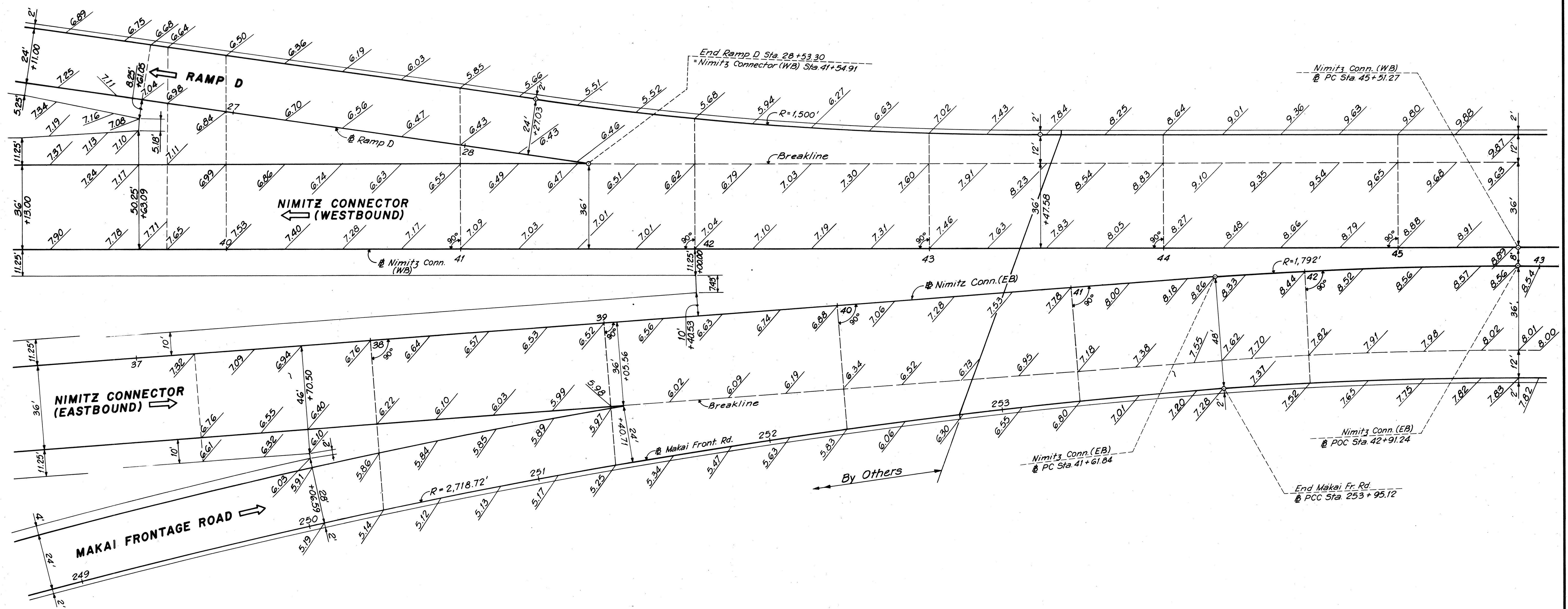
RAMP D & NIMITZ CONNECTOR (WB) and NIMITZ CONNECTOR (EB) & MAKAI FRONTAGE ROAD SCALE: 1"=20'
