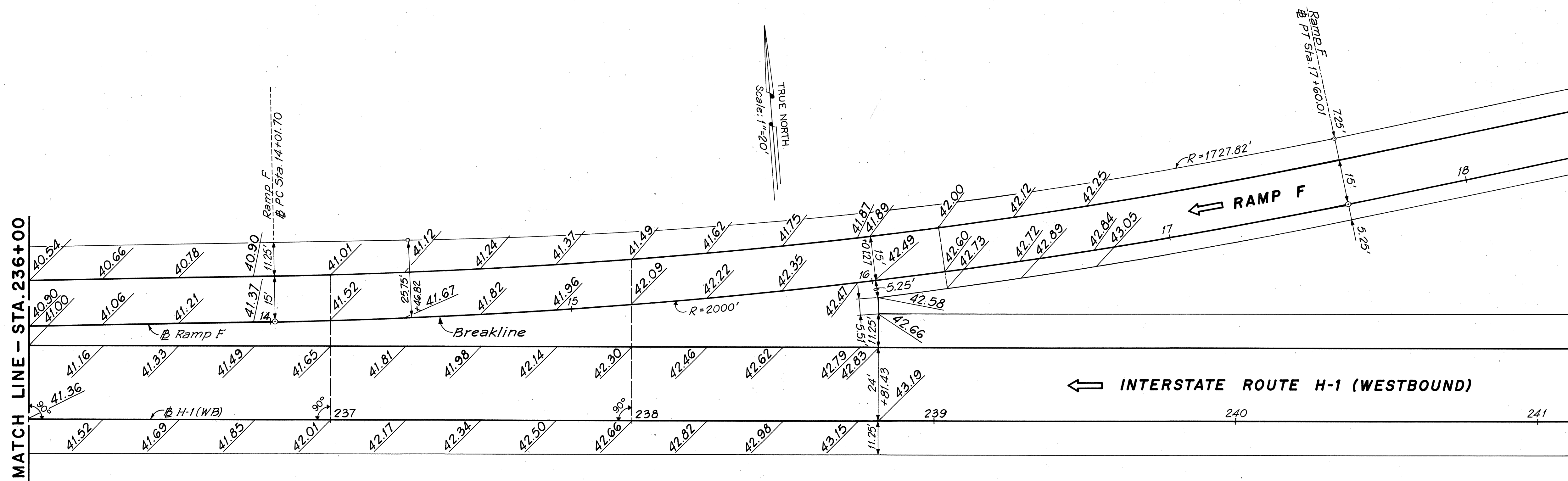
RAMP F & INTERSTATE ROUTE H-1 (WB) SCALE: 1" = 20'
