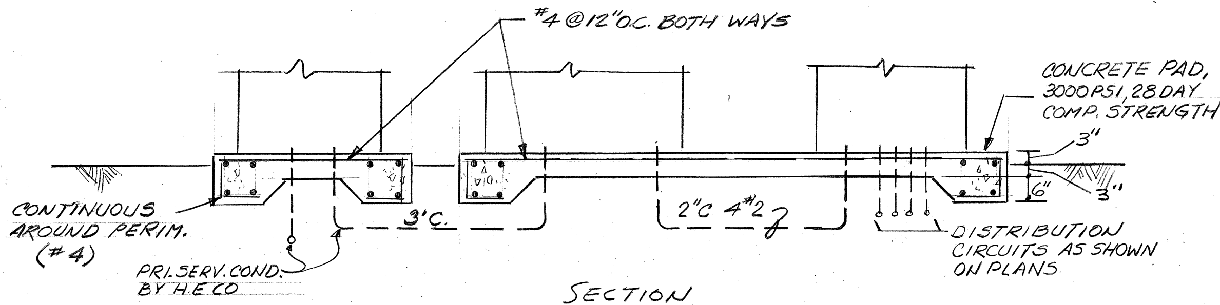
SECTION
