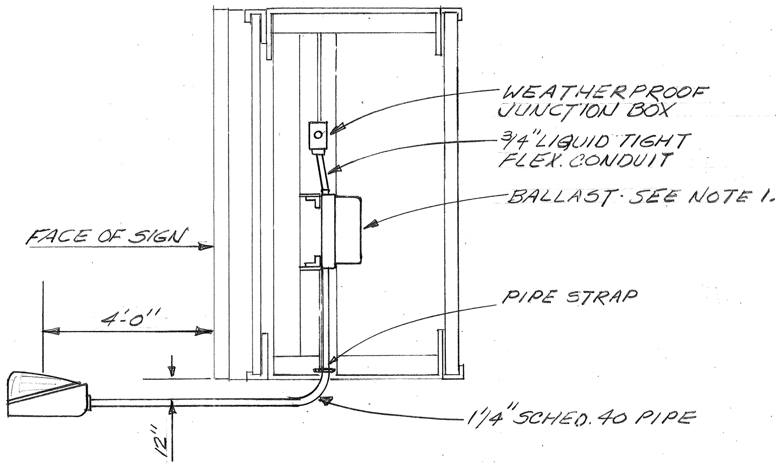
LUMINAIRE MOUNTING NOT TO SCALE
