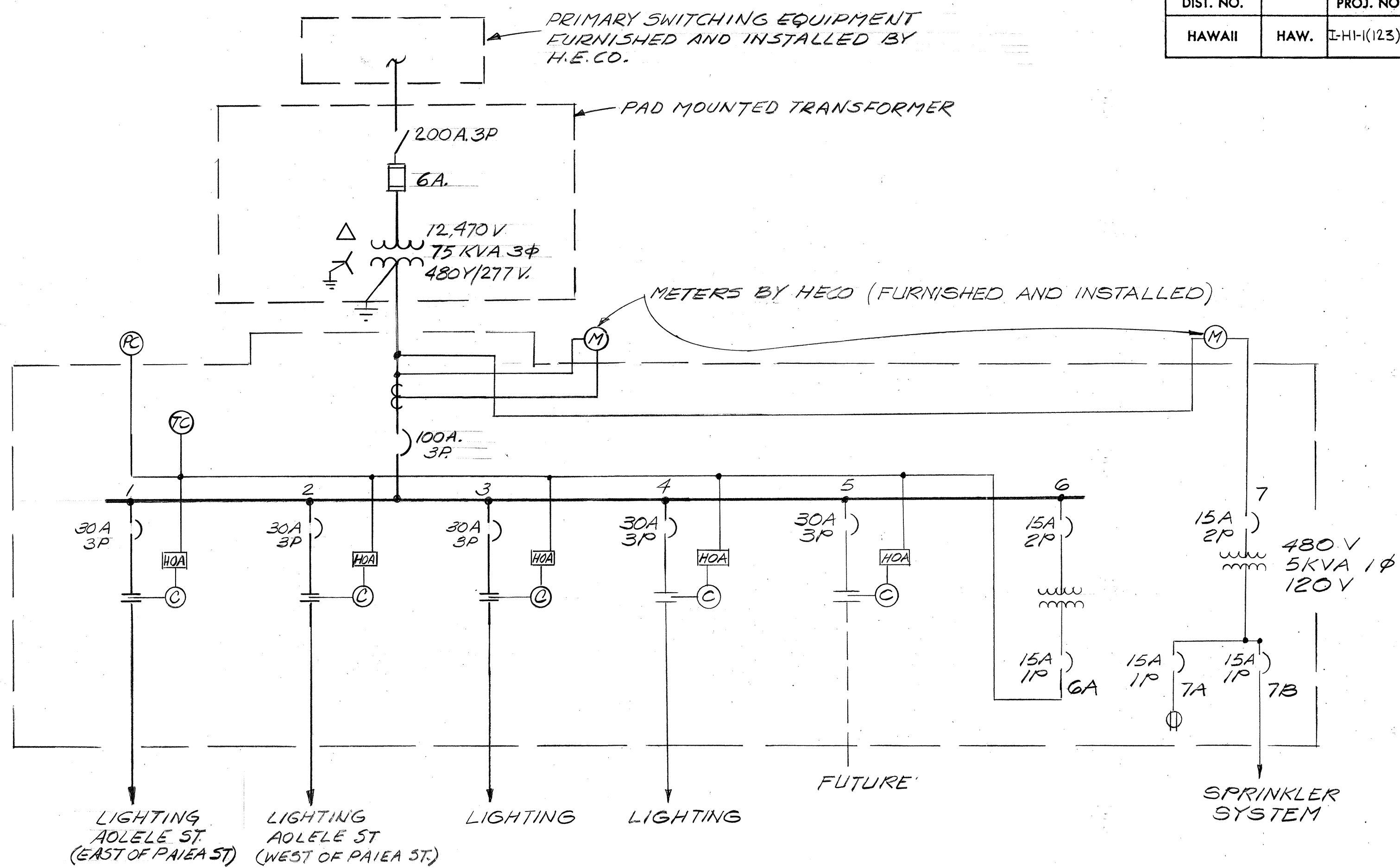
SUBSTATION SS4 SINGLE LINE DIAGRAM N.T.S.
