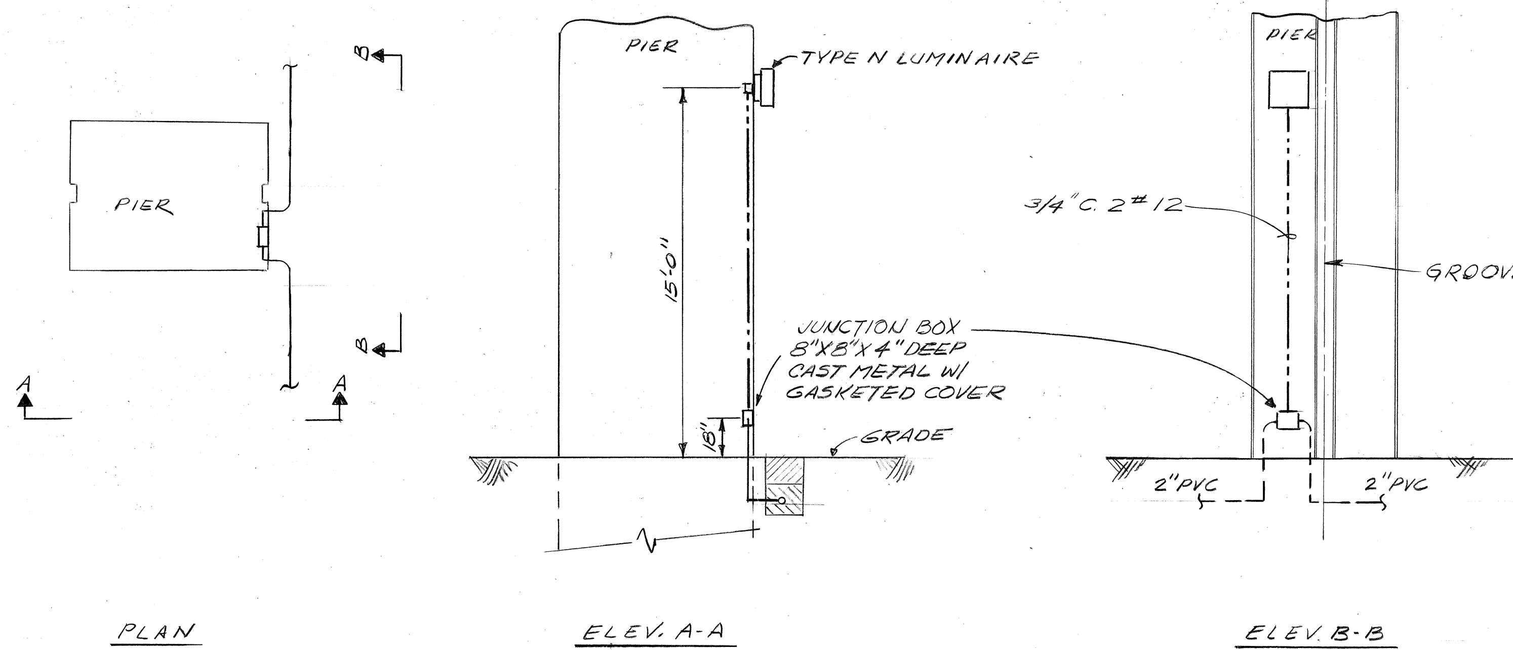
TYPE N FIXTURE MOUNTING DETAIL (1) 1/4" = 1'-0"
