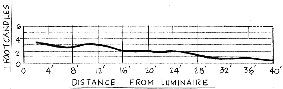
HORIZONTAL FOOTCANDLES ON PAVEMENT FIXTURE WITH 430 MA BALLAST CONTINUOUS ROW ON ONE SIDE
