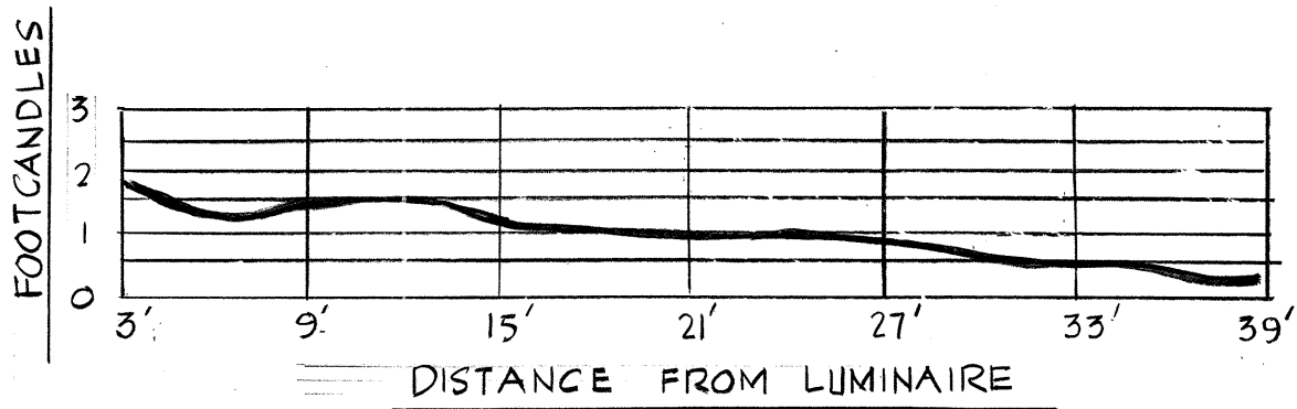
HORIZONTAL FOOTCANDLES ON PAVEMENT FIXTURES WITH 200MA BALLAST CONTINUOUS ROW ON ONE SIDE
