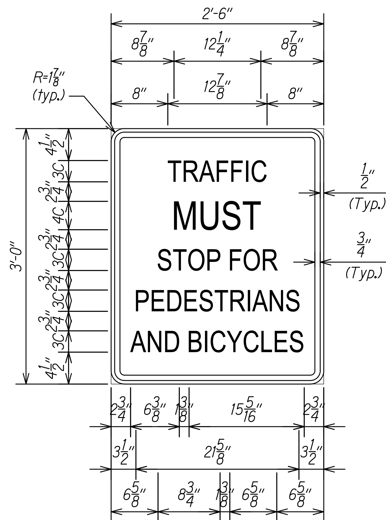
TRAFFIC MUST STOP SIGN (Black on White) Not To Scale
