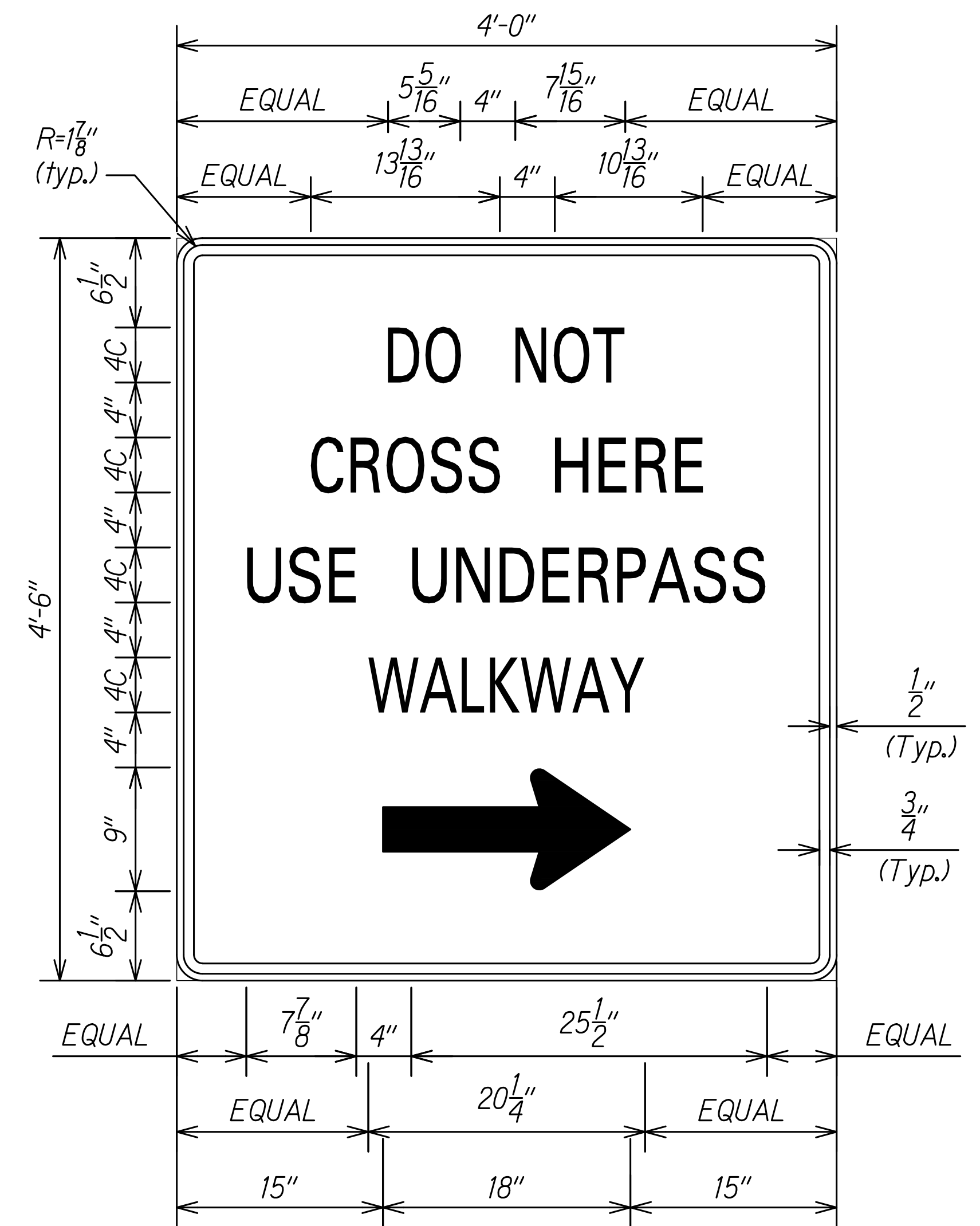
DO NOT CROSS SIGN (Black on White) Not To Scale
