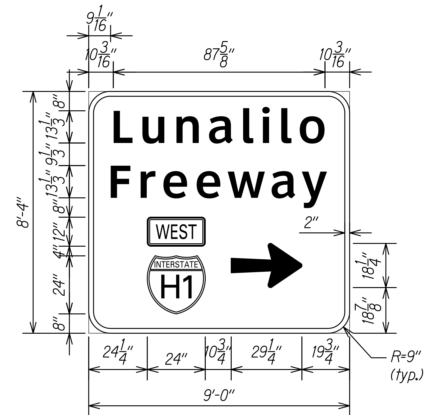
D-4 Not To Scale
