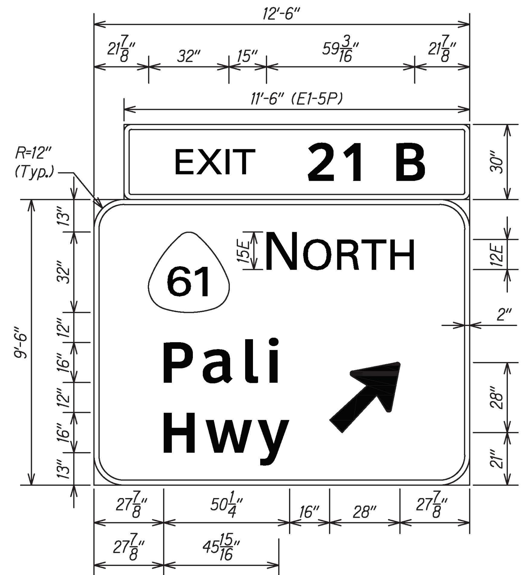
E-1 (White on Green) Scale: 1/2" = 1'-0"
