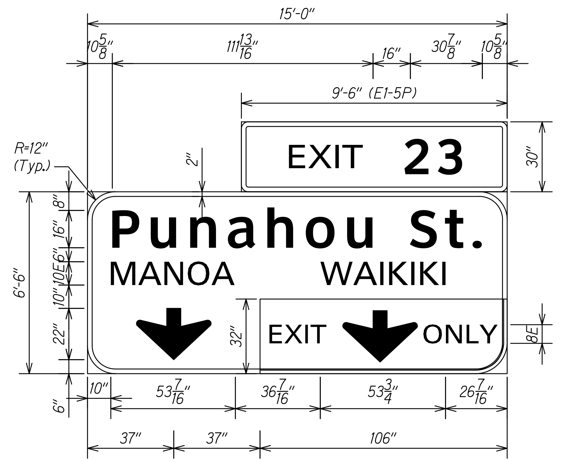
E-6 (White on Green) Scale: 1/2" = 1'-0"
