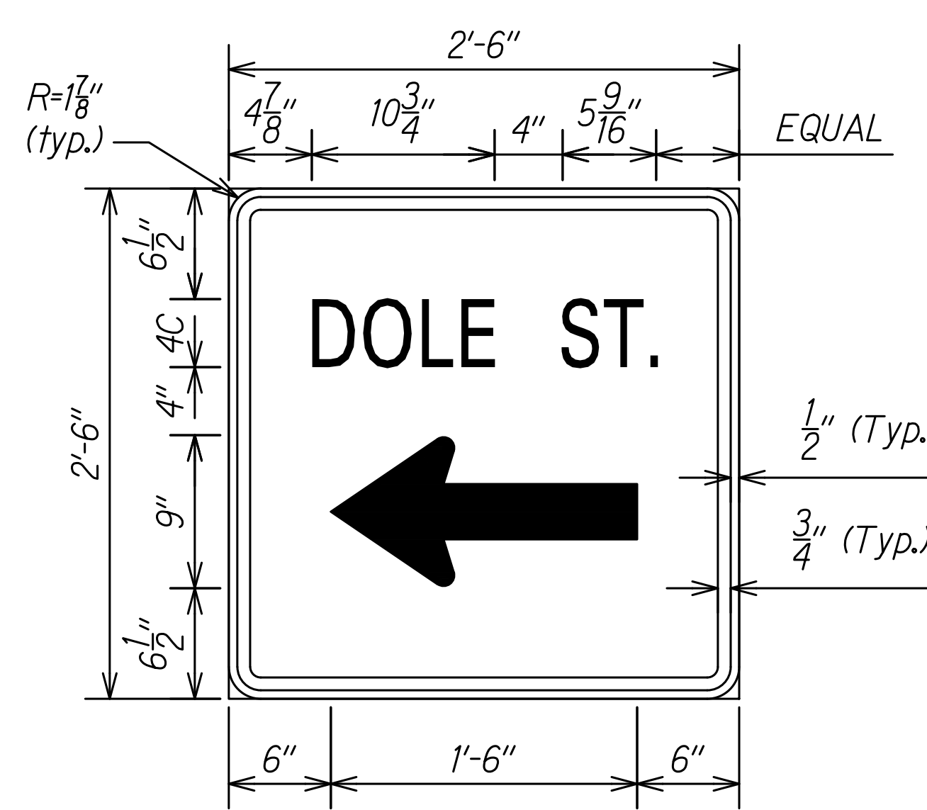
DIRECTIONAL SIGN (Black on White) Not To Scale
