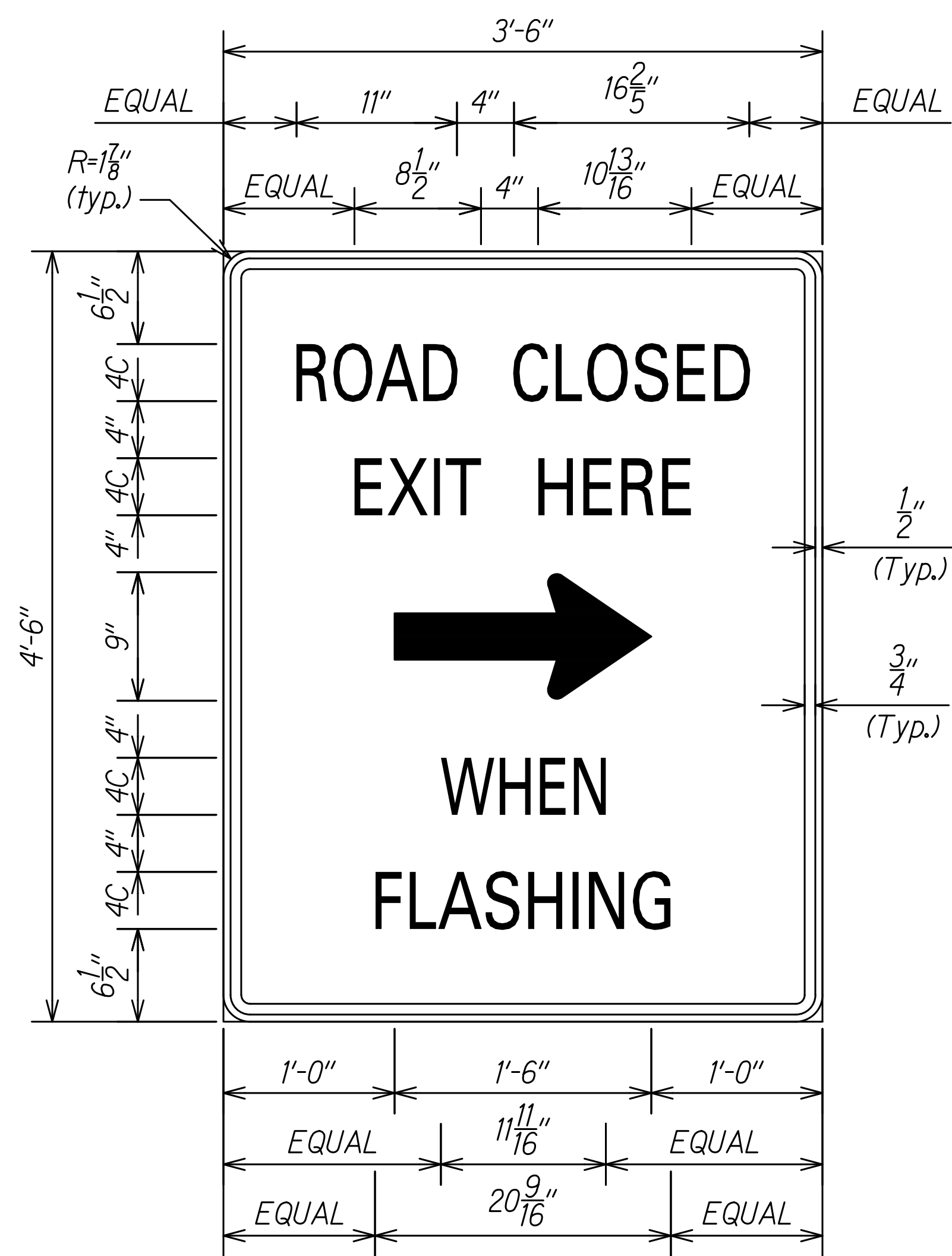
ROAD CLOSED SIGN (Black on Orange) Not To Scale
