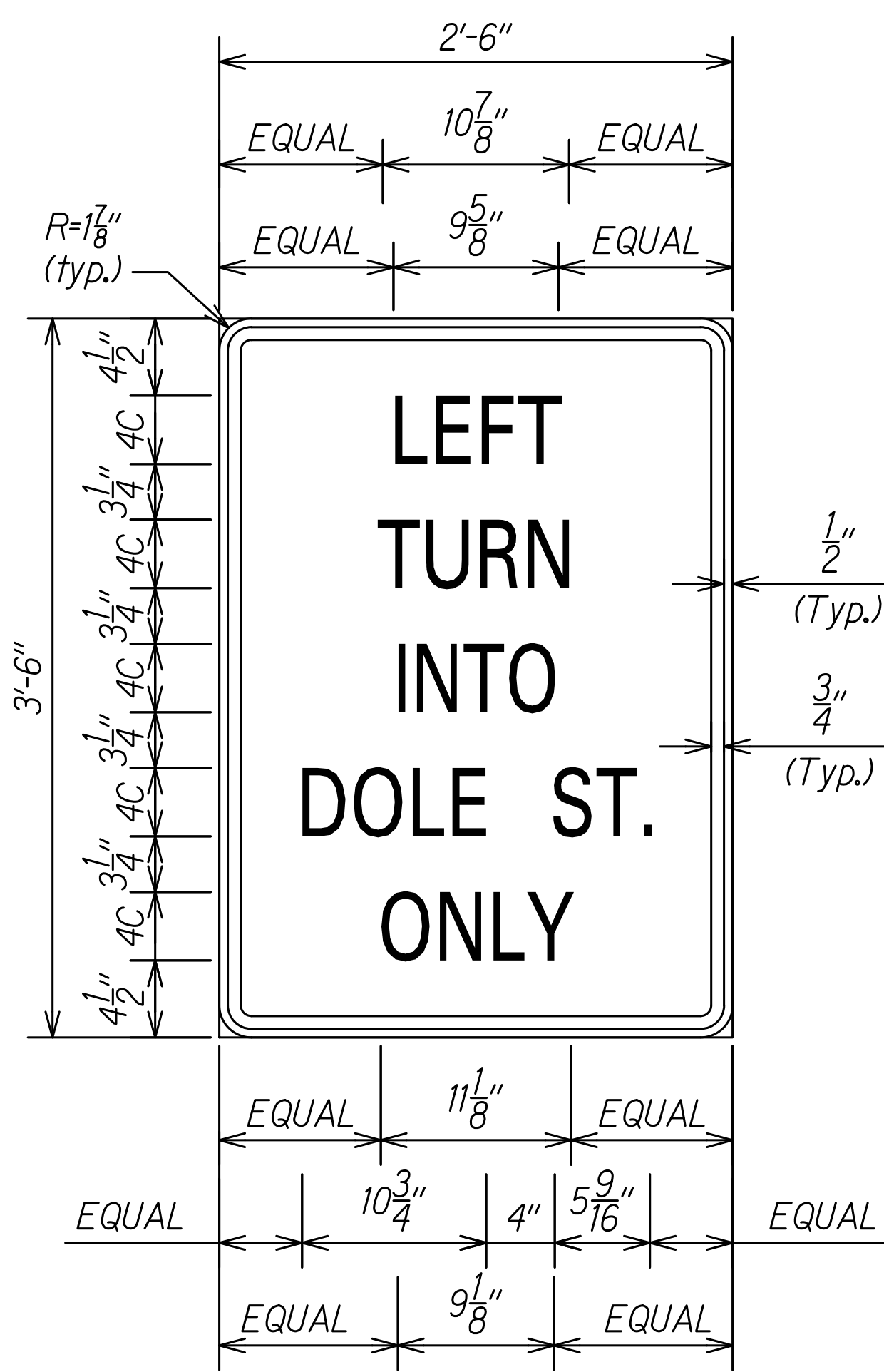
LEFT TURN SIGN (Black on White) Not To Scale
