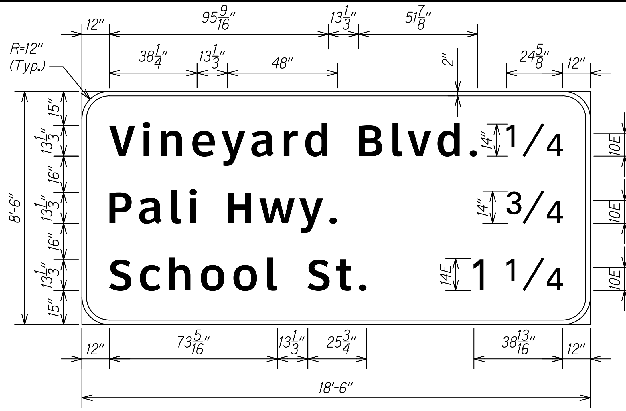
E-5 (White on Green) Scale: 1/2" = 1'-0"
