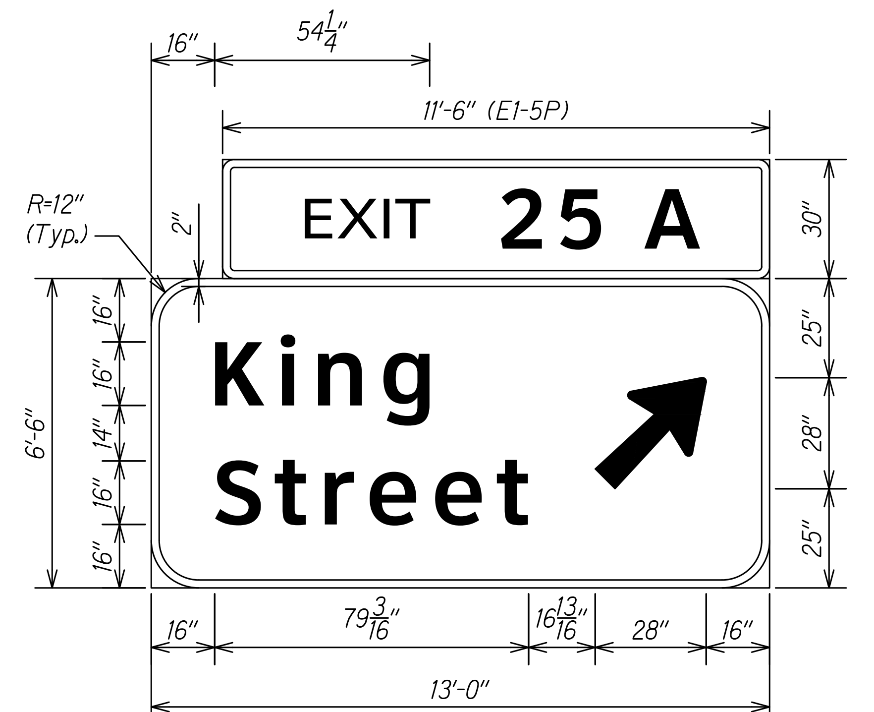
E-19 (White on Green) Scale: 1/2" = 1'-0"
