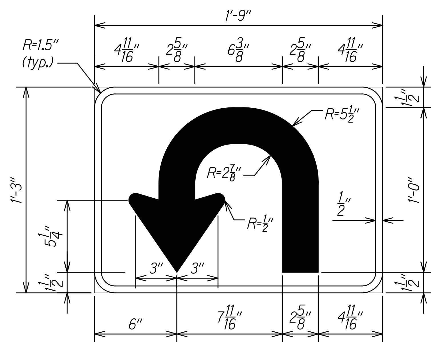
U-TURN ARROW SIGN Not To Scale
