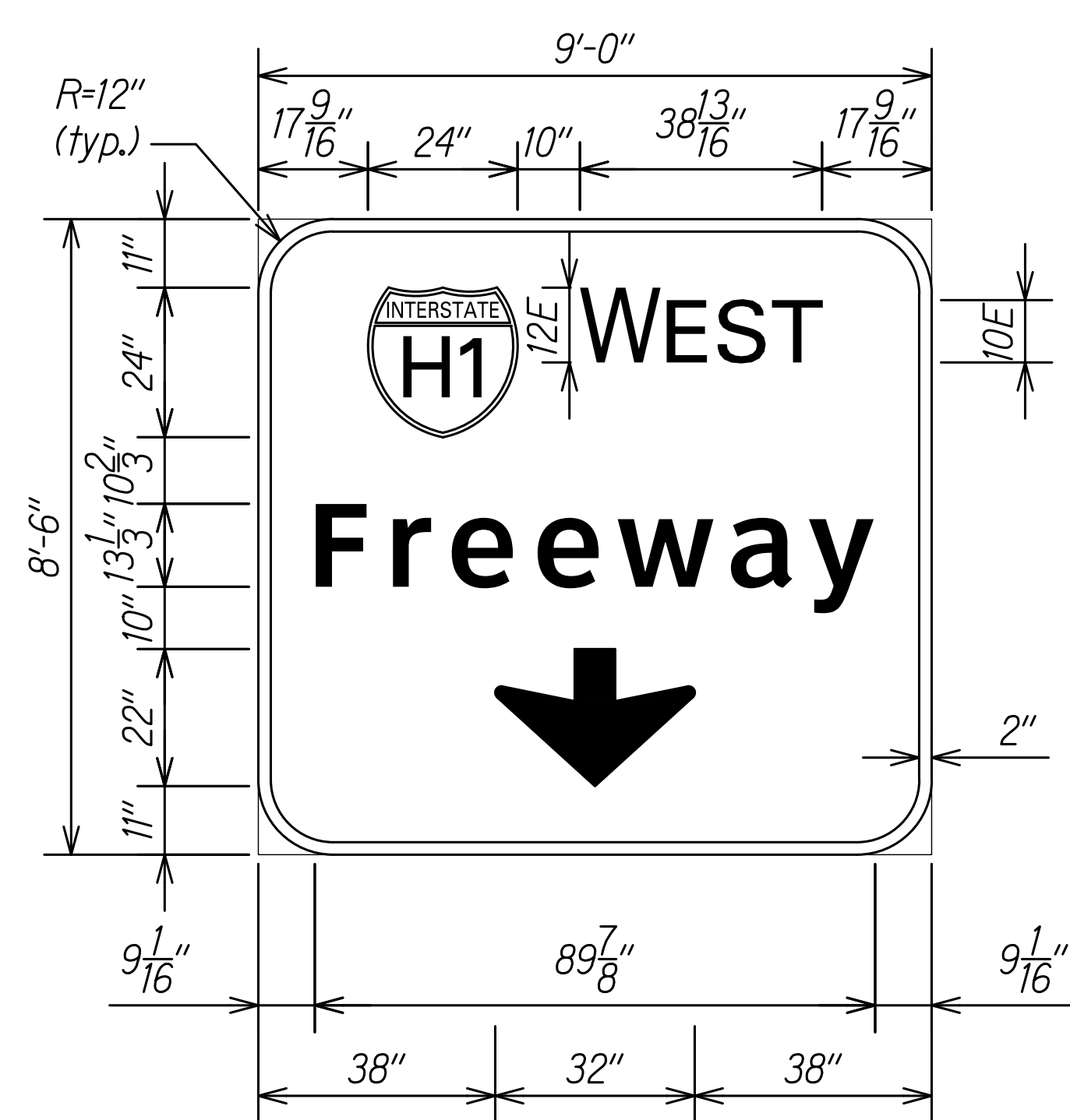
D-3 (R) Not To Scale
