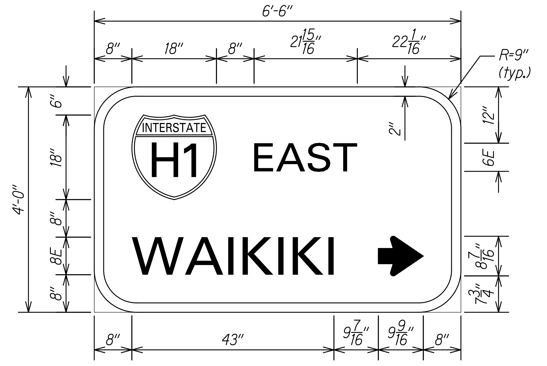
D-8 Not To Scale
