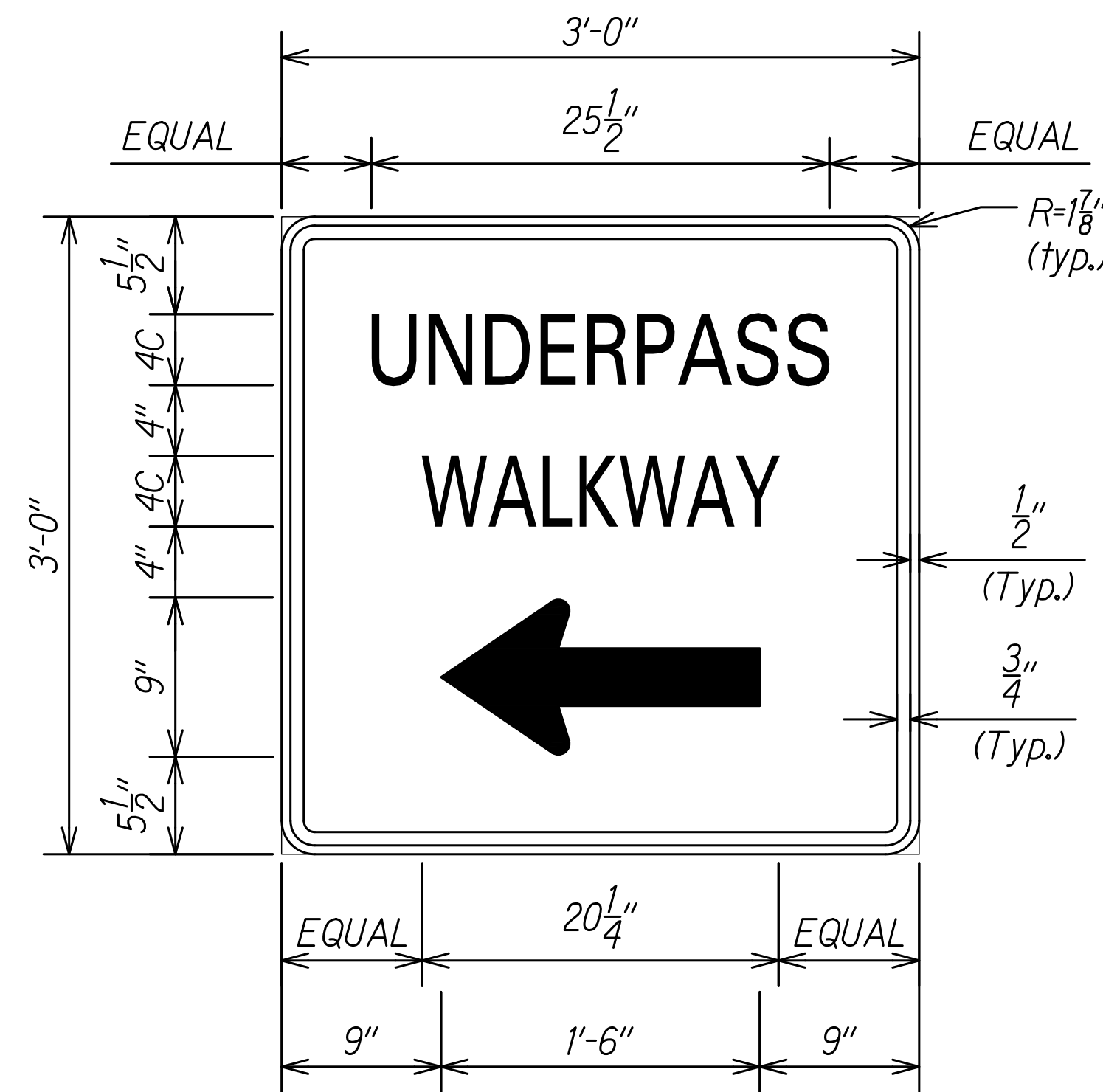
UNDERPASS WALKWAY SIGN (Black on White) Not To Scale
