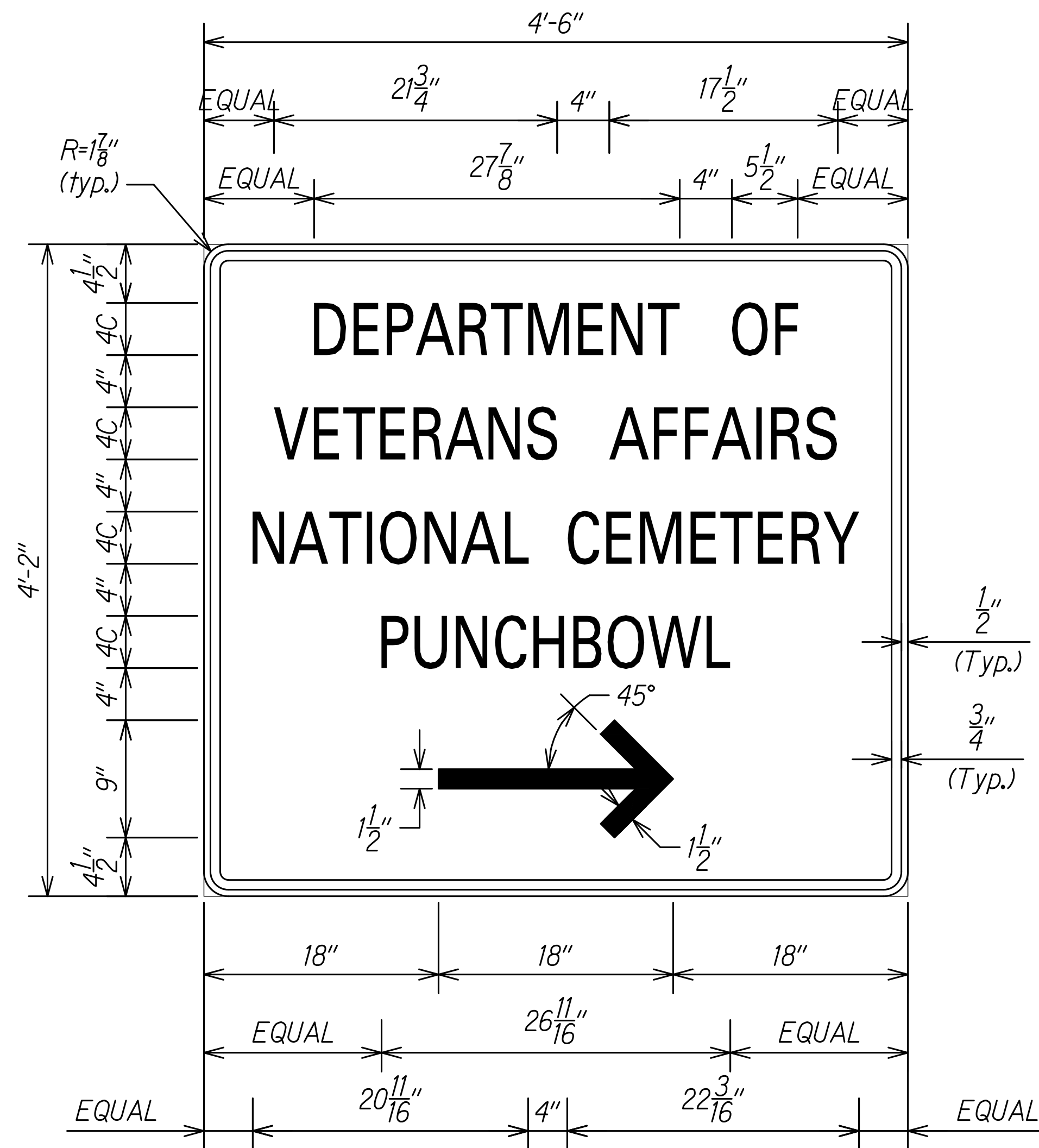
NATIONAL CEMETERY SIGN Not To Scale
