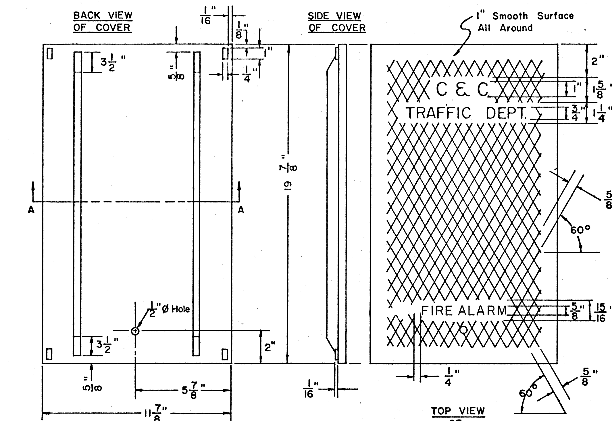
SECTION A-A N.T.S. NOTES 1. Sides of cover are slightly beveled to facilitate installation. Bevel is inward from front to back. 2. To be cast from grey iron.
