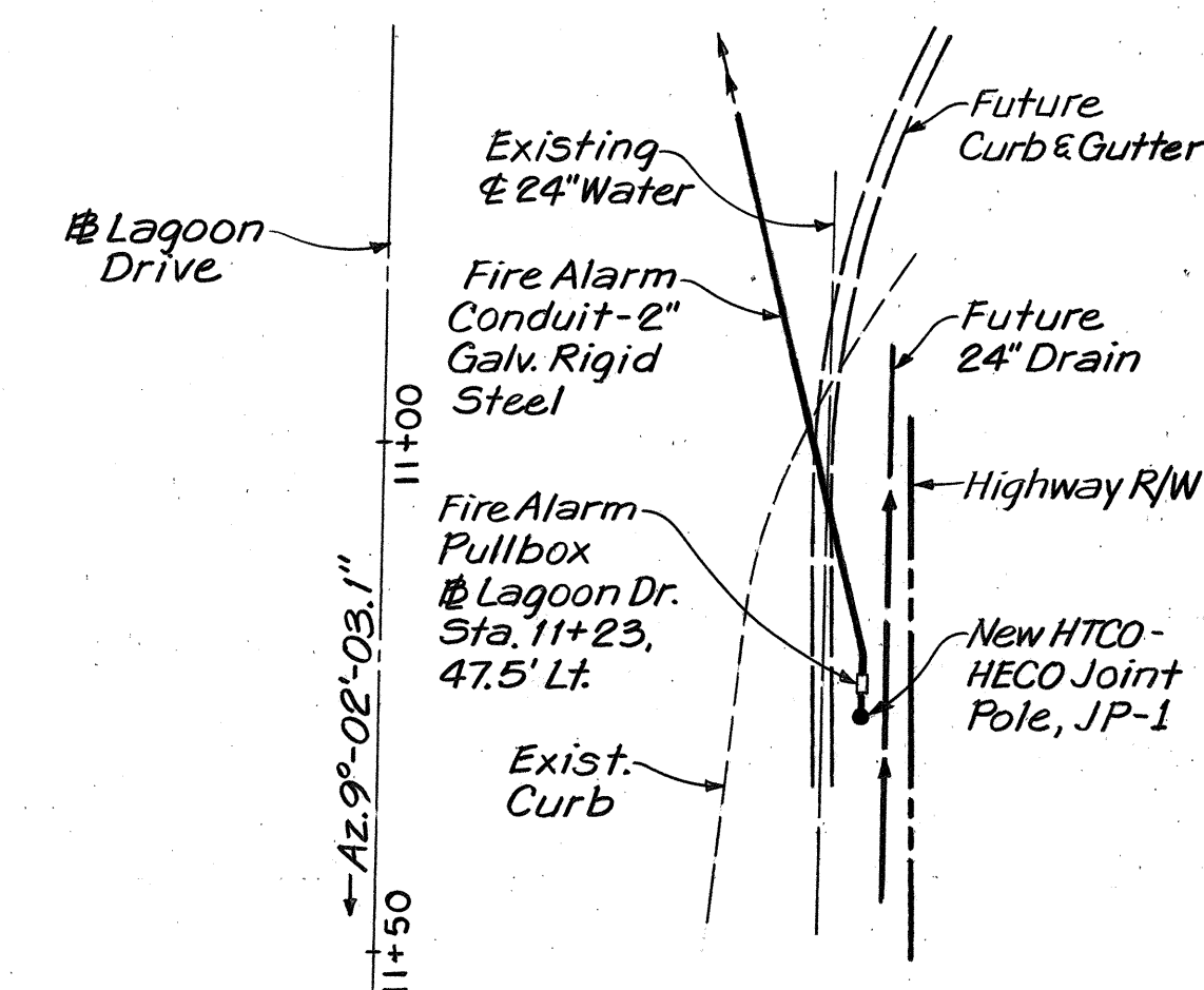
PLAN FIRE ALARM PULLBOX AT LAGOON DRIVE SCALE: 1"=20'
