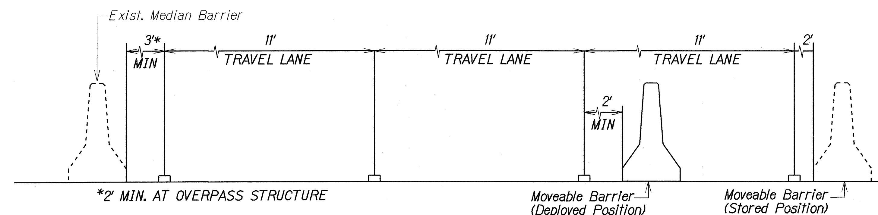
MOVEABLE BARRIER DEPLOYED POSITION DETAIL Not to Scale
