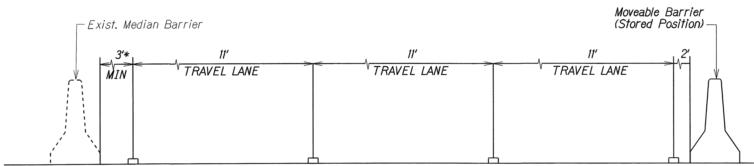
MOVEABLE BARRIER STORED POSITION DETAIL Not to Scale
