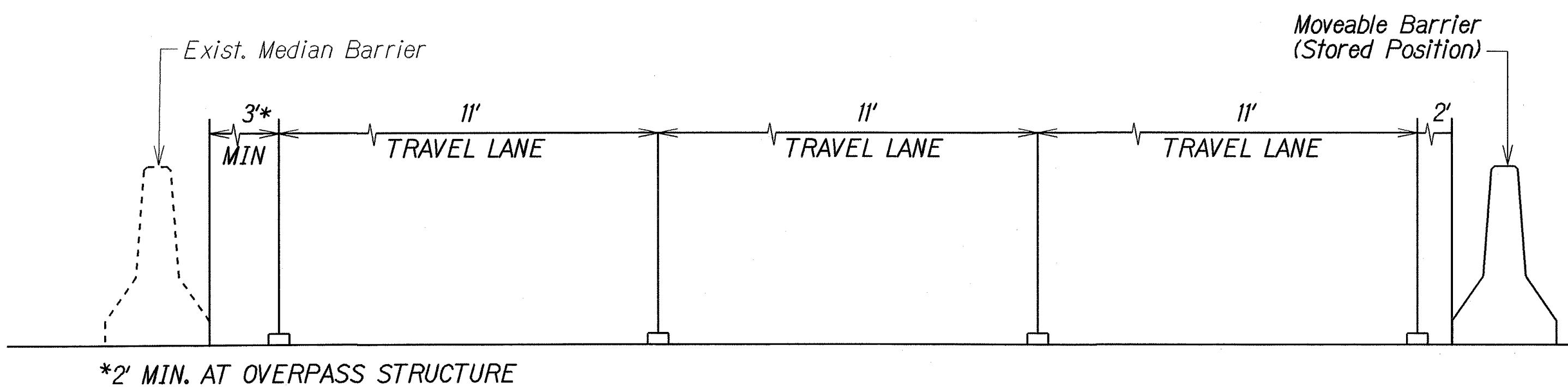
MOVEABLE BARRIER STORED POSITION DETAIL Not to Scale
