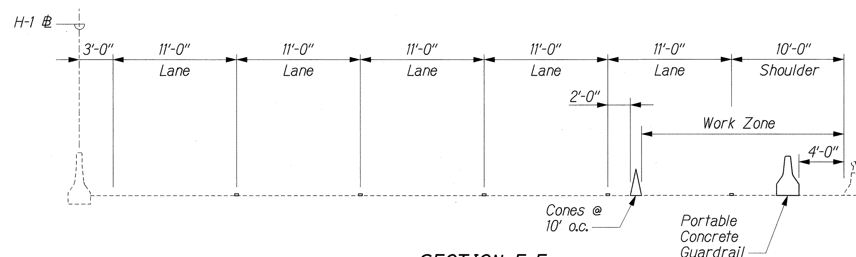
SECTION E-E Not to Scale
