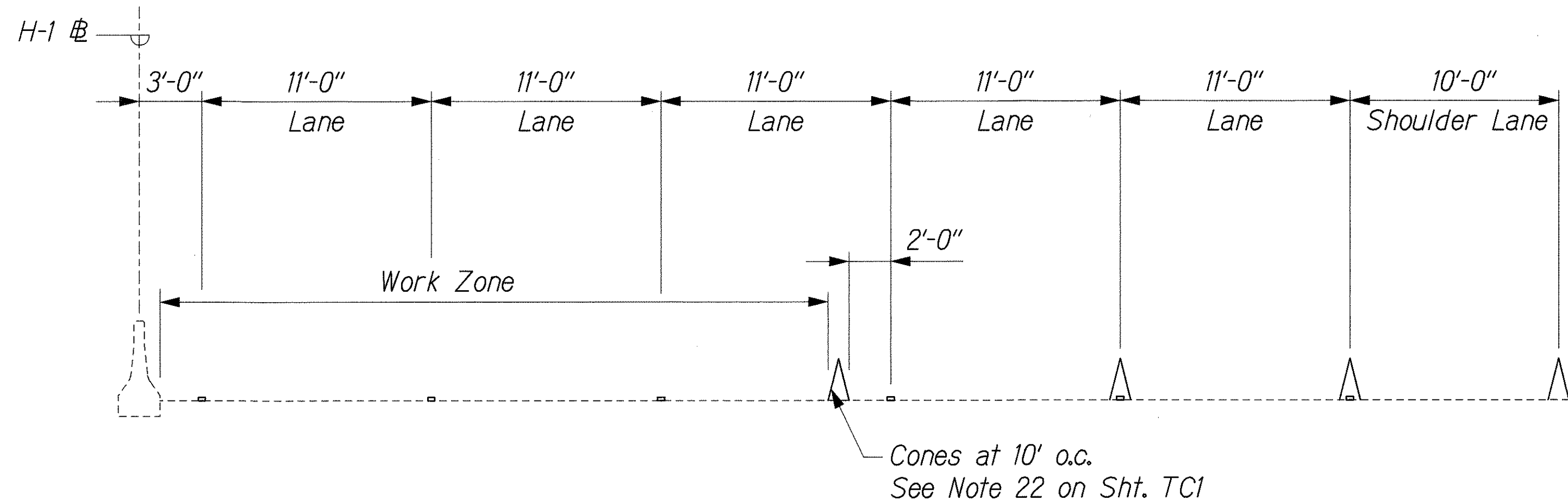
SECTION A-A Not to Scale
