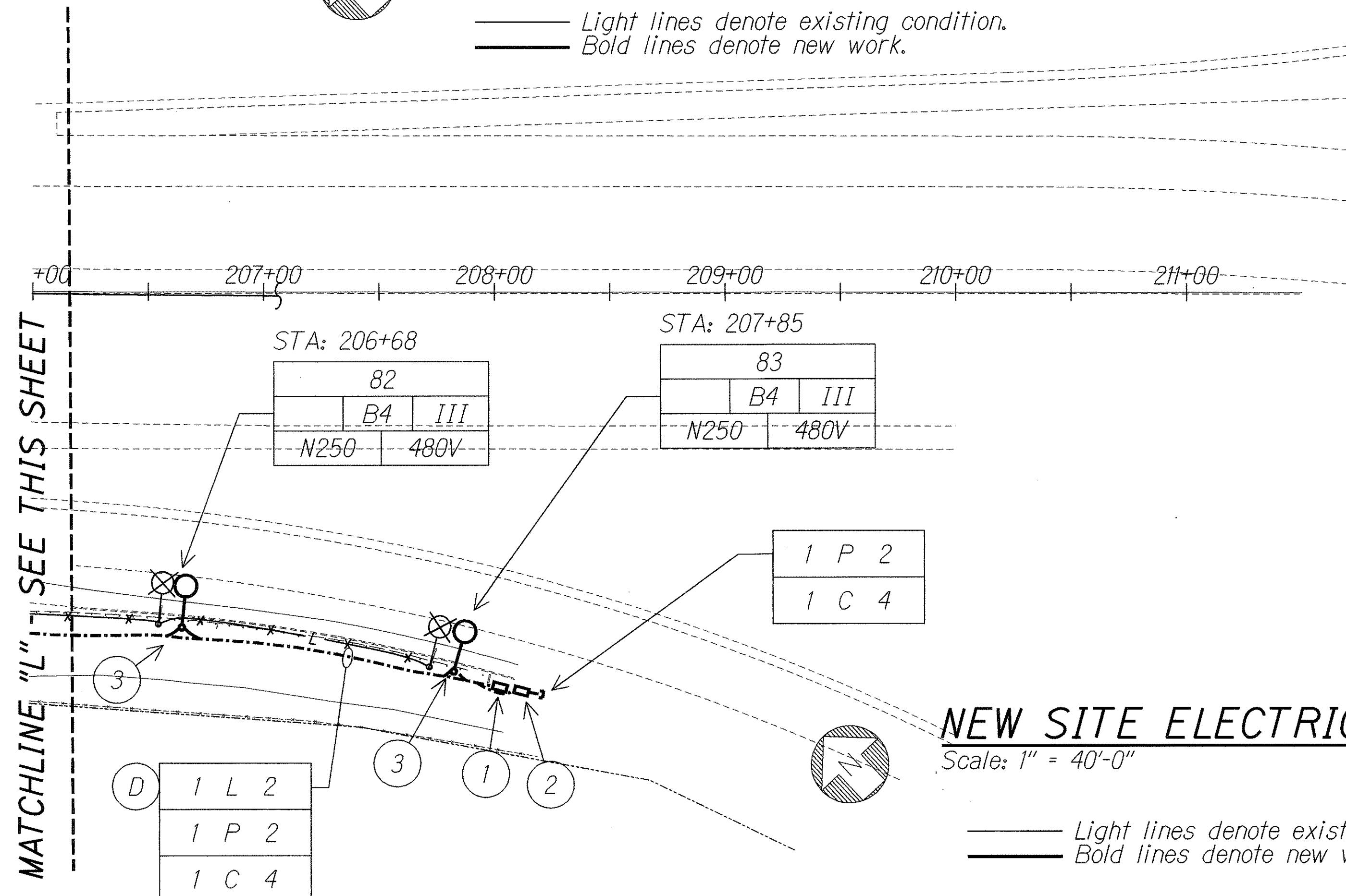
NEW SITE ELECTRICAL PLAN "L" Scale: 1" = 40'-0"
