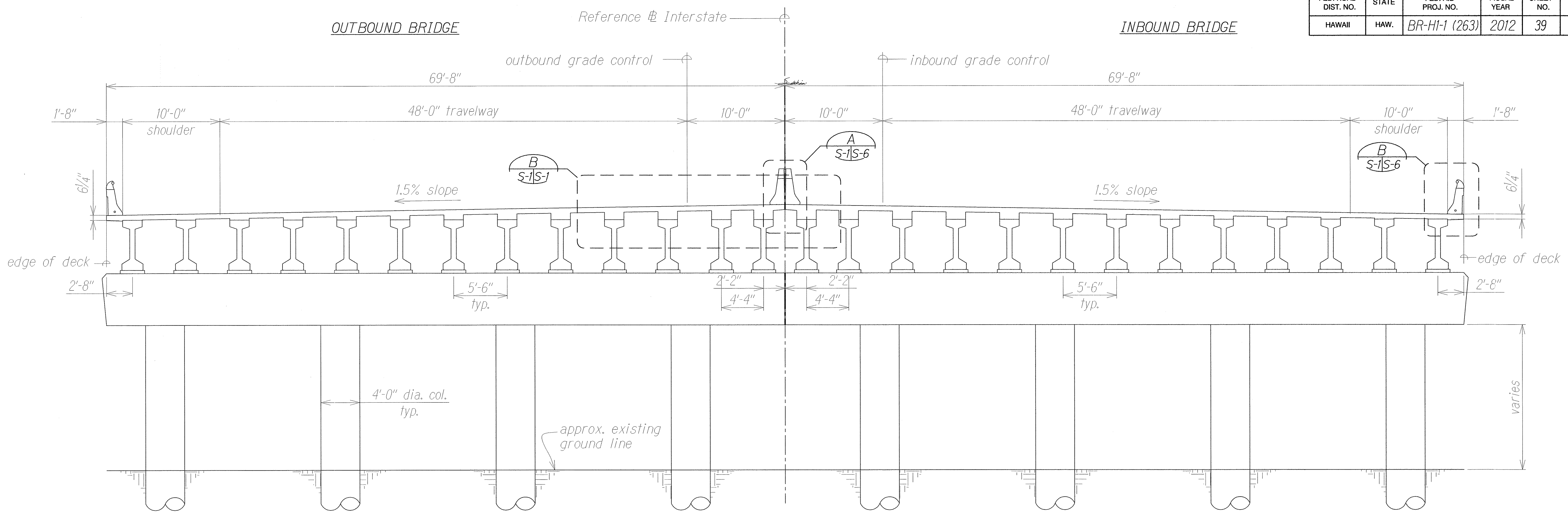
TRANSVERSE SECTION* AT PEARL CITY VIADUCT Scale: 3/16" = 1'-0" A S-1 S-1
