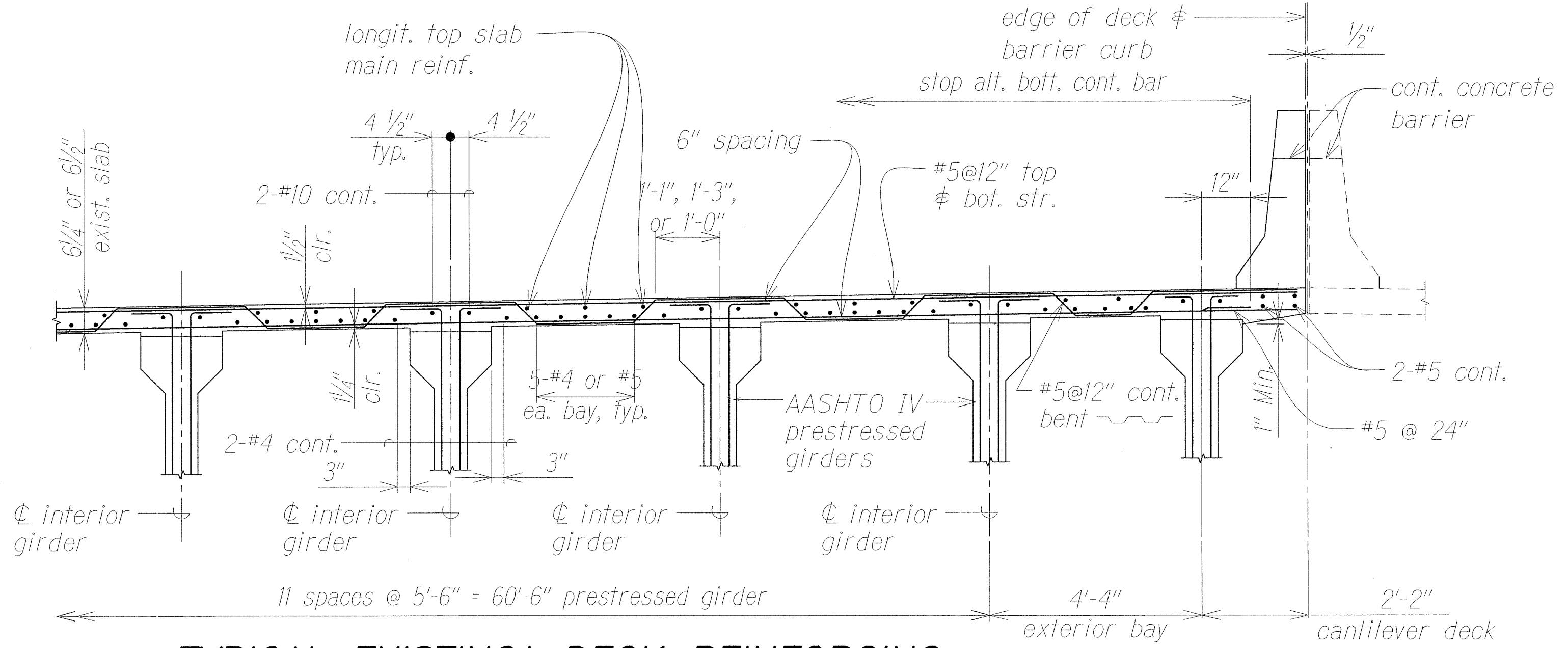
TYPICAL EXISTING* DECK REINFORCING (SECTION PERPENDICULAR TO TRAFFIC LANES) Scale: 1/2" = 1'-0" B S-1 S-1
