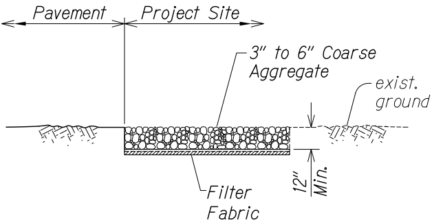
TEMPORARY STABILIZED CONSTRUCTION INGRESS/EGRESS Not to Scale
