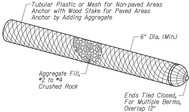
AGGREGATE FILTER POUCH Not to Scale
