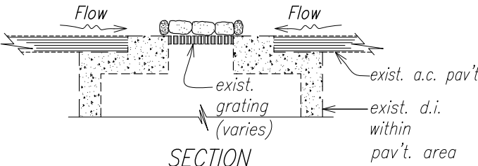
SAND OR GRAVEL BAGS AT GRATED DRAIN INLET Not to Scale
