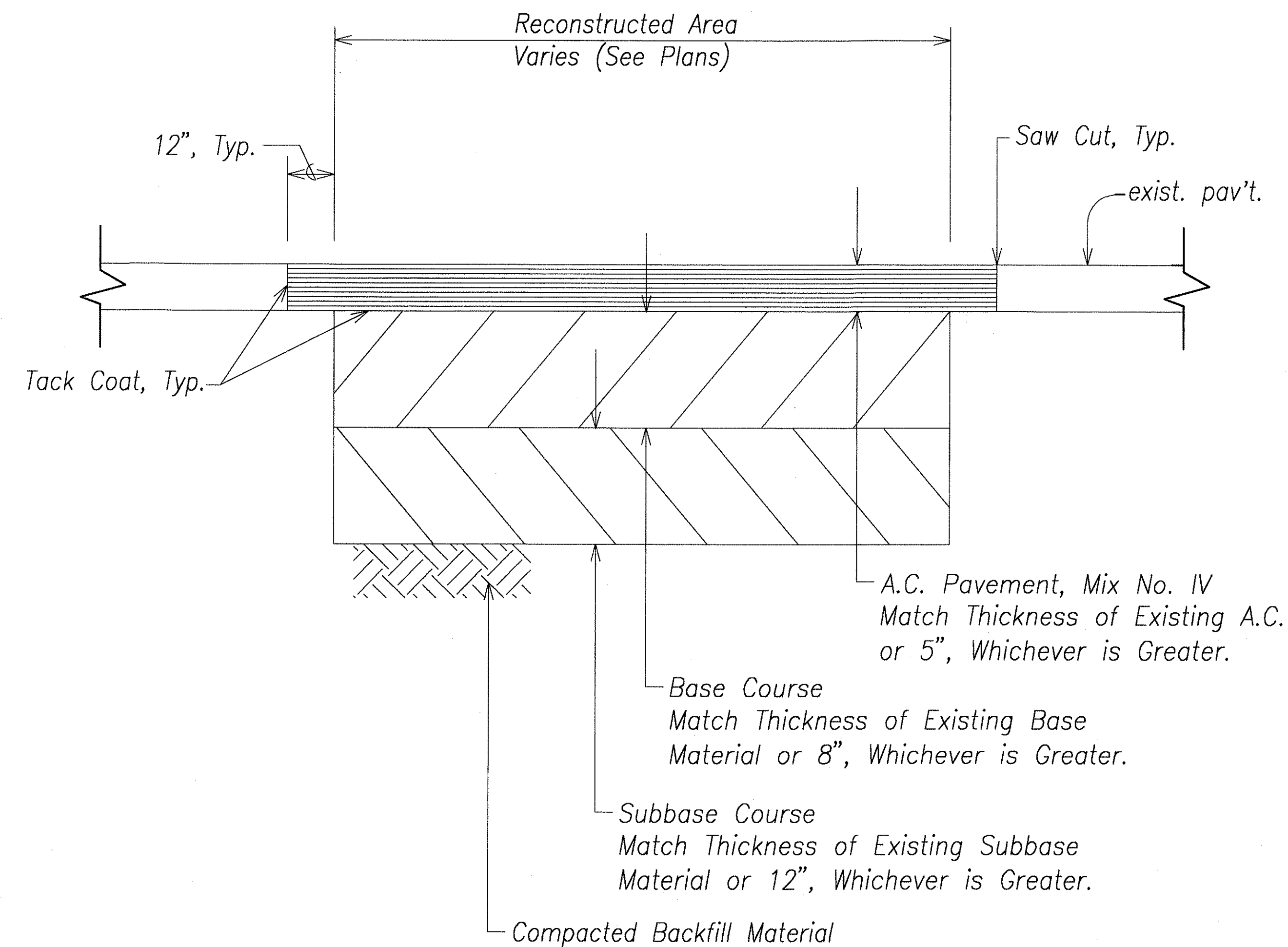
Typical Pavement Reconstruction Scale: Not To Scale
